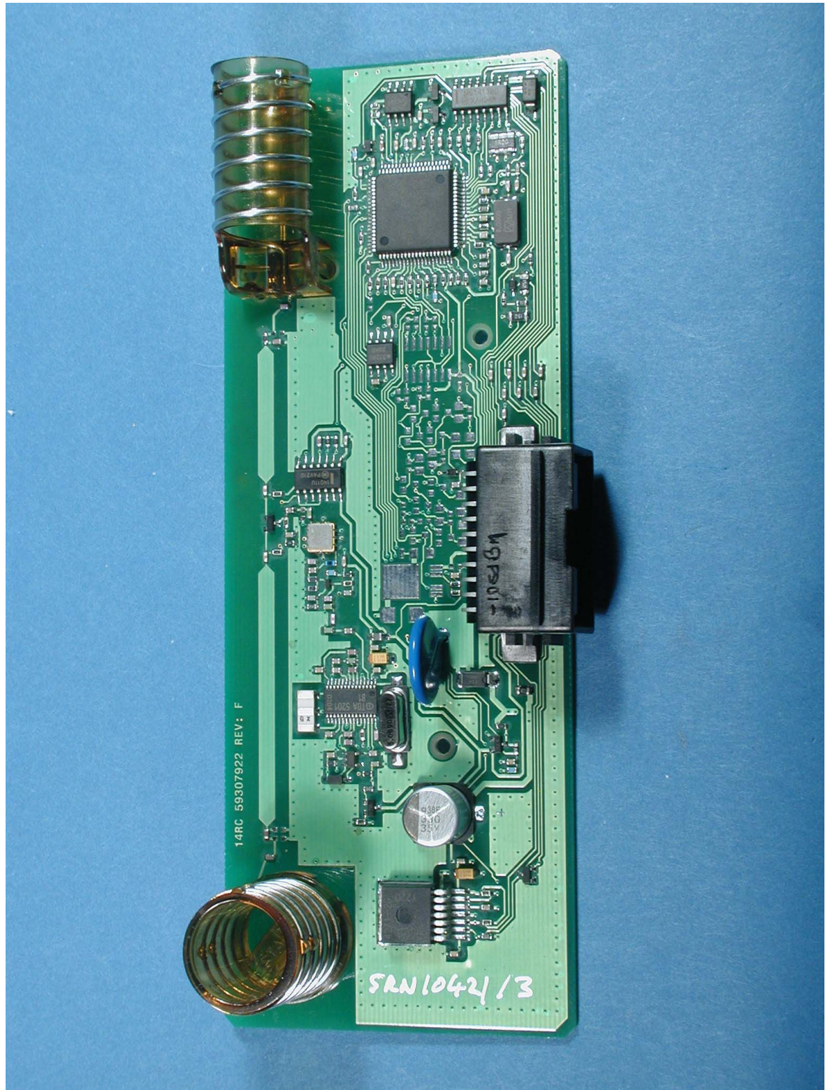
Photograph 7: Lowline receiver 14RC, PCB top view
