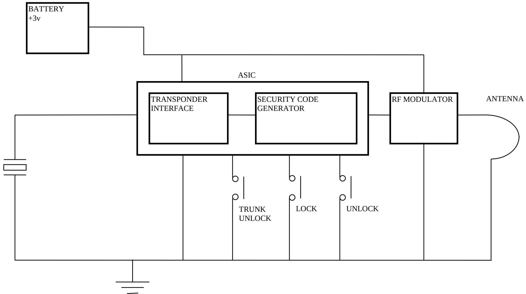
20TN-1 Block Diagram
