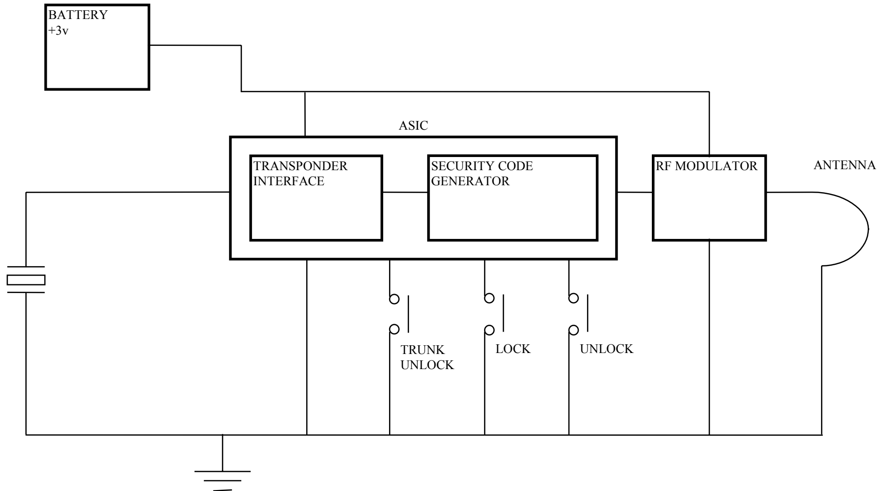
20TN Block Diagram
