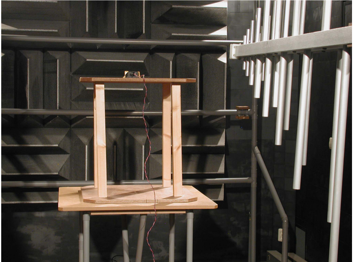
Photograph 6: Test set up ( > 30 MHz)
