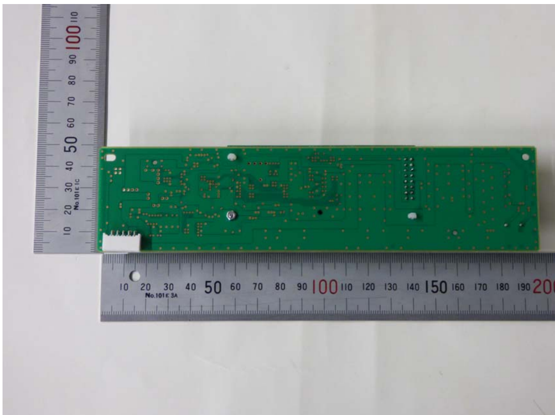
[LCD panel board, bottom side]
