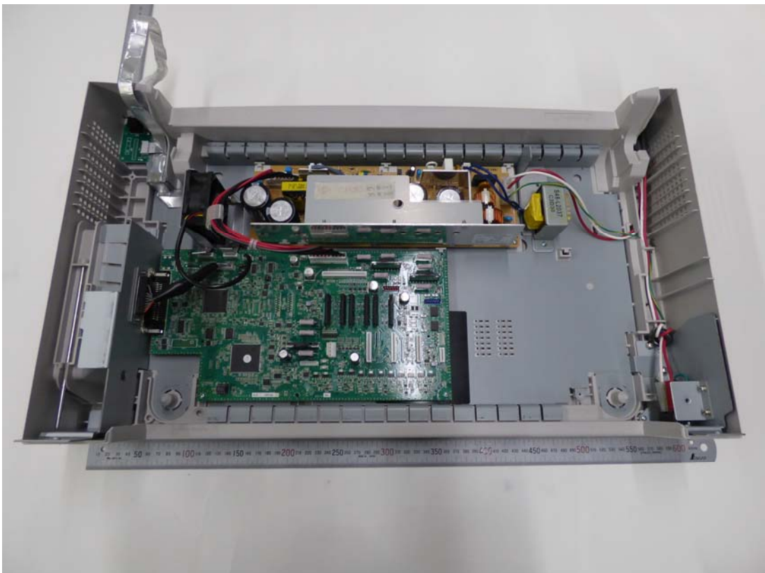
[Main board (Serial) and Power supply board]
