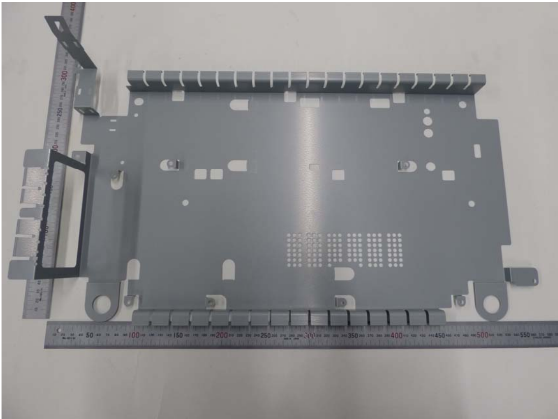
[EUT bottom, sheet metal]
