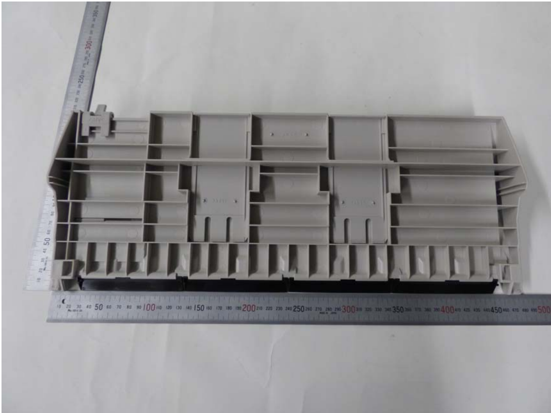
[Paper Receiver of EUT, back side]
