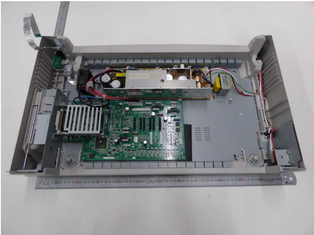
[Main board (USB) and Power supply board]
