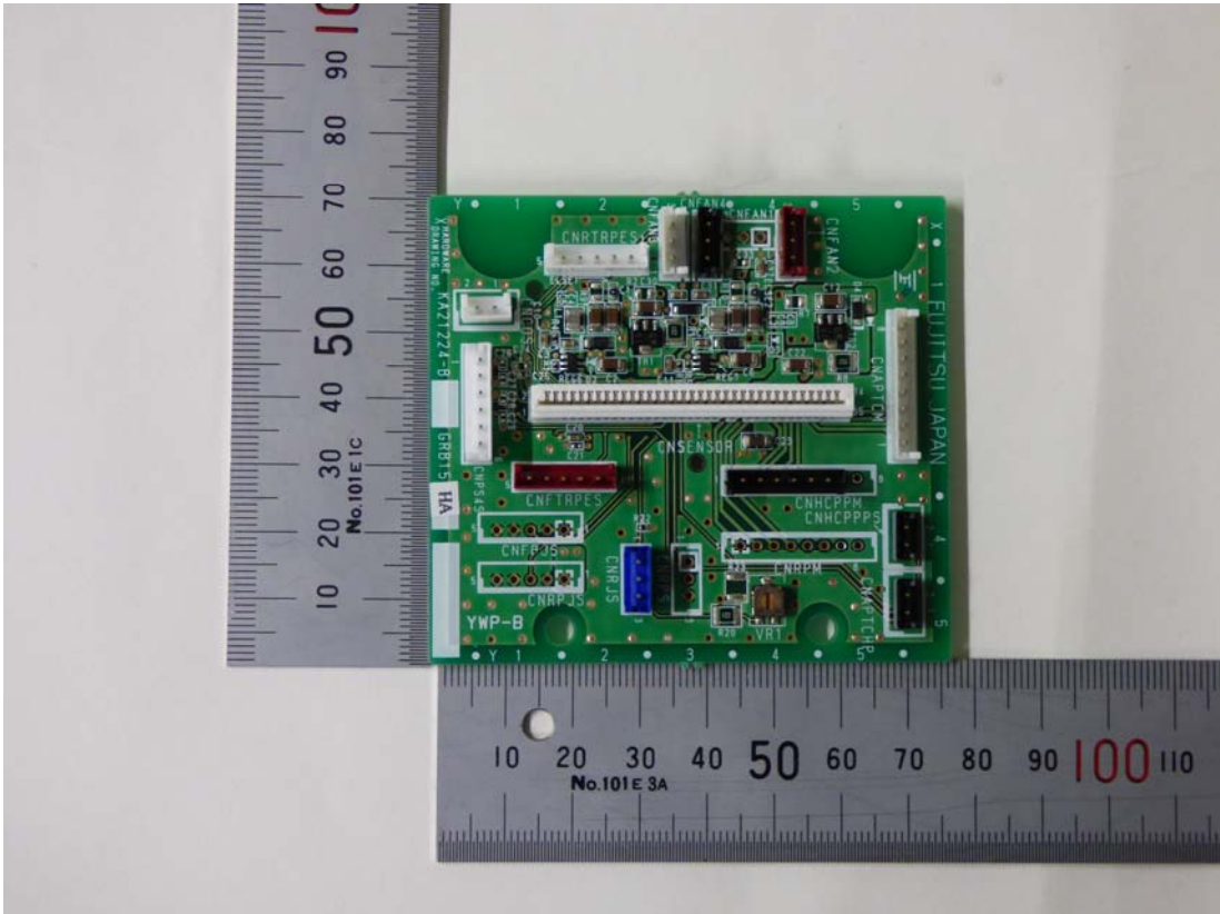
[Relay board, top side]
