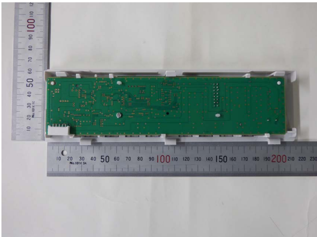
[LCD panel set, bottom side]
