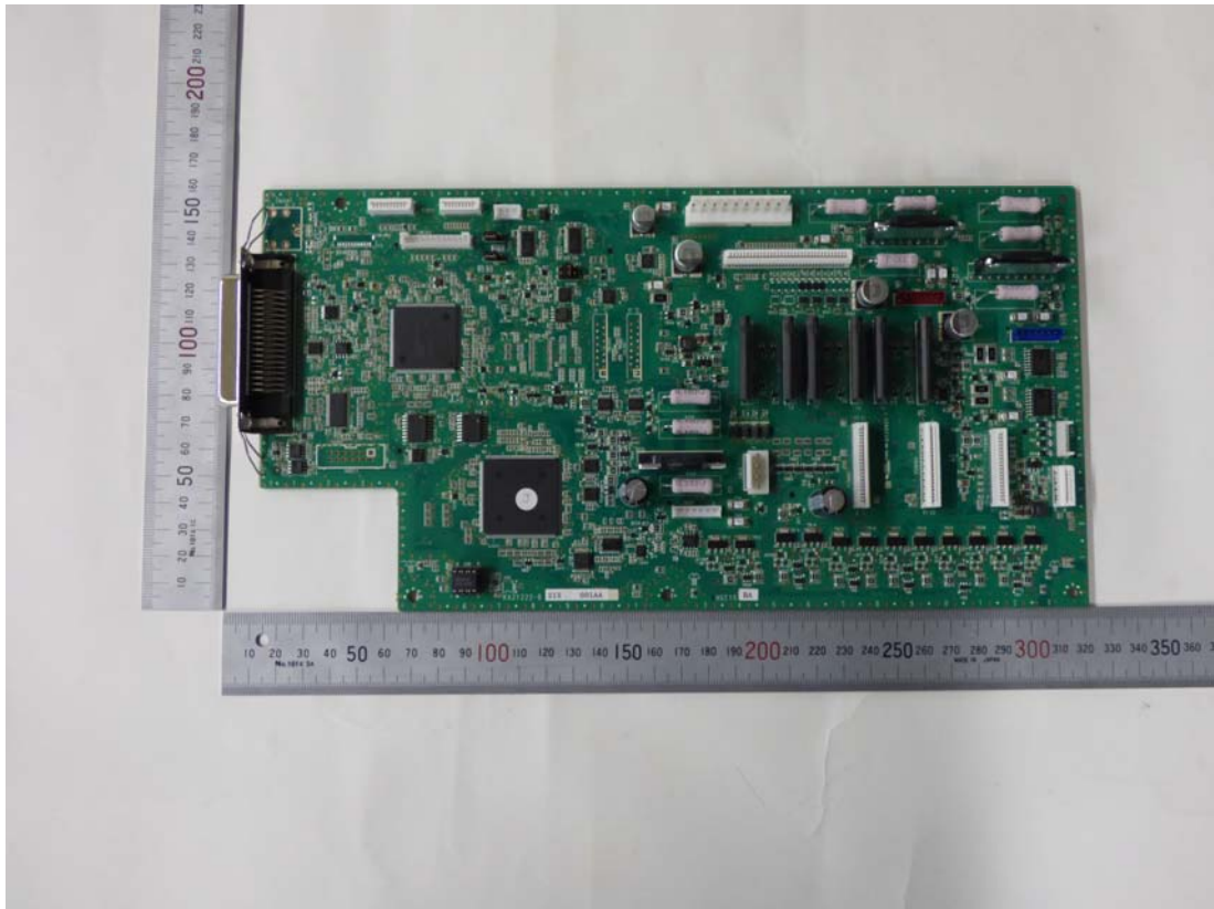
[Main board (Serial), top side]
