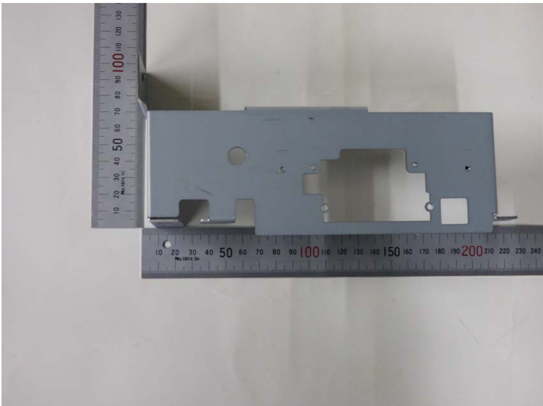
[USB I/F sheet metal, outside]
