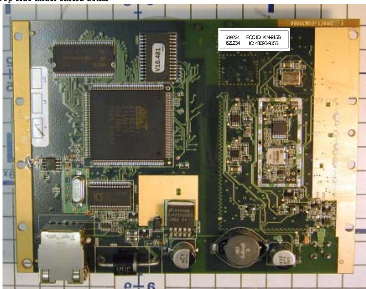
Top side under shield detail
