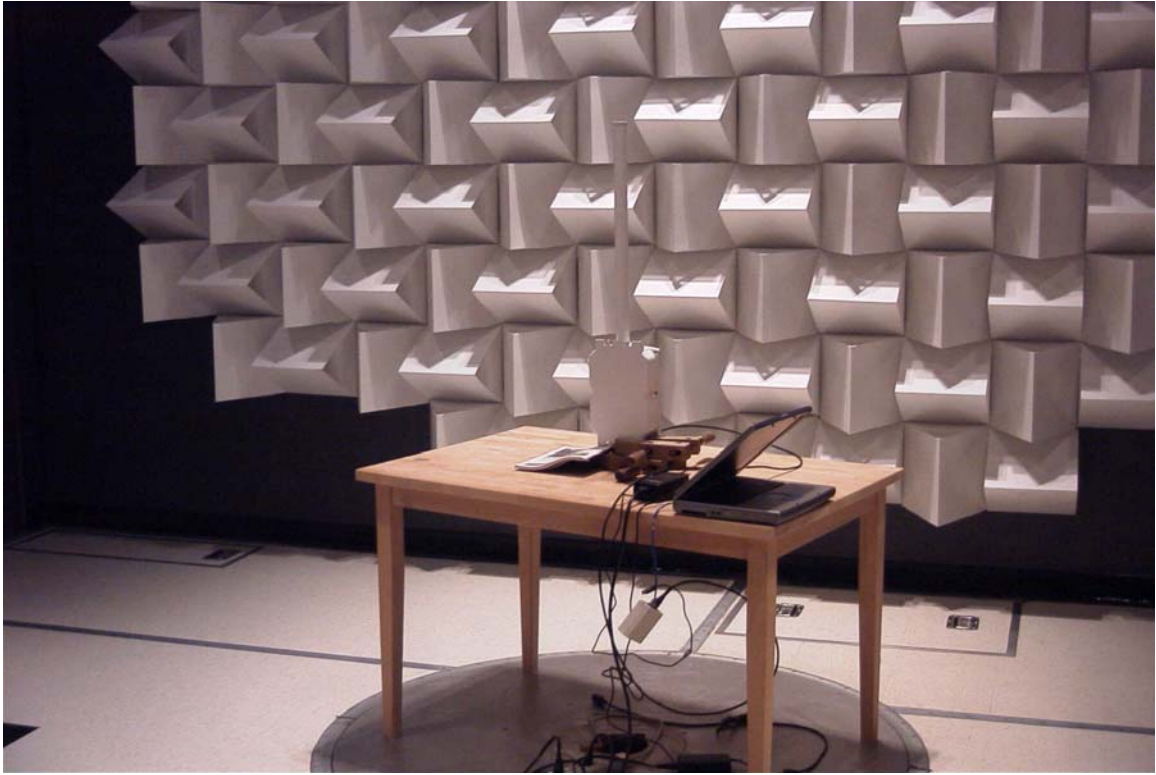
RADIATED TEST SET UP PHOTO
