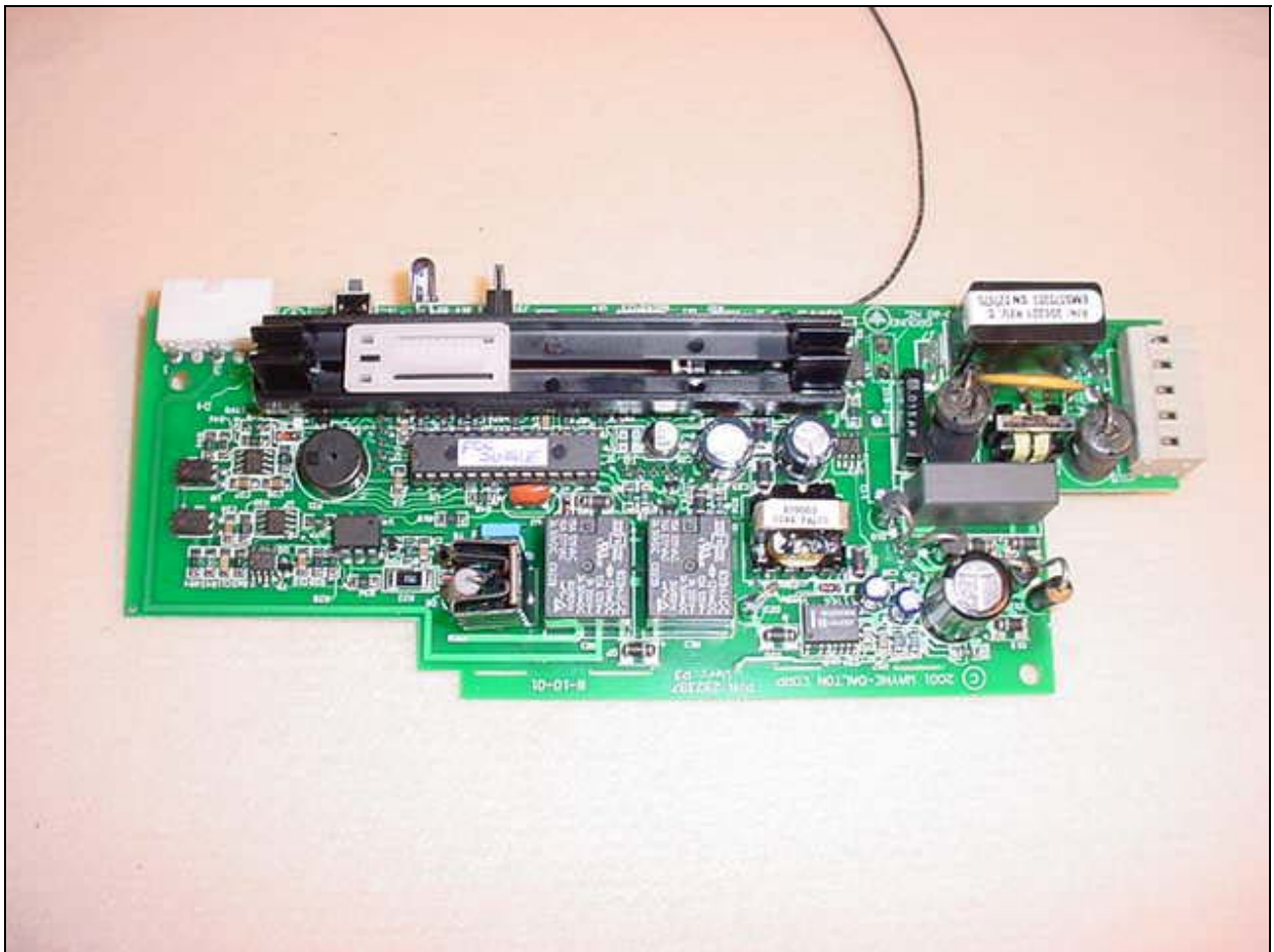
Figure 1: Internal Main Board– Top View
