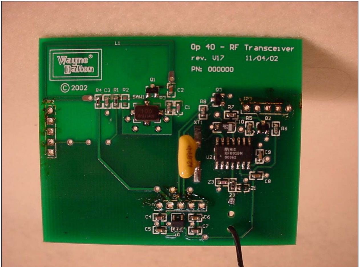
Figure 3: Transceiver Board – Top View
