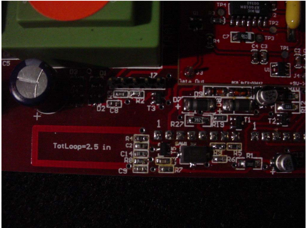
Figure 7: Transmitter Circuitry
