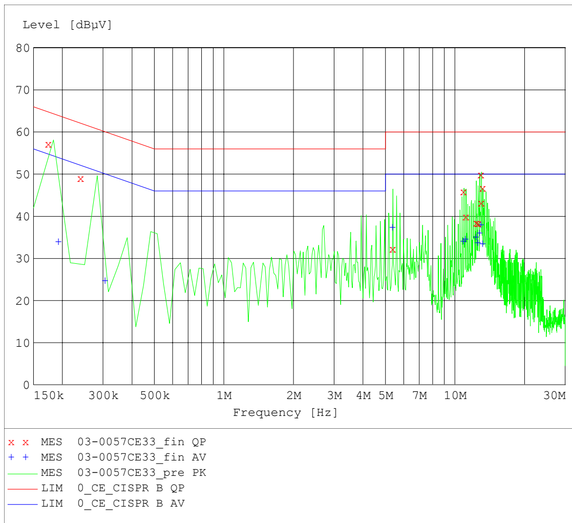
Figure 6.2.1-2: Conducted Emissions Graph – Line
