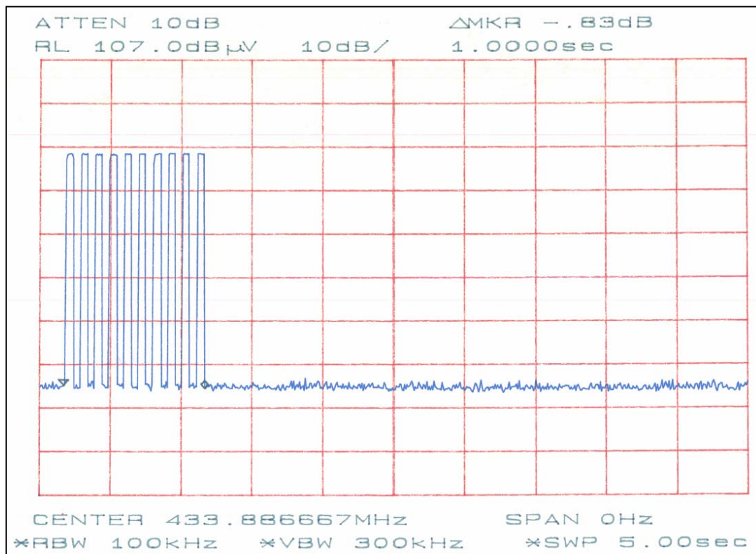
Figure 6.3.3-1: Transmission Duration Timing Diagram
