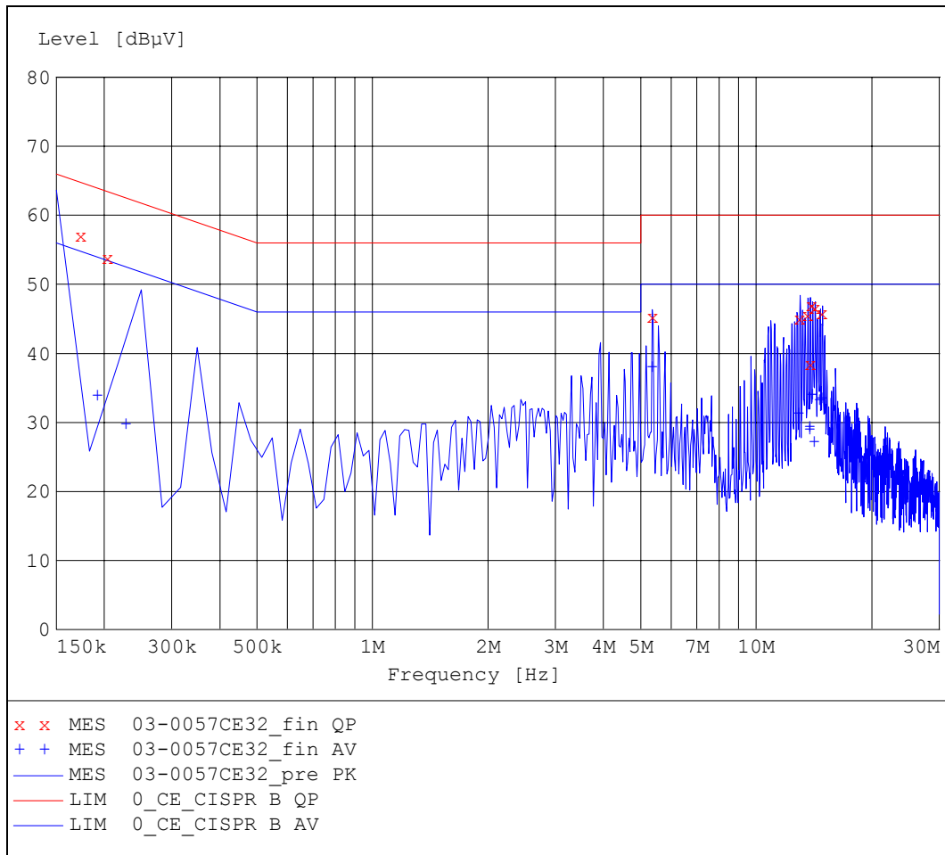
Figure 6.2.1-1: Conducted Emissions Graph – Neutral Line
