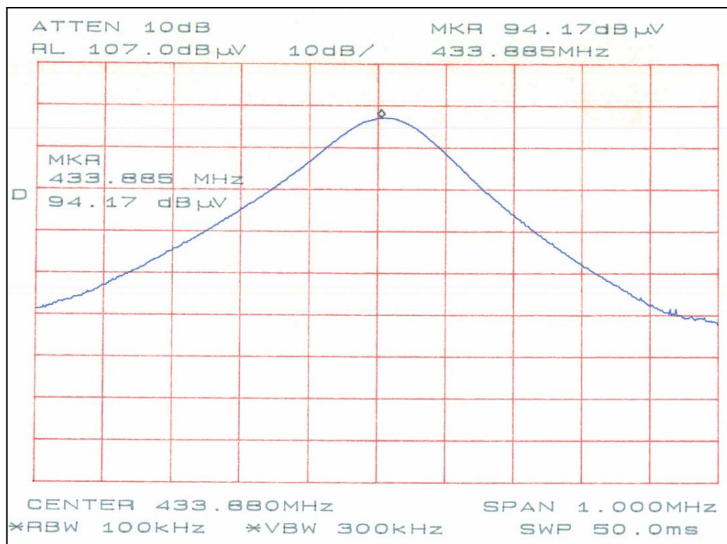
Figure 6.4.3.2-1: Fundamental Field Strength
