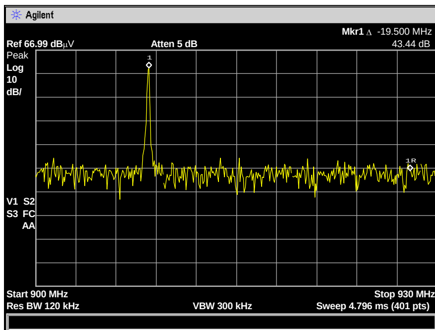
Figure 7.5.3-1 Band Edge Plot
