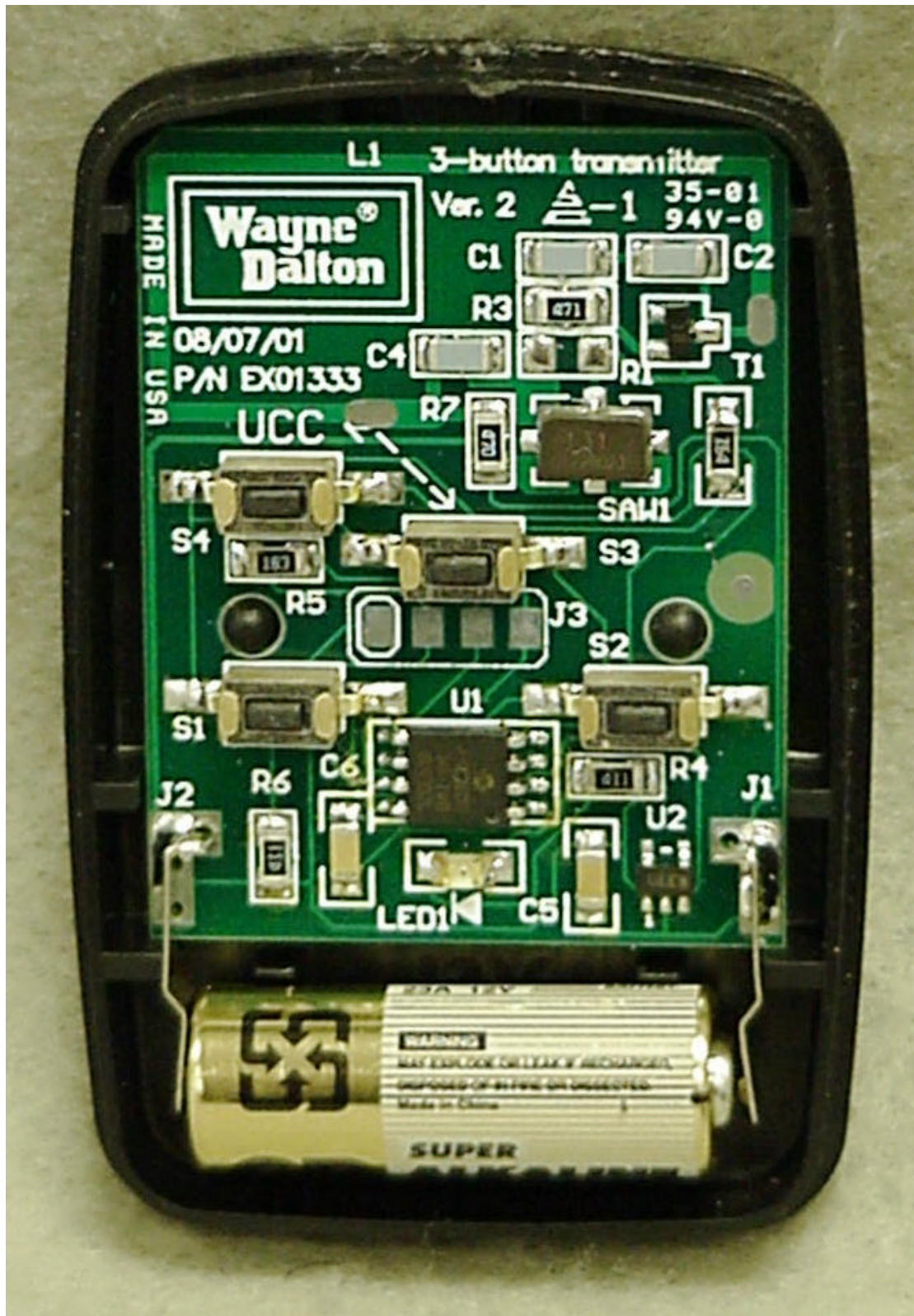
Photo 3. Internal View, Top Side
