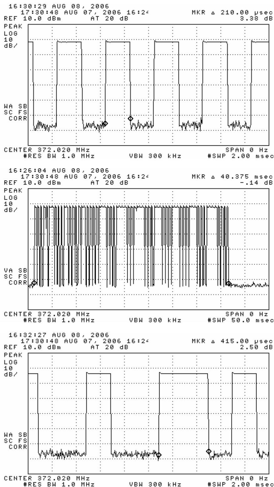
Figure 6.1(b). Transmissions modulation characteristics: (top) expanded wakeup, (center) expanded PWM data, (bottom) expanded PWM bit.
