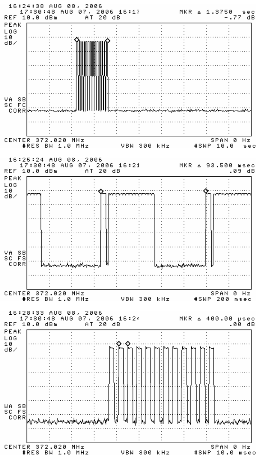
Figure 6.1(a). Transmissions modulation characteristics: (top) single button press, (center) expanded word, (bottom) expanded wake-up.
