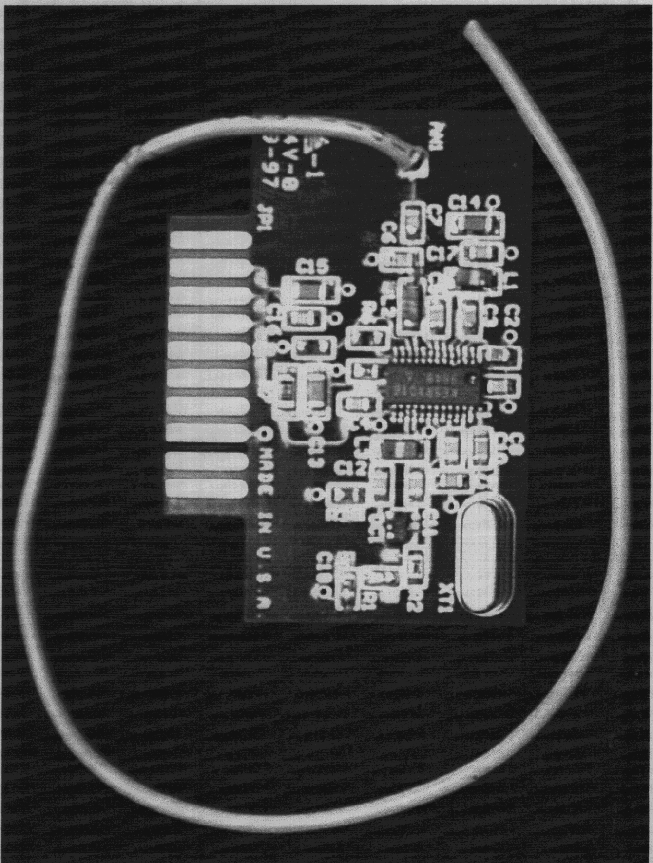
Photo 5. Receiver Board, Component Side
