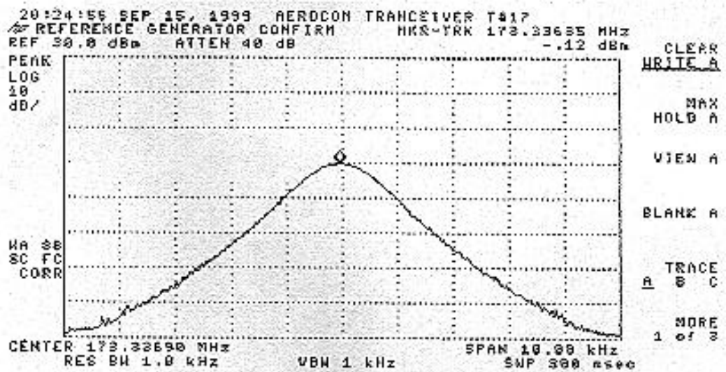
Transmitter Output and Signal Generator Confirmation @ 50 °C
