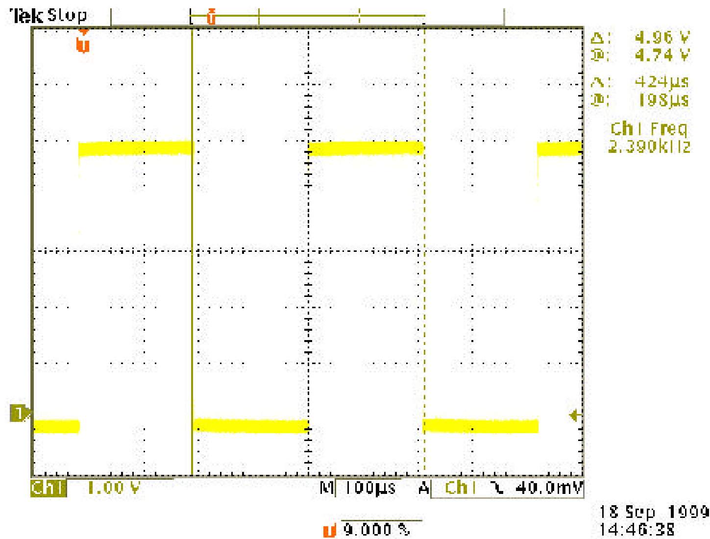
Waveform of the Modulation Input Signal to the Transmitter
