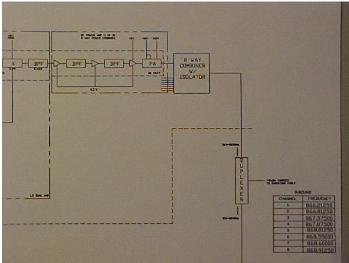
Figure 4: Block Diagram 4 of 7
