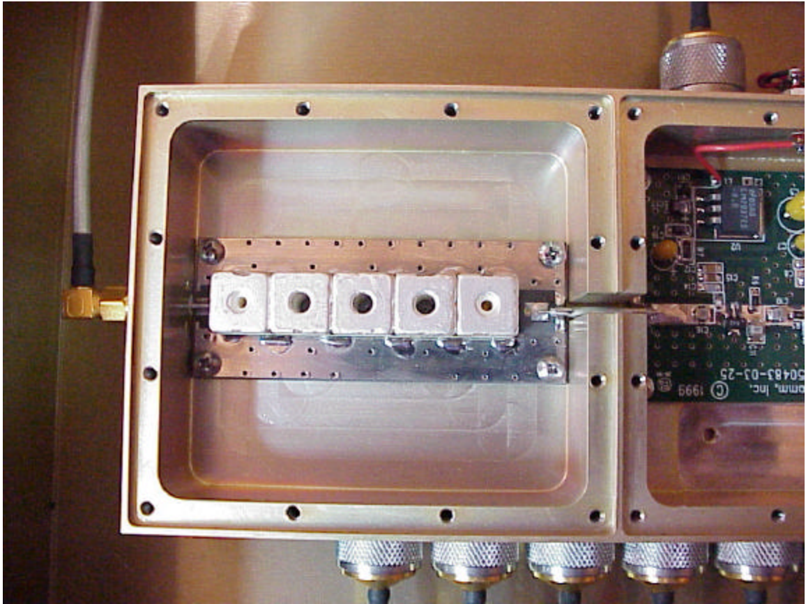
Figure 10: LNA Picture 2 of 3: Component Side
