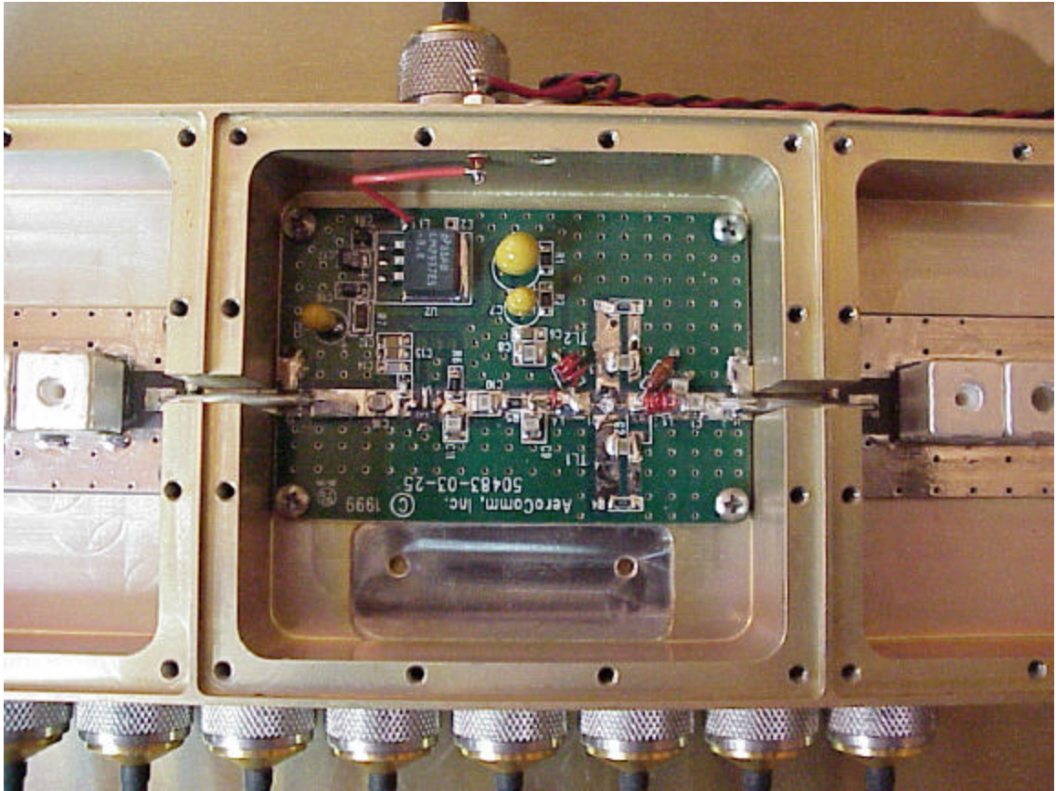
Figure 9:LNA picture 1 of 3: Component side
