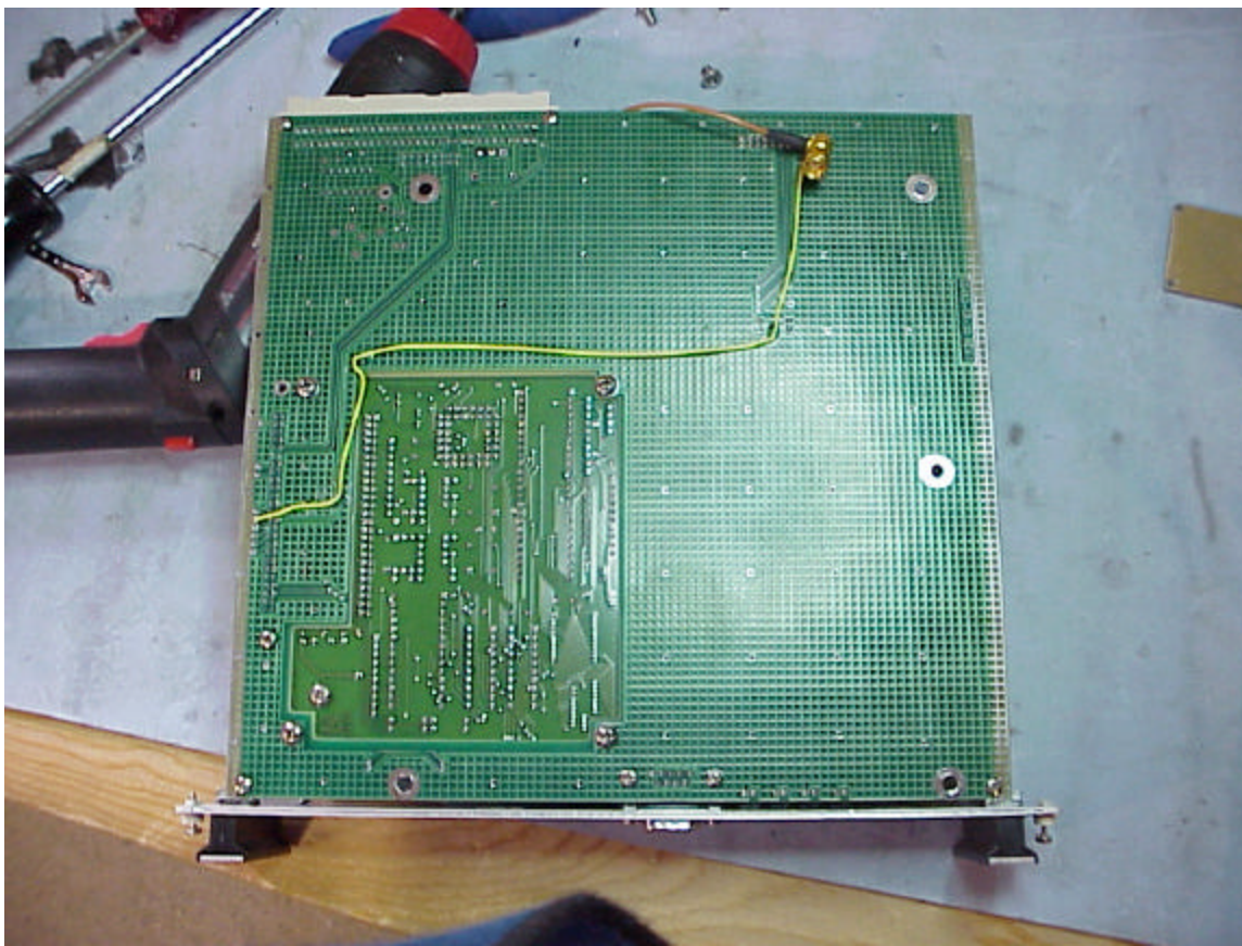
Figure 8:PLL OSC Board Trace side
