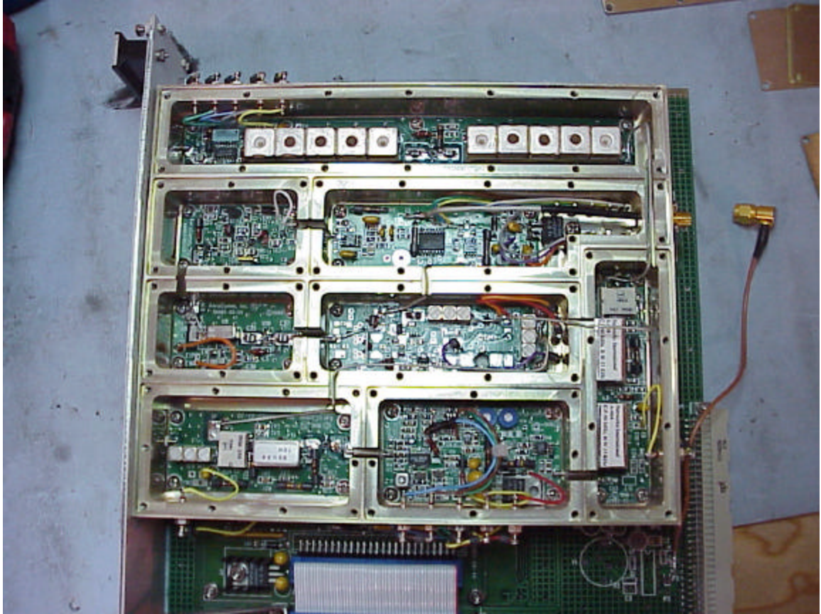
Figure 5: PLL module component side
