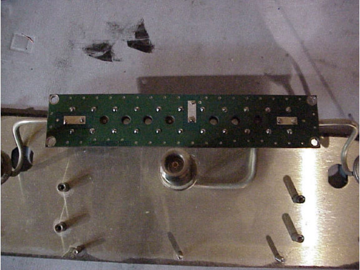
Figure 15: Duplexer trace side
