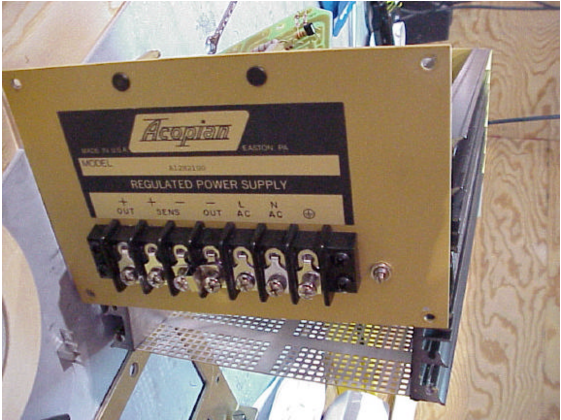
Figure 2: Power Supply back Panel
