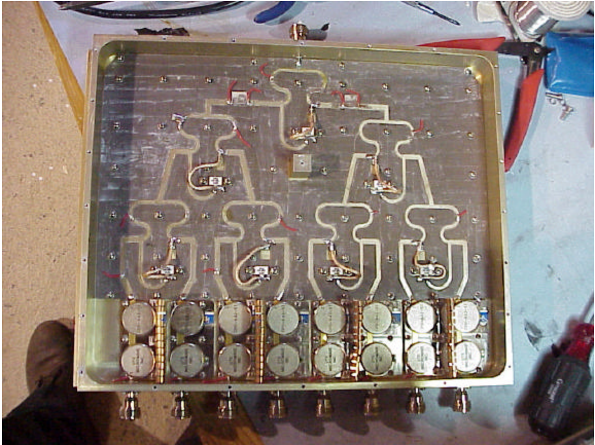
Figure 13: Amp Combiner; Trace side
