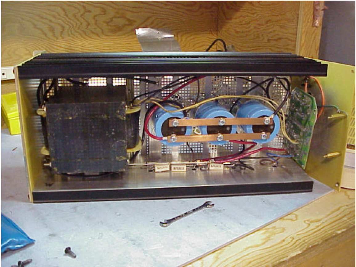
Figure 1: Power Supply
