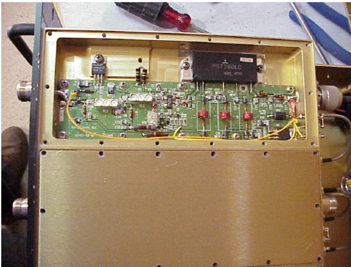
Figure 12: Amp combiner component side
