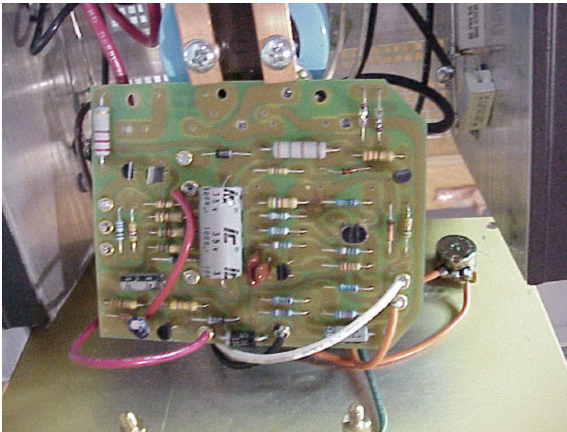
Figure 4: Power supply: Component Side of PCB
