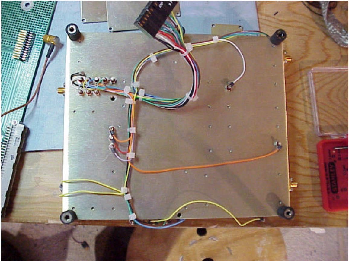
Figure 6: PLL module back side
