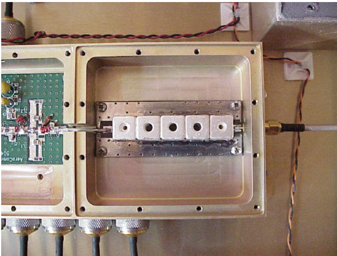
Figure 11: LNA Picture 3 of 3 : component side
