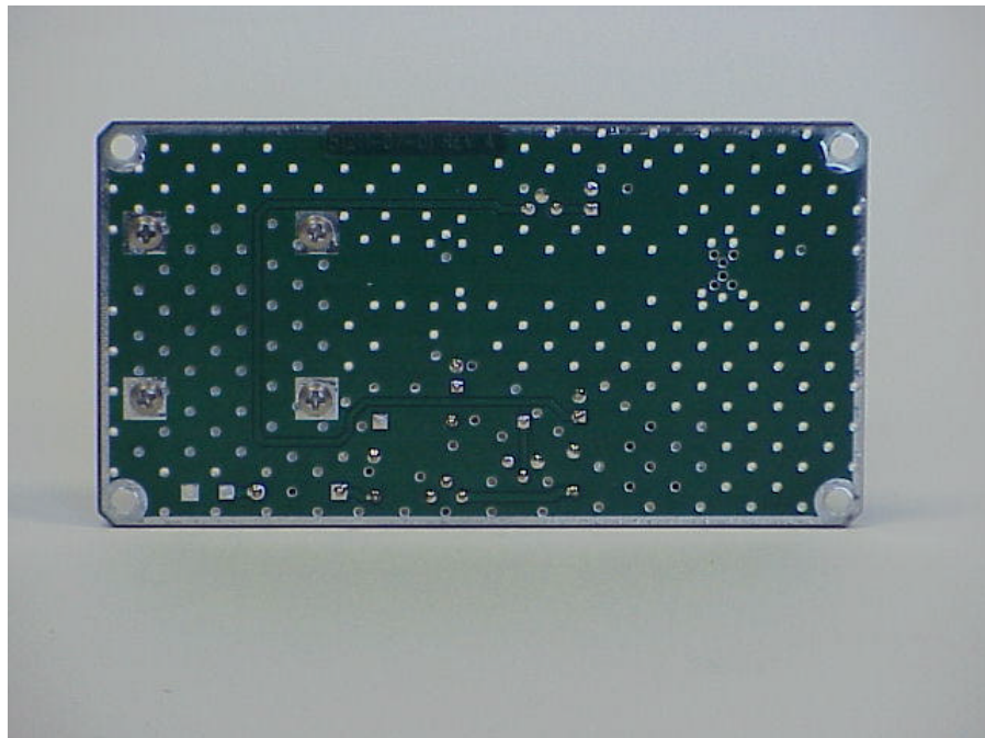
PHOTOGRAPH OF LNA Module Soldering Side Model: 51211CELL, S/N 0101-99
