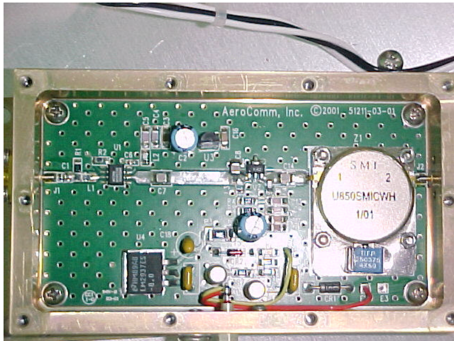
PHOTOGRAPH OF LNA Module Component Side Model: 51211CELL, S/N 0101-99
