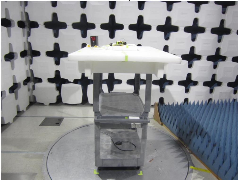
Radiated Spurious
