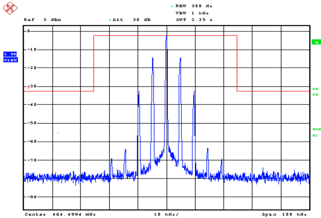
Low Channel, 464.5 MHz, fC ± 50 kHz
