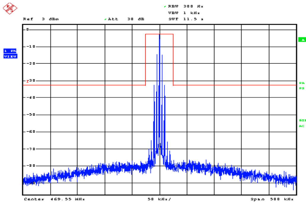
High Channel, 469.55 MHz, f_c \pm 250 kHz
