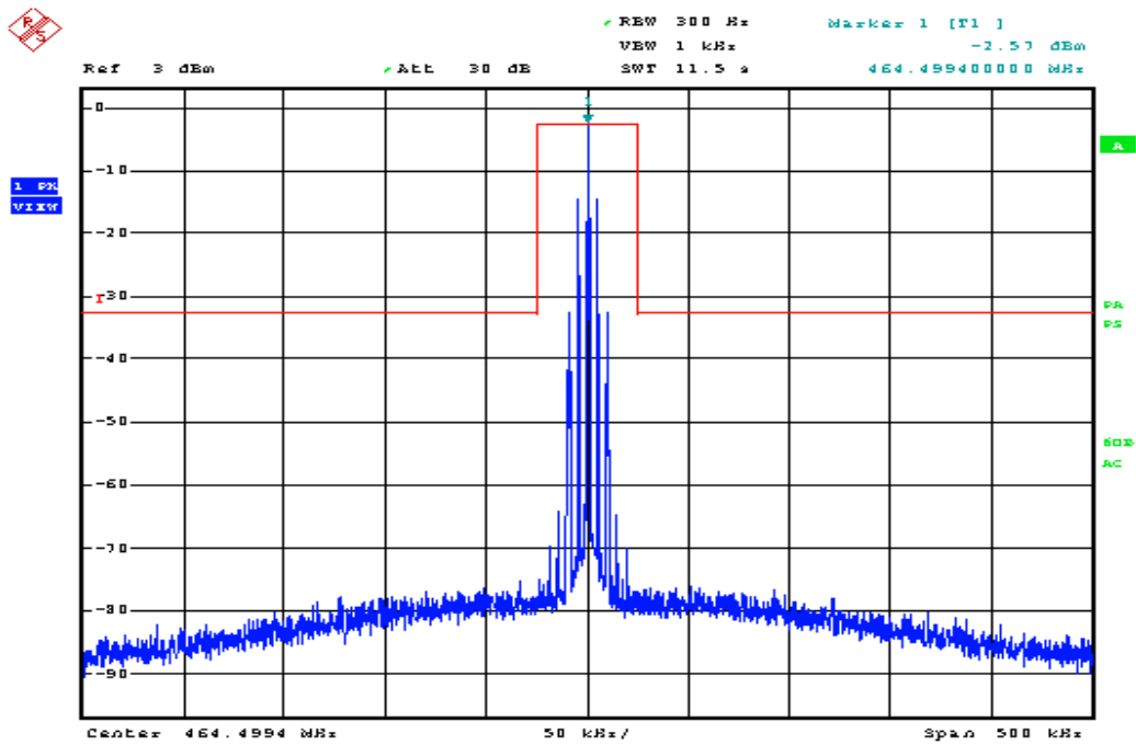
Low Channel, 464.5 MHz, fC ± 250 kHz
