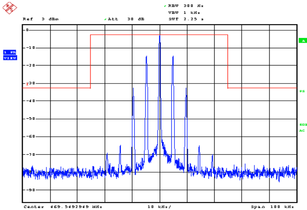
High Channel, 469.55 MHz, f_c \pm 50 kHz
