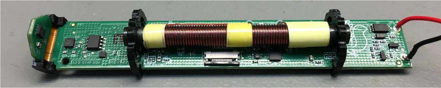
Top Side, Antenna removed
