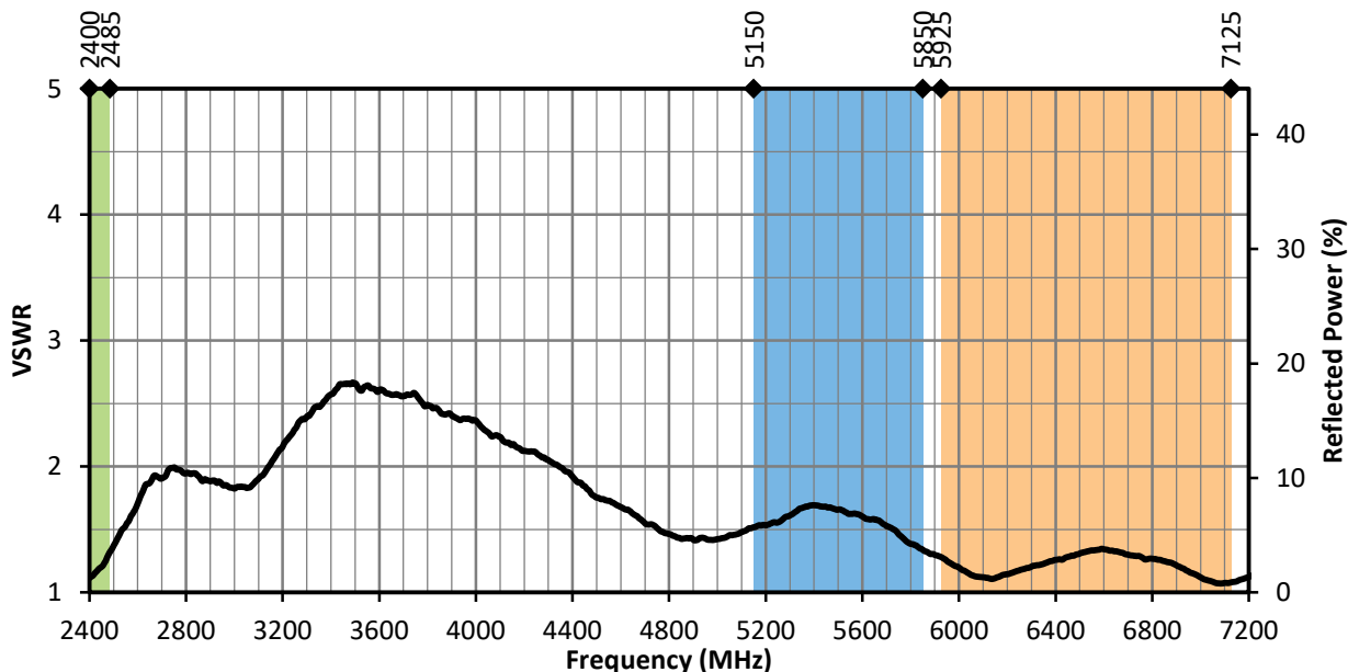
Figure 11. ANT-W63WS2-ccc VSWR, Edge-Bent
