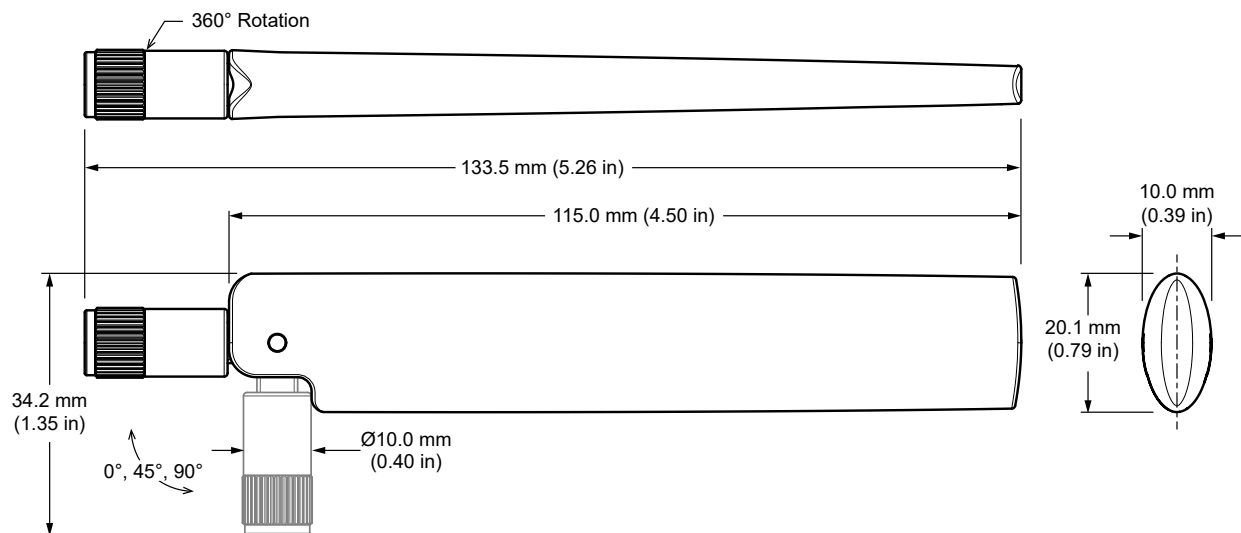
Figure 1. ANT-W63WS2-ccc Antenna Dimensions
