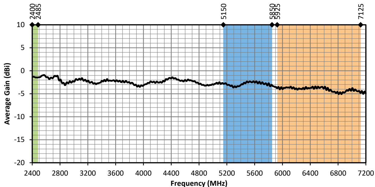
Figure 14. ANT-W63WS2-ccc Antenna Average Gain, Edge-Bent
