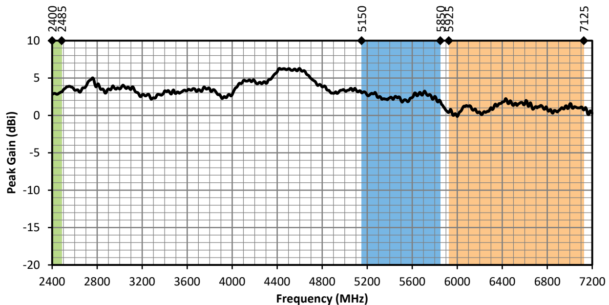
Figure 13. ANT-W63WS2-ccc Peak Gain, Edge-Bent
