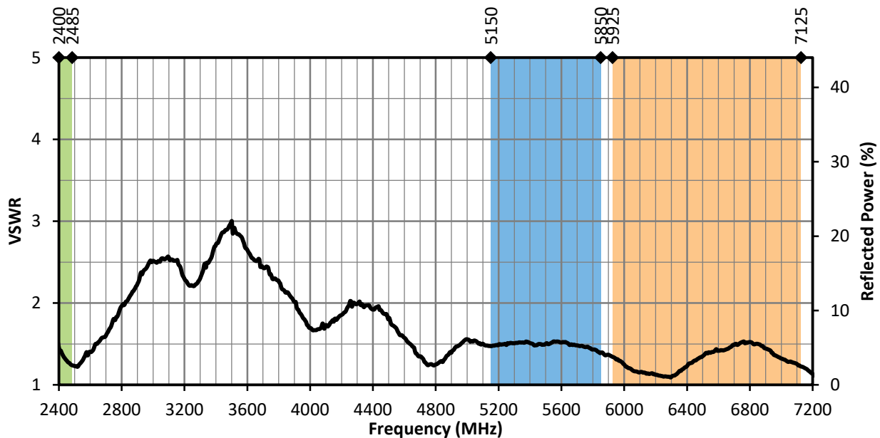
Figure 4. ANT-W63WS2-ccc VSWR, Straight
