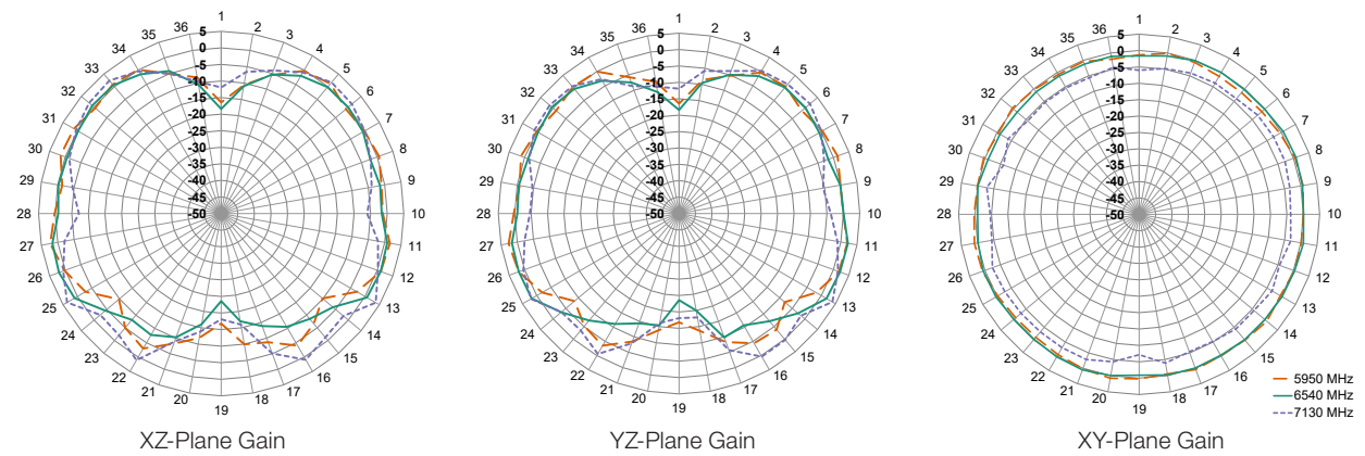
Figure 9. Radiation Patterns for ANT-W63WS2-ccc, Straight
