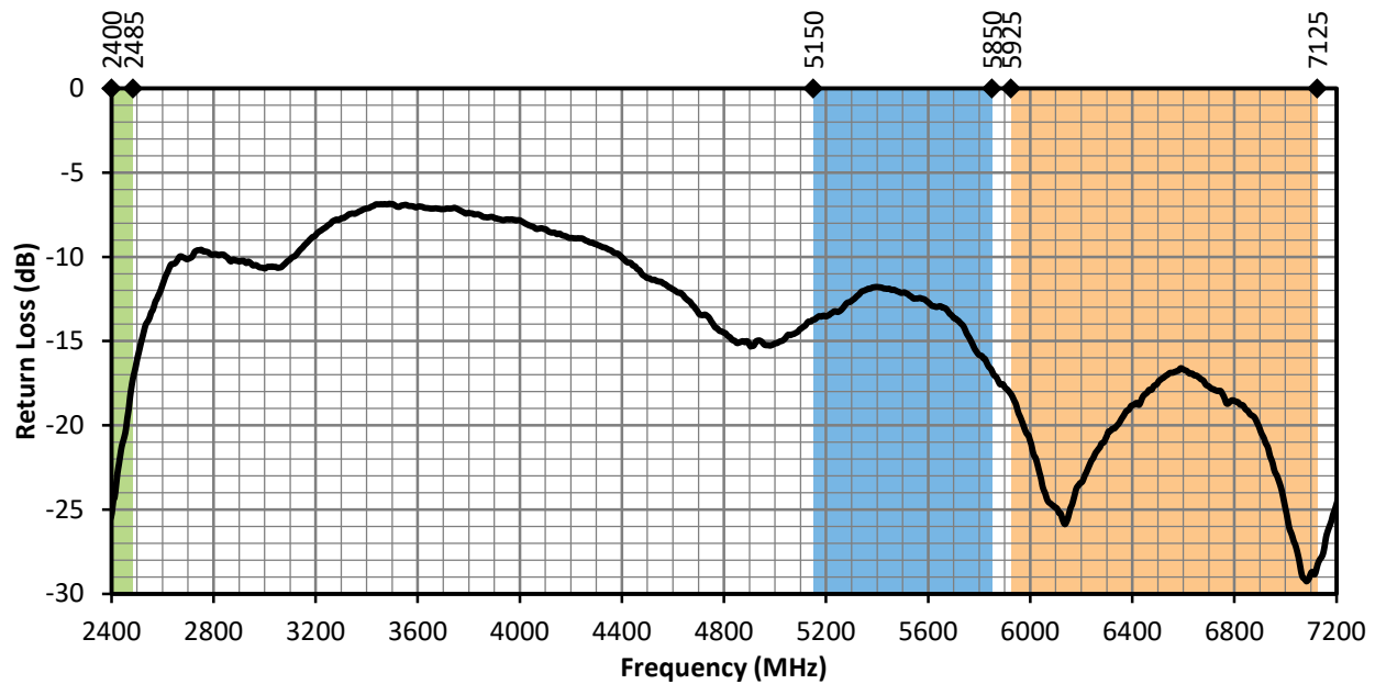
Figure 12. ANT-W63WS2-ccc Return Loss, Edge-Bent
