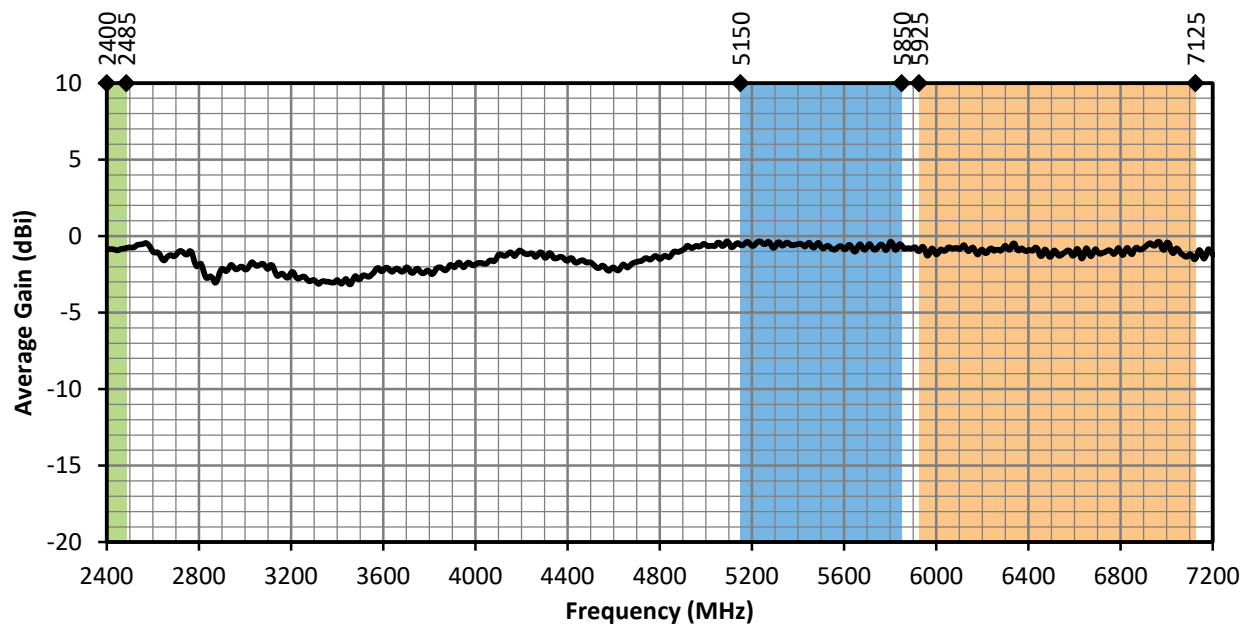
Figure 7. ANT-W63WS2-ccc Antenna Average Gain, Straight
