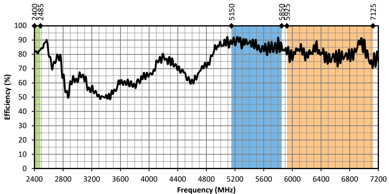
Figure 8. ANT-W63WS2-ccc Antenna Efficiency, Straight
