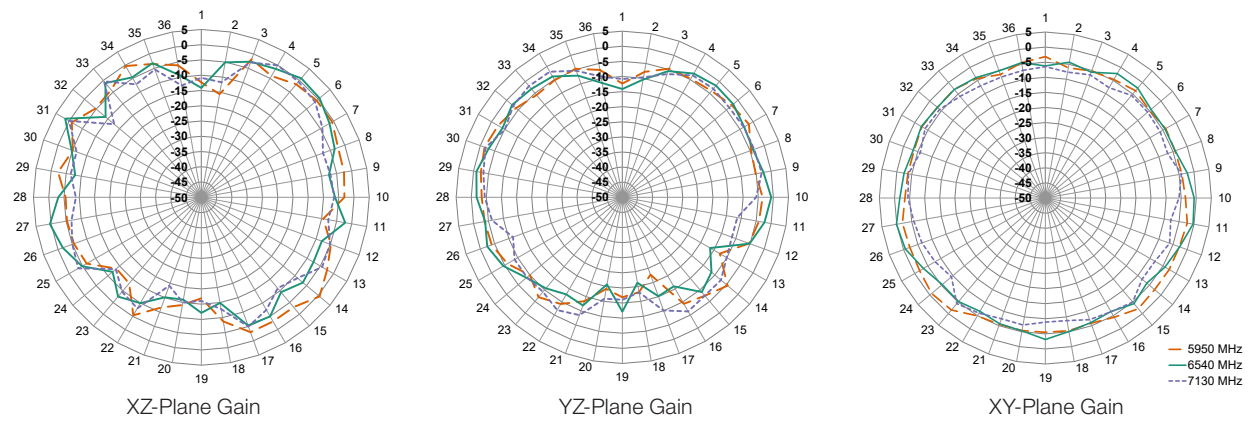
Figure 16. Radiation Patterns for ANT-W63WS2-ccc, Edge-Bent
