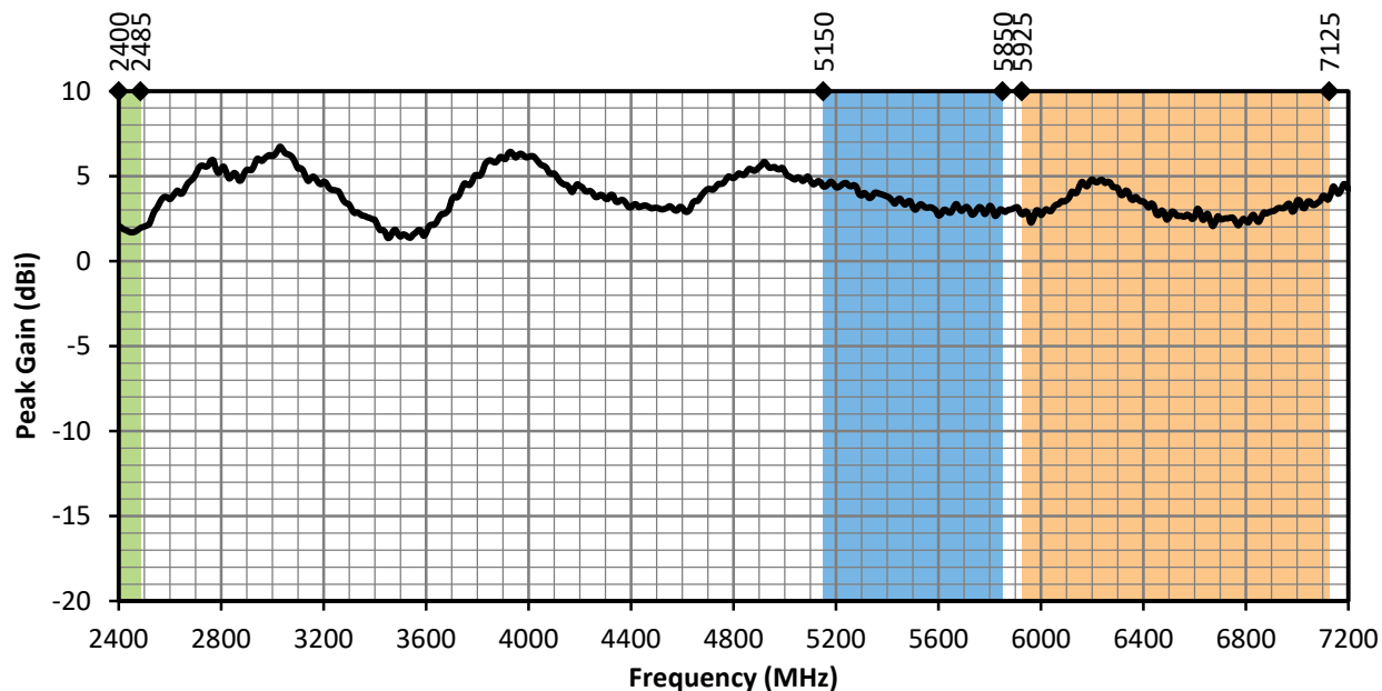
Figure 6. ANT-W63WS2-ccc Peak Gain, Straight
