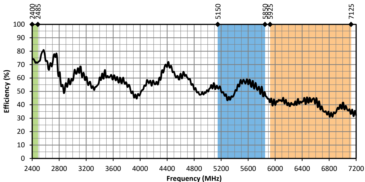
Figure 15. ANT-W63WS2-ccc Antenna Efficiency, Edge-Bent
