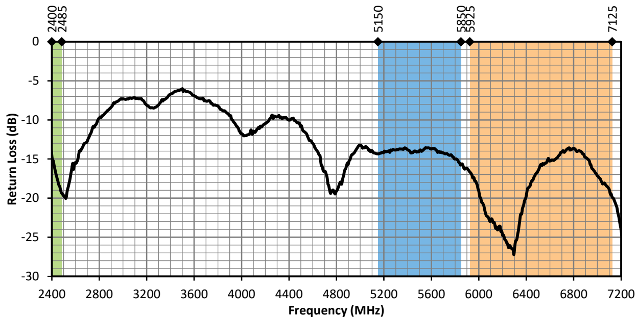
Figure 5. ANT-W63WS2-ccc Return Loss, Straight
