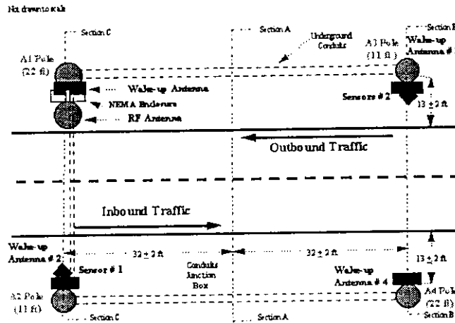
Figure 3-2 Four-pole configuration
