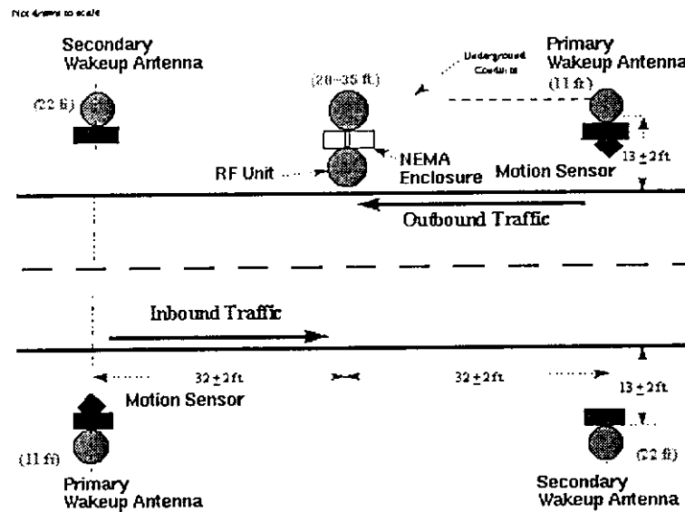
Figure 3-1 Five-pole configuration
