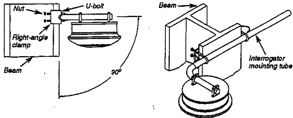
Figure 2-9 Beam Mounting Kit—perpendicular orientation
