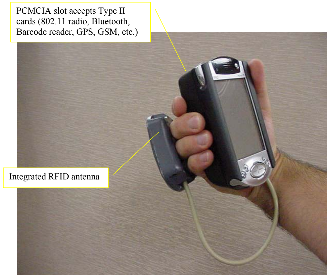
SMR-640P MobileReader connected to PDA handheld
