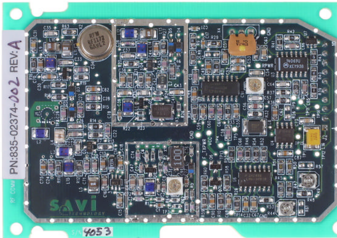
RF Board – Top View with and without shields
