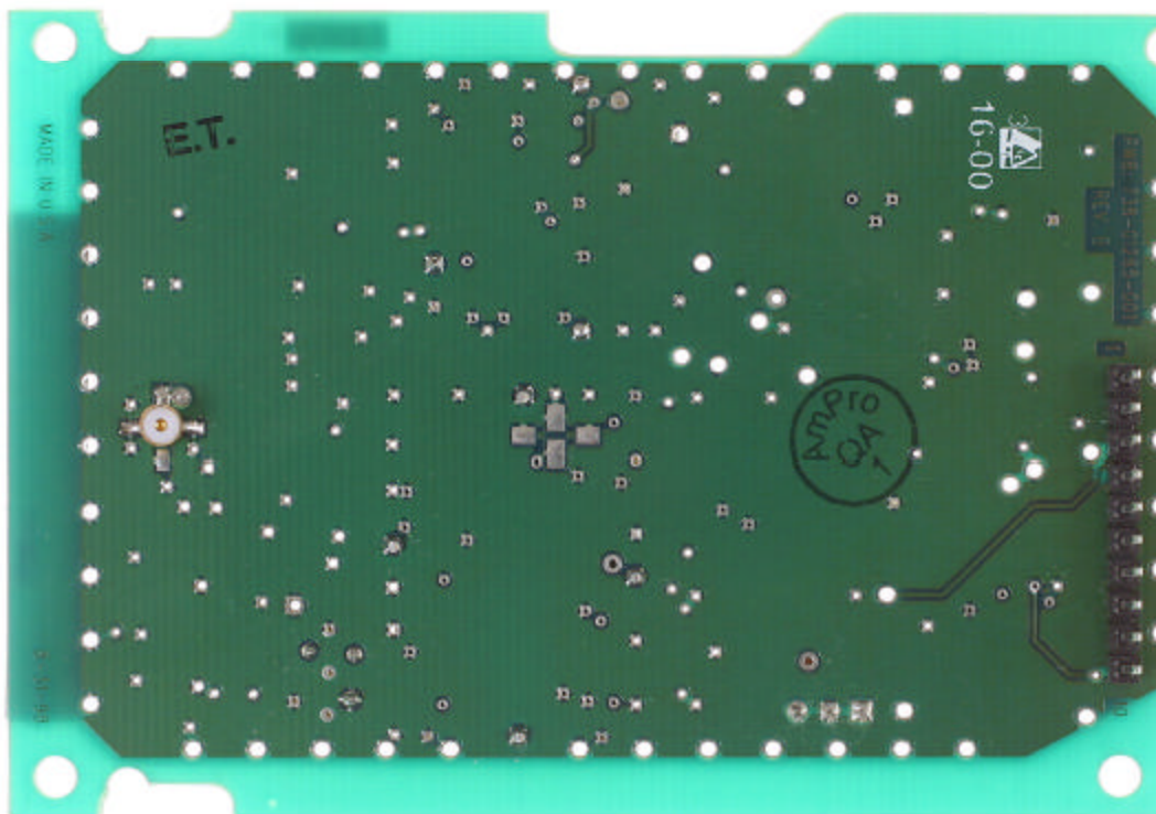
RF Board – Bottom View
