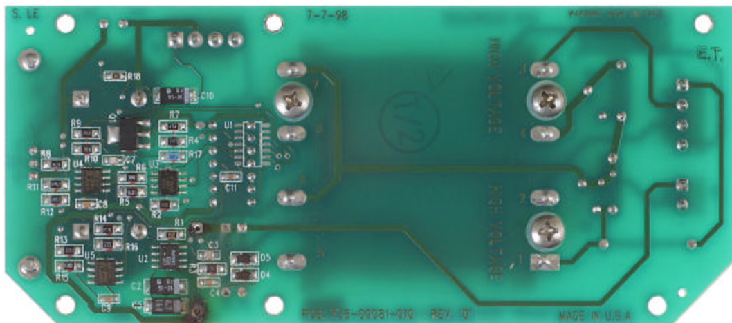
Power Supply Board – Top and Bottom Views
