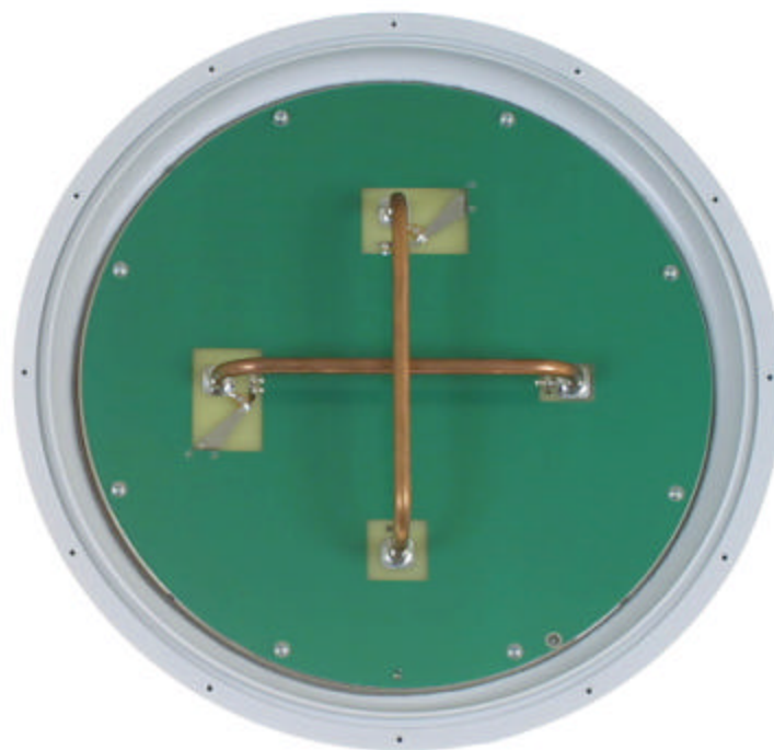
Antenna Board – Top and Bottom
