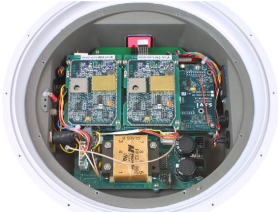
Bottom section – assembly view
