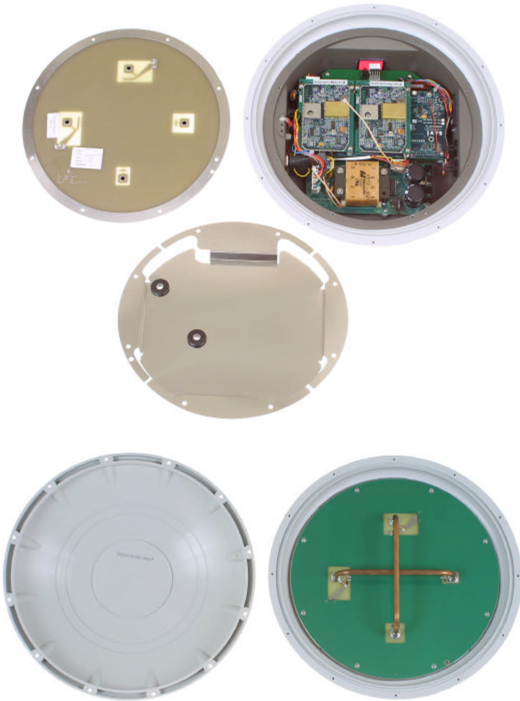
Assembly views – top and bottom sections
