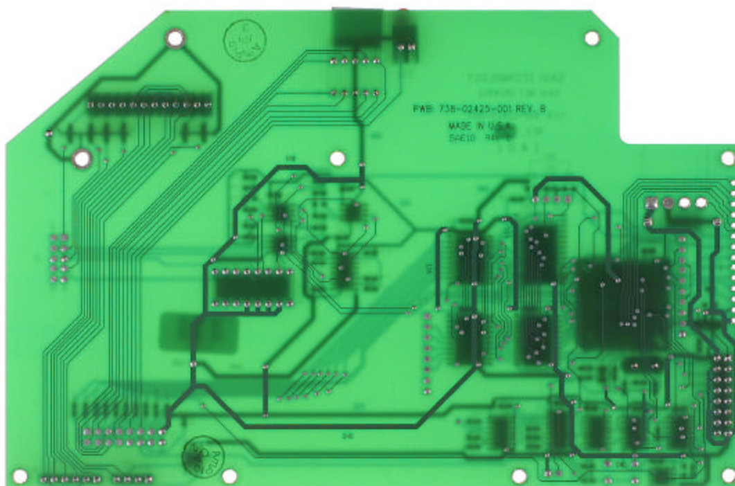
PWB 738-02425-001 Rev B Top and Bottom Views
