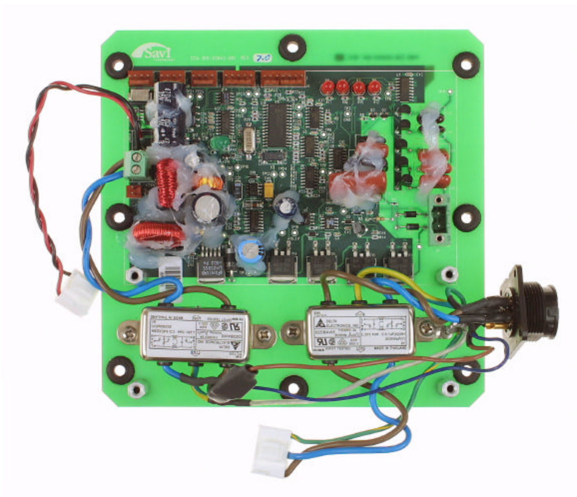
Main Circuit Board – Bottom and Top
