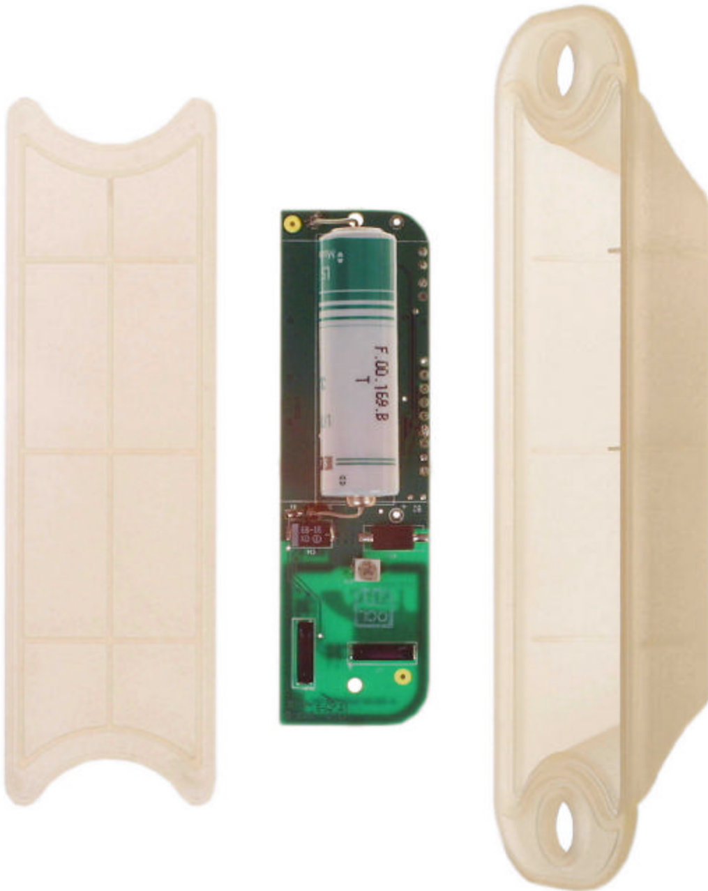
Assembly View
