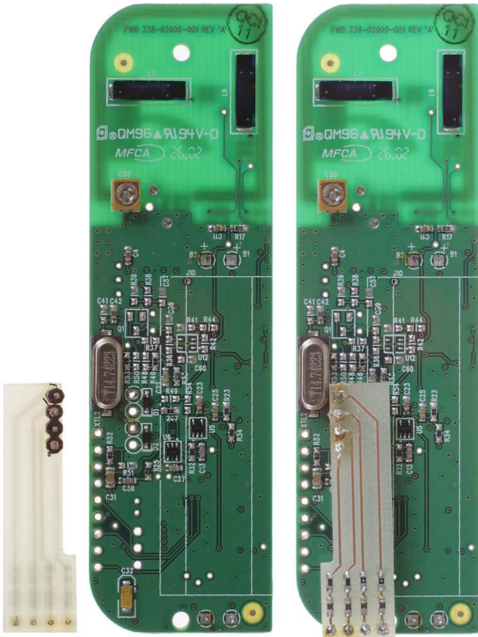
Main circuit board (Top) showing the Daughter Card for the ST-645 Sensor
