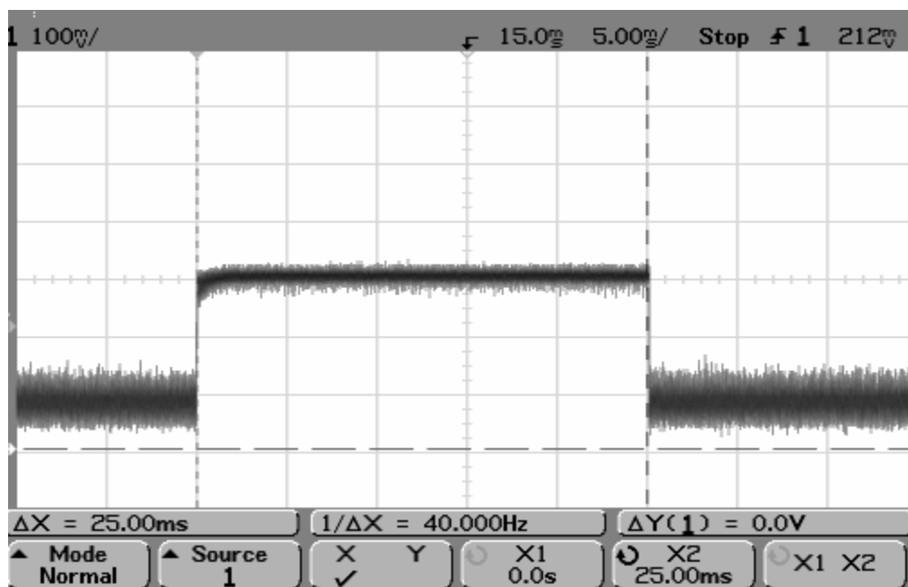
ST-656/675/676 Tag Response to Hello Command (25 msec)
