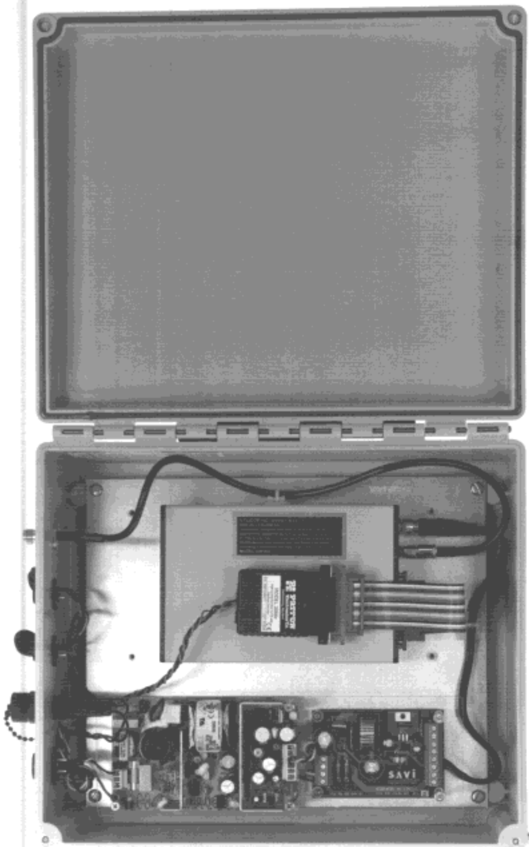
Savi Technology FCC ID: KL7-RELAY-V1 Internal View - RFR100
