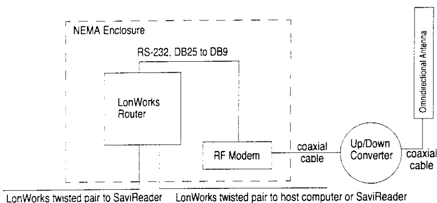
Figure 1-2 Block diagram of Savi RF Relay signal connections (model RFR-200)
