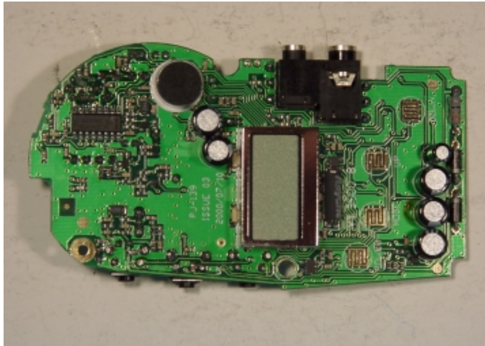
PCB Front
