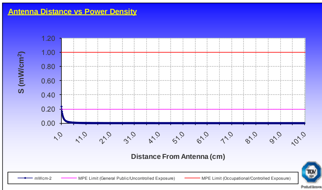
Figure 5 - This graph shows the S field ( \text{mW/cm}^2 ) strength value with regards to distance from the Antenna (cm)
