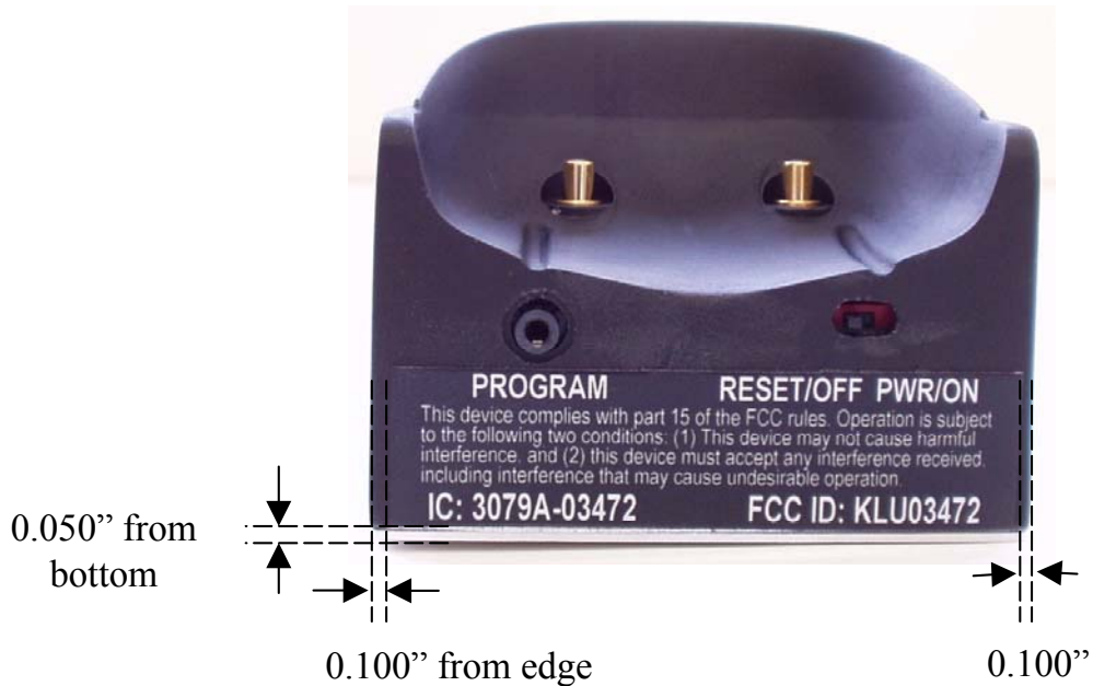
Figure 1 – FCC ID Label Location – Rear View of OVPC2
