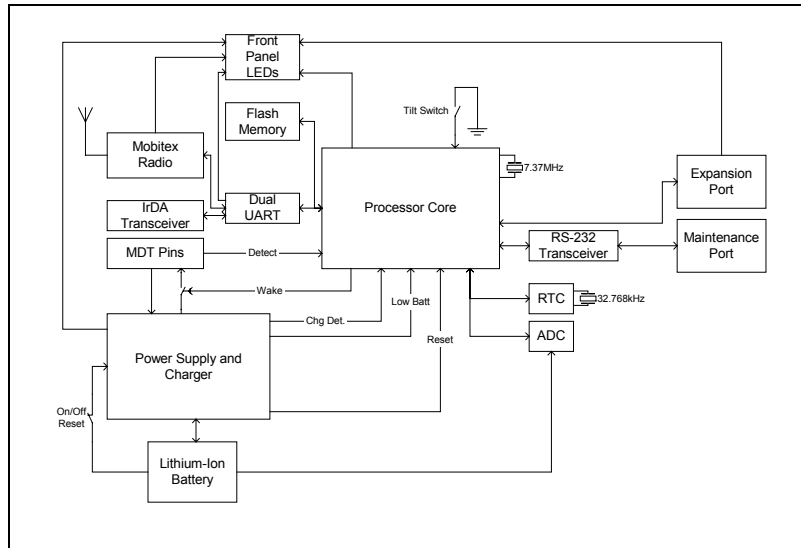
Figure 2 - OVPC2 Block Diagram
