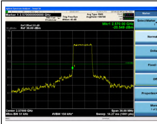
Band 38_QPSK_5M_Low_Full RB Config
