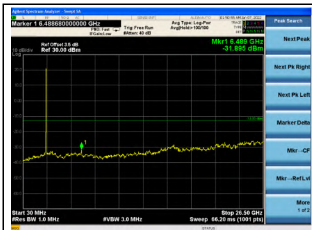
Band 38_QPSK_20M_Low - 30MHz~26.5GHz
