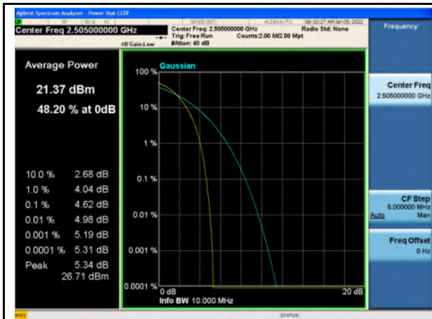
Band 7_QPSK_10M_Low_Full RB Config
