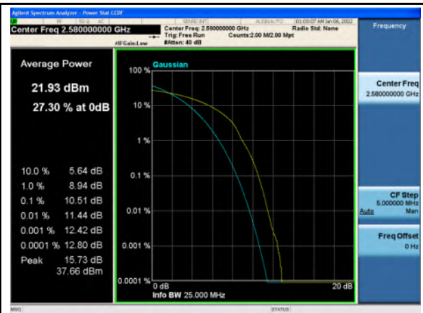
Band 38_16-QAM_20M_Low_Full RB Config
