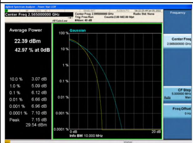
Band 7_16-QAM_10M_High_Full RB Config
