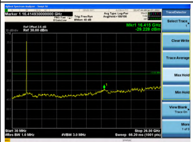
Band 38_QPSK_15M - Mid- 30MHz~26.5GHz
