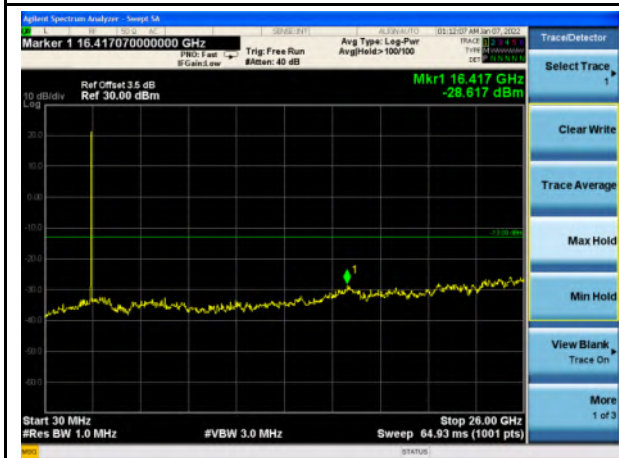
Band 7_QPSK_15M - High - 30MHz~26GHz
