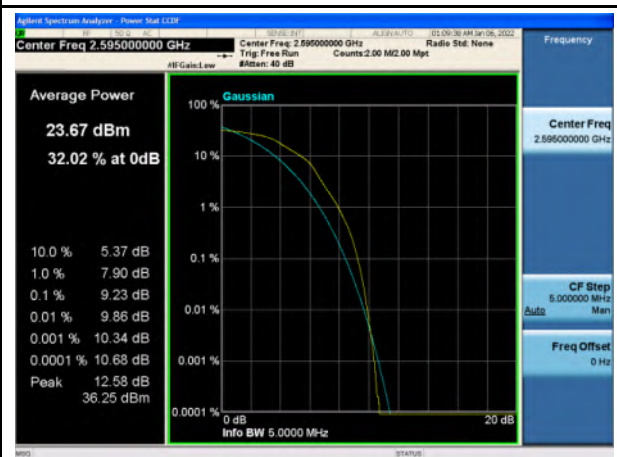
Band 38_16-QAM_5M_Mid_Full RB Config
