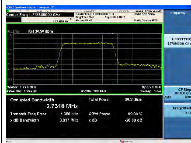
LTE Band 66, QPSK, 3MHz-High CH
