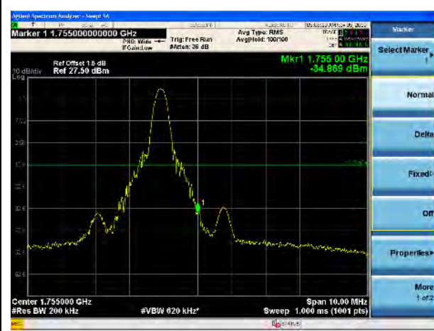
LTE Band 4, QPSK, 20MHz-High CH, 1RB
