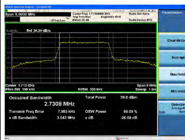
LTE Band 66, 16QAM, 3MHz-Low CH
