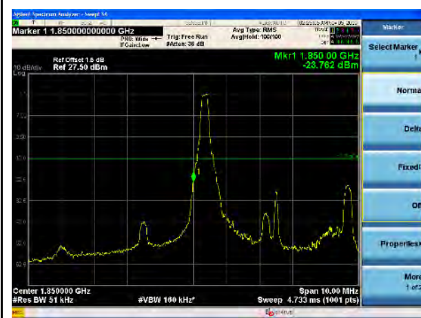
LTE Band 2, QPSK, 5MHz-Low CH, 1RB
