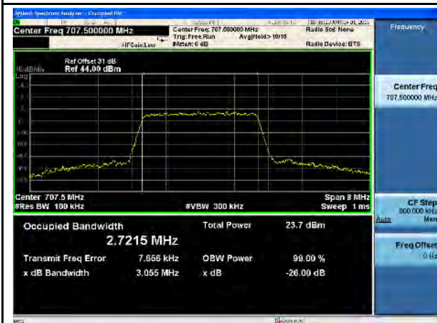
LTE Band 12, 16QAM, 3MHz-Mid CH
