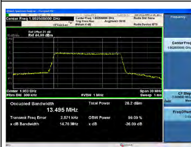
LTE Band 2, QPSK, 15MHz-High CH
