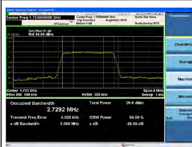
LTE Band 4, QPSK, 3MHz-High CH
