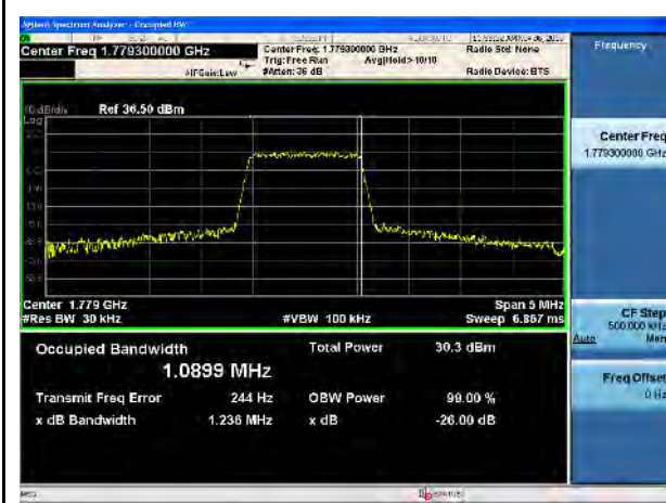
LTE Band 66, QPSK, 1.4MHz-High CH
