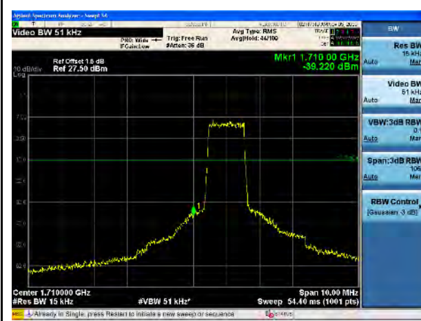
LTE Band 4, QPSK, 1.4MHz-Low CH, 100% RB
