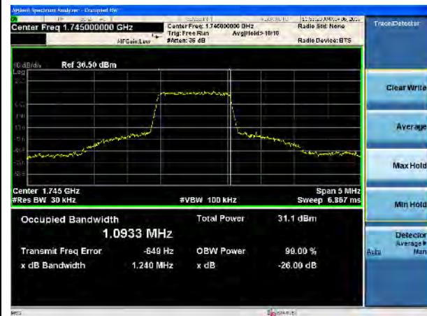
LTE Band 66, QPSK, 1.4MHz-Mid CH
