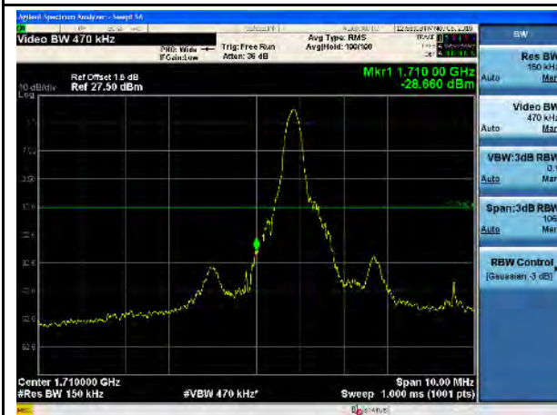
LTE Band 66, 16QAM, 15MHz-Low CH, 1RB
