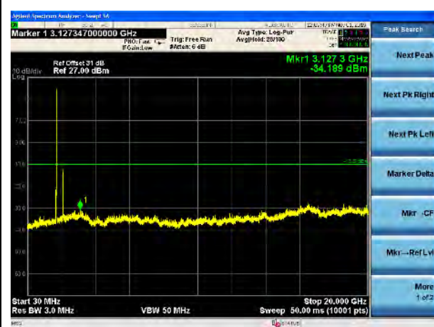
LTE Band 4, 20MHz-Low CH
