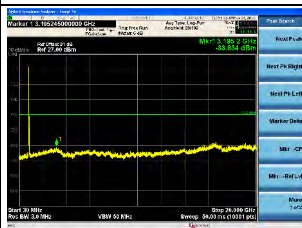
LTE Band 5, 10MHz- High CH
