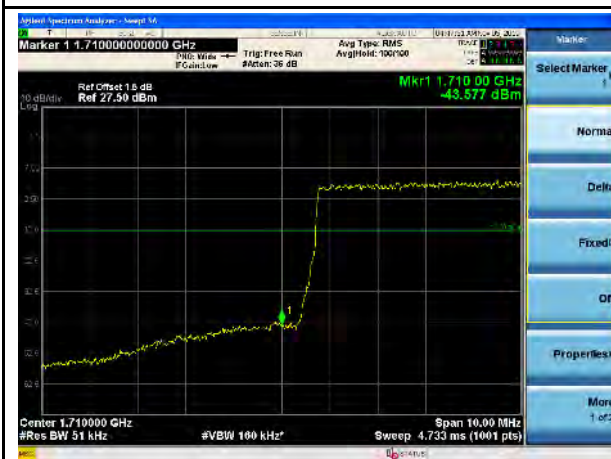
LTE Band 4, 16QAM, 5MHz-Low CH, 100% RB
