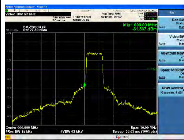
LTE Band 12, QPSK, 1.4MHz-Low CH, 100% RB
