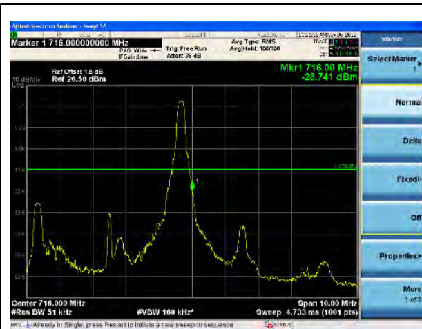
LTE Band 17, QPSK, 5MHz-High CH, 1RB
