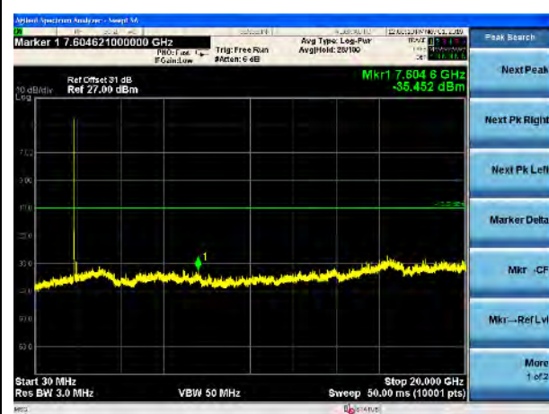
LTE Band 2, 10MHz-Low CH
