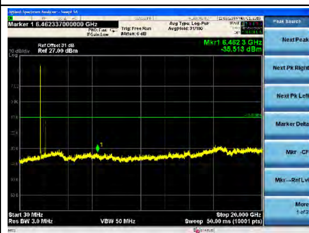
LTE Band 4, 10MHz- High CH
