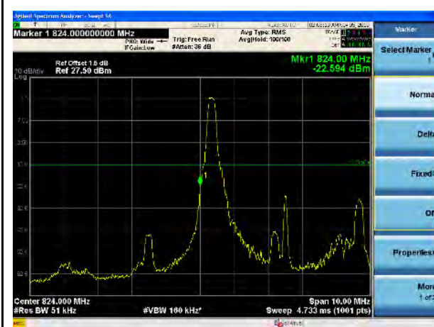
LTE Band 5, QPSK, 5MHz-Low CH, 1RB
