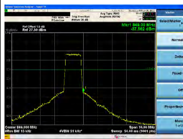
LTE Band 5, 16QAM, 1.4MHz-High CH, 100% RB
