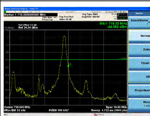
LTE Band 17, 16QAM, 5MHz-High CH, 1RB
