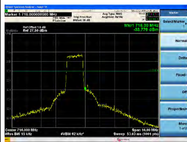
LTE Band 12, 16QAM, 1.4MHz-High CH, 100% RB
