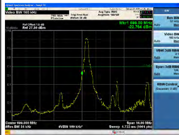
LTE Band 12, 16QAM, 5MHz-Low CH, 1RB
