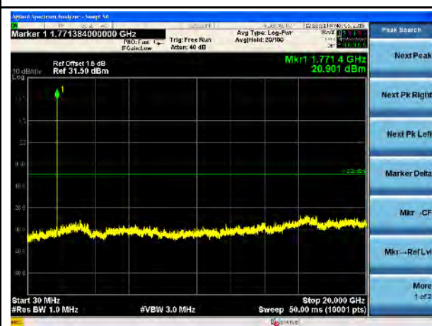
LTE Band 66, 10MHz-High CH
