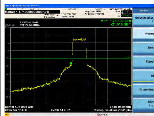
LTE Band 66, QPSK, 1.4MHz-Low CH, 100% RB
