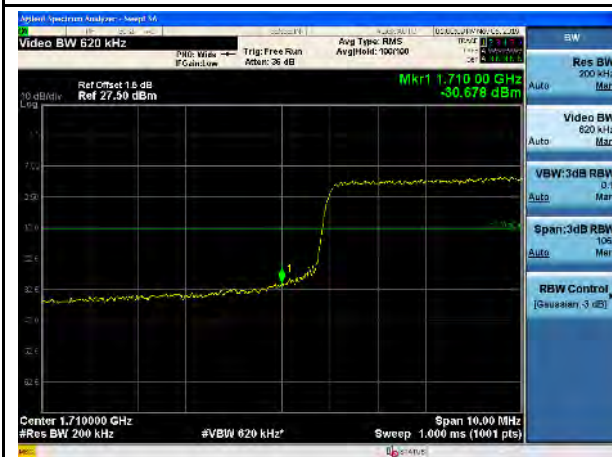
LTE Band 66, QPSK, 20MHz-Low CH, 100% RB
