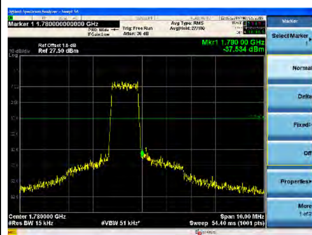
LTE Band 66, 16QAM, 1.4MHz-High CH, 100% RB
