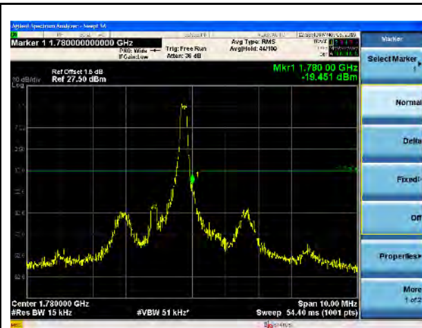
LTE Band 66, QPSK, 1.4MHz-High CH, 1RB
