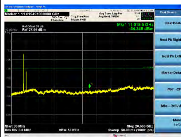
LTE Band 4, 10MHz-Low CH
