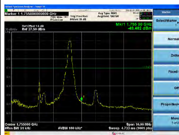
LTE Band 4, 16QAM, 5MHz-High CH, 1RB
