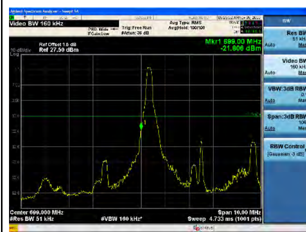
LTE Band 12, QPSK, 5MHz-Low CH, 1RB
