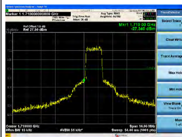
LTE Band 66, 16QAM, 1.4MHz-Low CH, 100% RB
