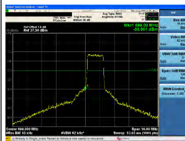
LTE Band 12, 16QAM, 1.4MHz-Low CH, 100% RB
