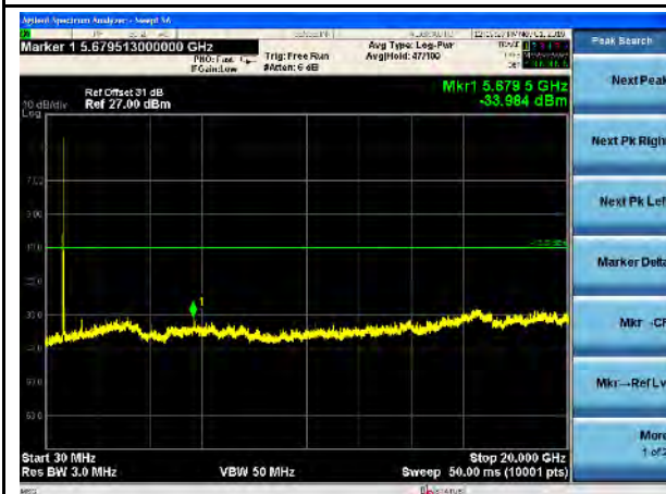
LTE Band 17, 10MHz-Mid CH
