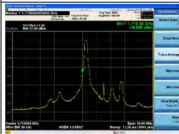
LTE Band 66, QPSK, 3MHz-Low CH, 1RB
