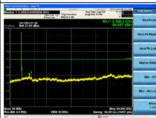
LTE Band 2, 10MHz-High CH
