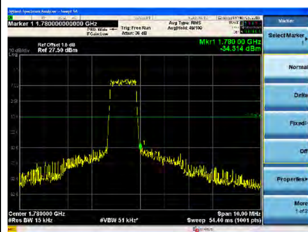
LTE Band 66, QPSK, 1.4MHz-High CH, 100% RB
