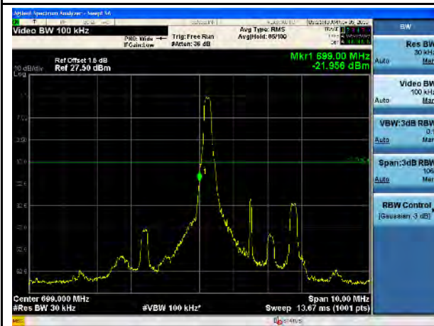
LTE Band 12, QPSK, 3MHz-Low CH, 1RB
