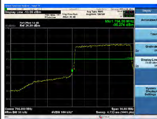
LTE Band 17, QPSK, 5MHz-Low CH, 100% RB
