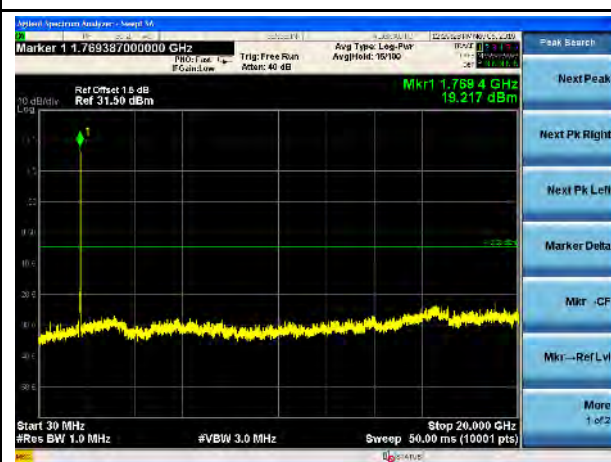
LTE Band 66, 20MHz-High CH
