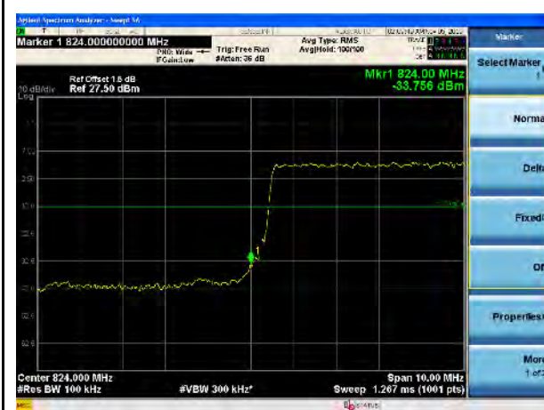
LTE Band 5, QPSK, 10MHz-Low CH, 100% RB
