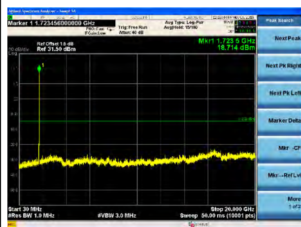
LTE Band 66, 20MHz-Low CH
