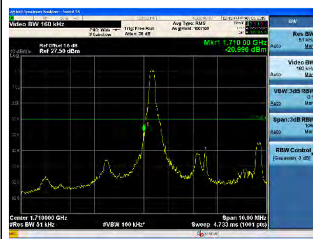
LTE Band 66, 16QAM, 5MHz-Low CH, 1RB
