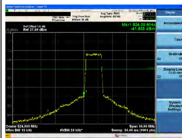
LTE Band 5, 16QAM, 1.4MHz-Low CH, 100% RB
