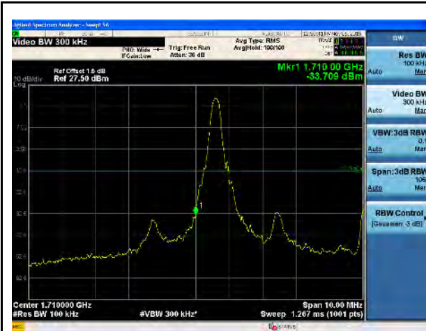
LTE Band 66, QPSK, 10MHz-Low CH, 1RB
