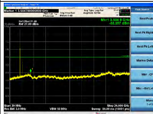
LTE Band 4, 3MHz- High CH
