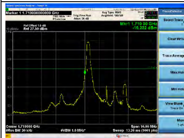
LTE Band 66, 16QAM, 3MHz-Low CH, 1RB
