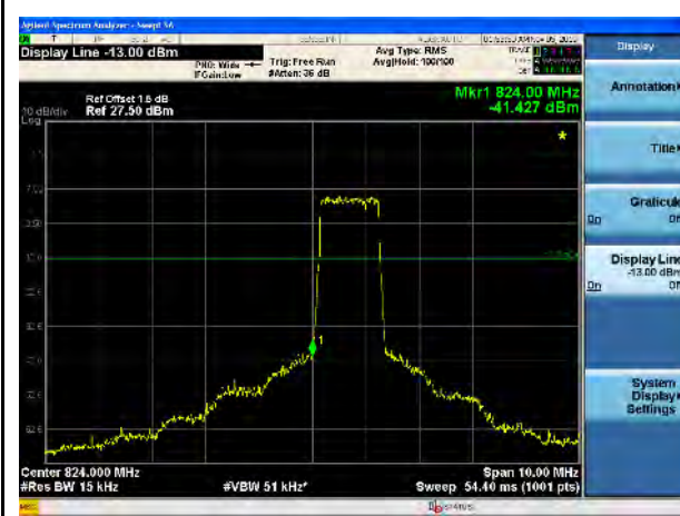
LTE Band 5, QPSK, 1.4MHz-Low CH, 100% RB
