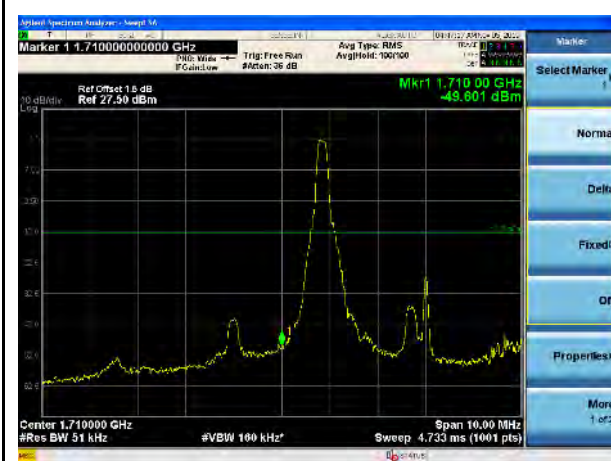
LTE Band 4, 16QAM, 5MHz-Low CH, 1RB
