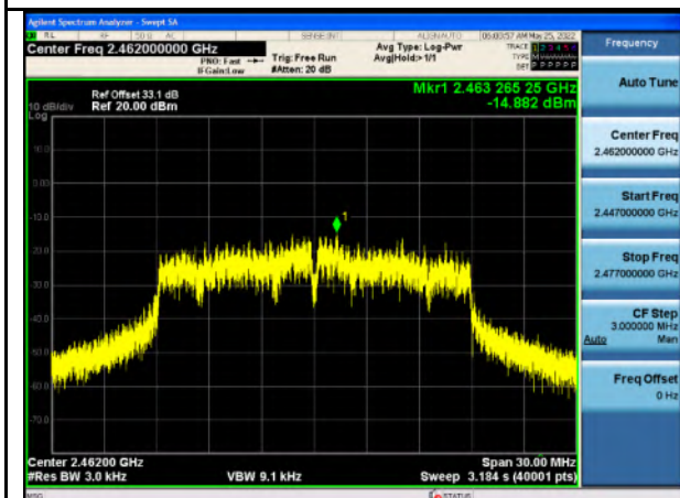
PSD-802.11n20-High CH
