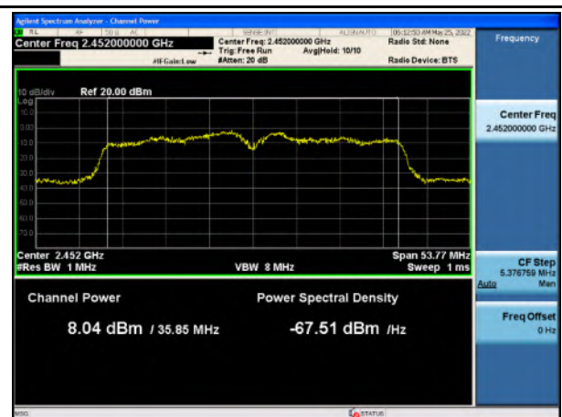
OP_802.11n40_High CH
