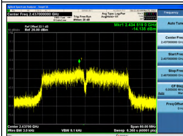
PSD-802.11n40-Mid CH
