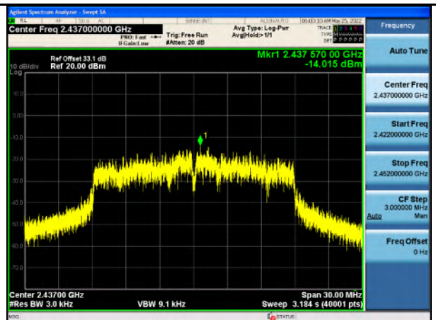
PSD-802.11n20-Mid CH
