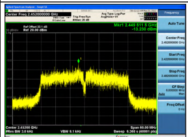
PSD-802.11n40-High CH
