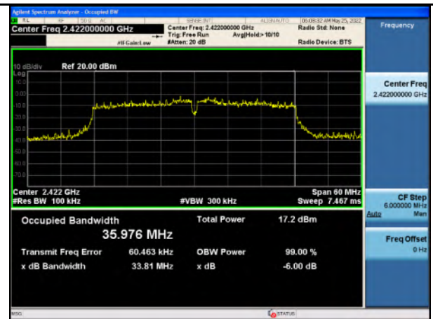
99%_802.11n40_Low CH
