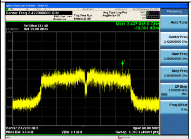
PSD-802.11n40-Low CH
