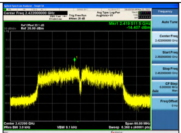
PSD-802.11n40-Low CH
