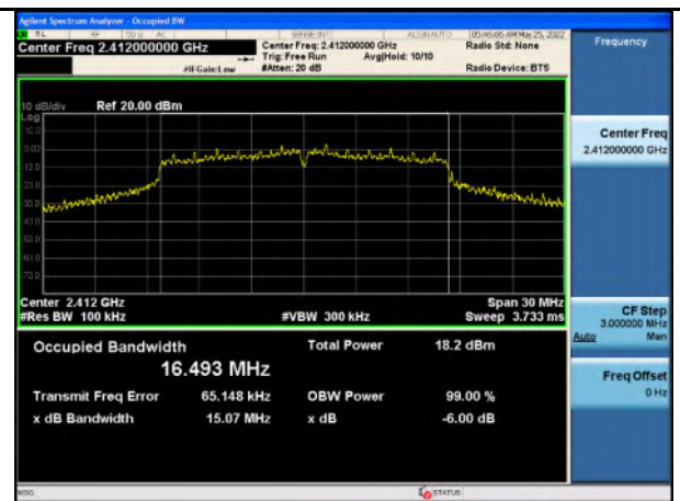
99%_802.11g_Low CH
