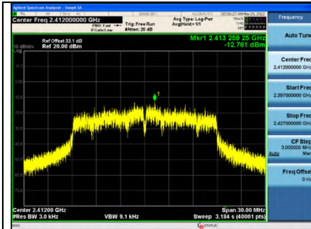
PSD-802.11n20-Low CH
