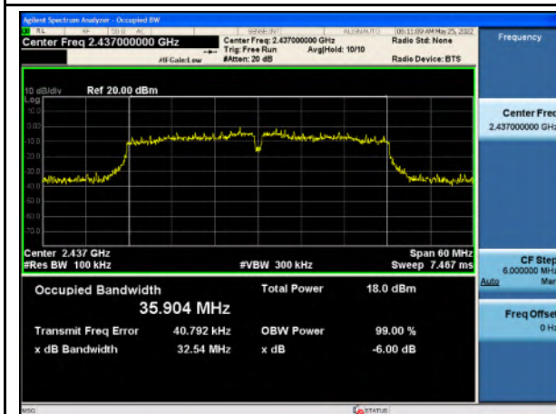
99%_802.11n40_Mid CH
