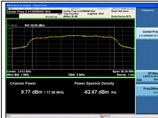
OP_802.11n_Low CH
