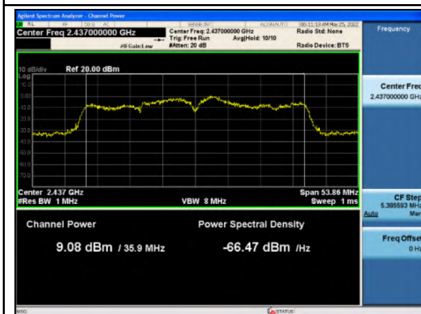
OP_802.11n40_Mid CH
