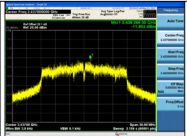
PSD-802.11n20-Mid CH
