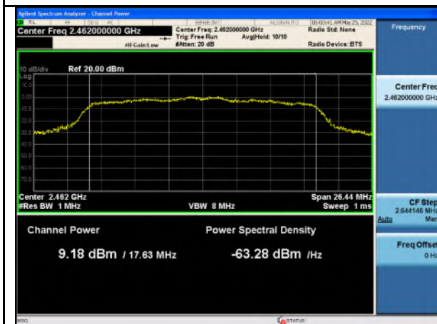
OP_802.11n_High CH
