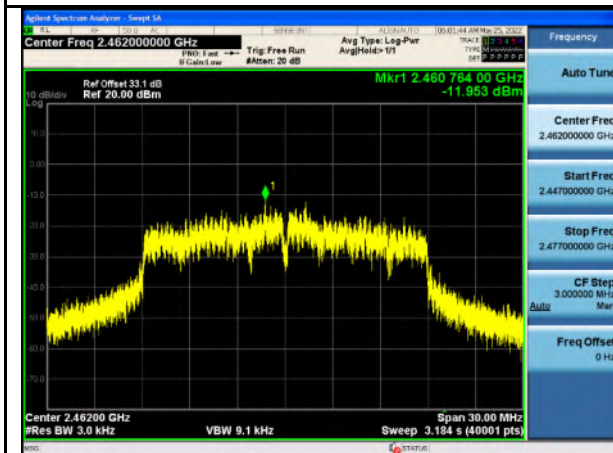
PSD-802.11n20-High CH
