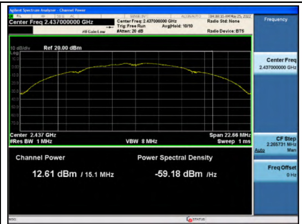
OP_802.11b_Mid CH
