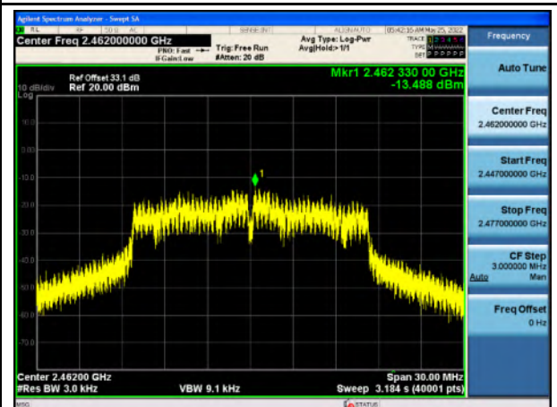
PSD-802.11g-High CH
