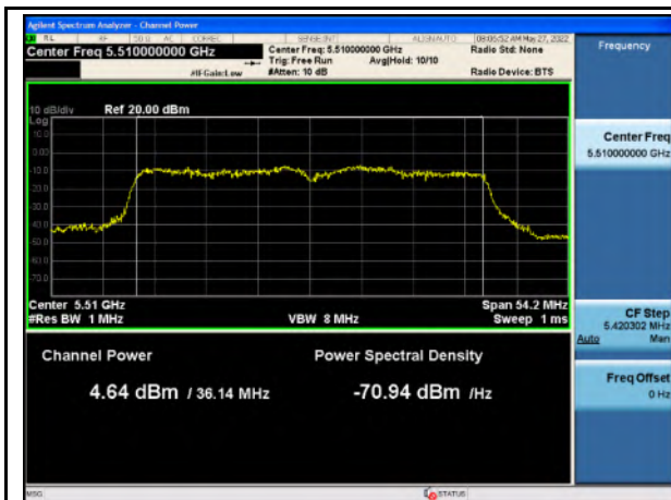
Output Power_U-NII-2C_802.11n40_5510
