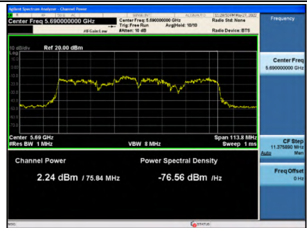
Output Power_Cross band_802.11ac80_5690
