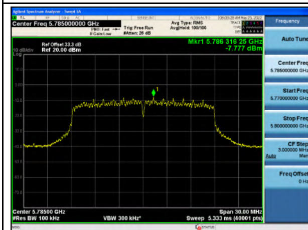
PSD_U-NII-3_802.11n_5785
