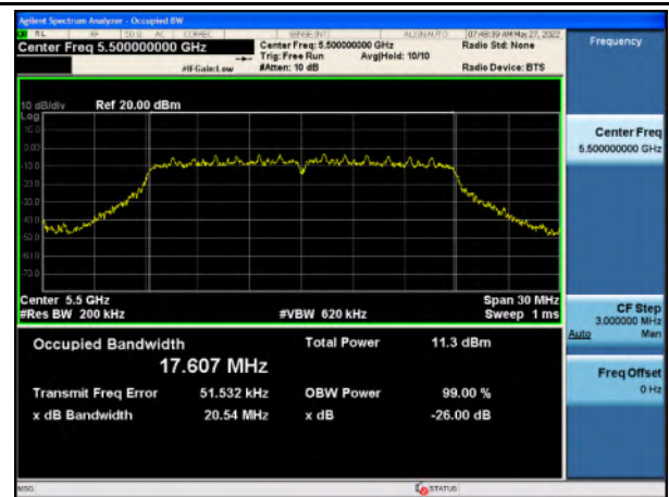
26 dB & 99% BW_U-NII-2C_802.11n_5500
