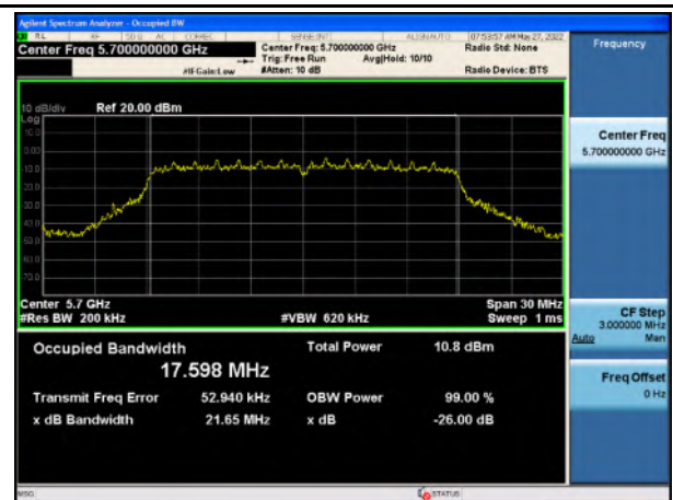
26 dB & 99% BW_U-NII-2C_802.11n_5700
