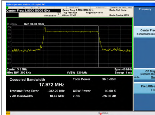
n77_Low Band_16QAM_20M_Mid_Full RB Config
