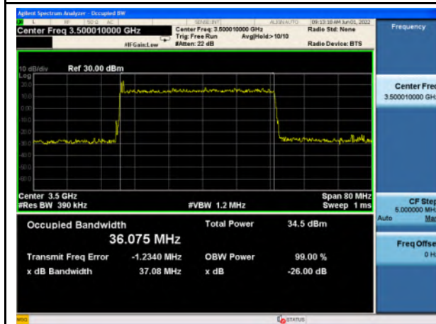
n77_Low Band_256QAM_40M_Mid_Full RB Config
