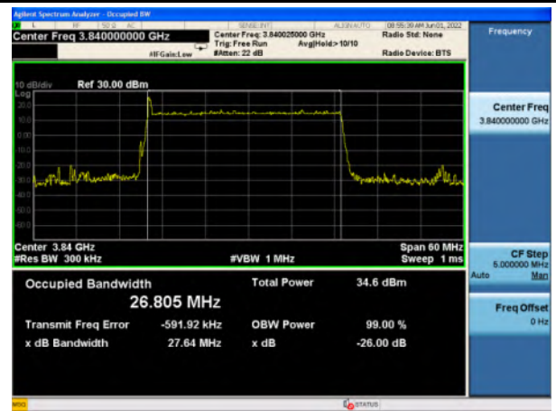
n77_High Band_64QAM_30M_Mid_Full RB Config
