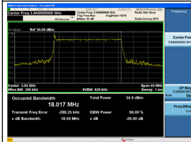
n77_High Band_16QAM_20M_Mid_Full RB Config
