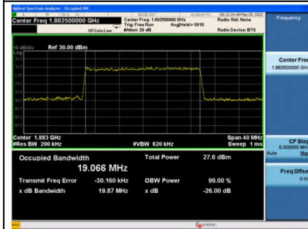
n2_256QAM_20M_Mid_Full RB Config
