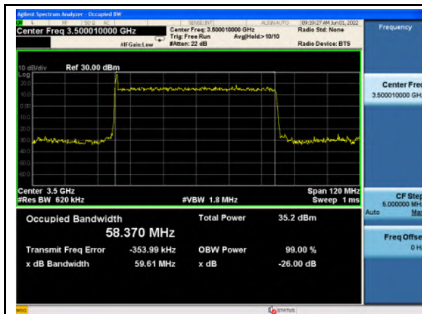
n77_Low Band_Pi/2 BPSK_60M_Mid_Full RB Config
