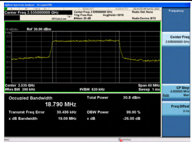
n7_64QAM_20M_Mid_Full RB Config
