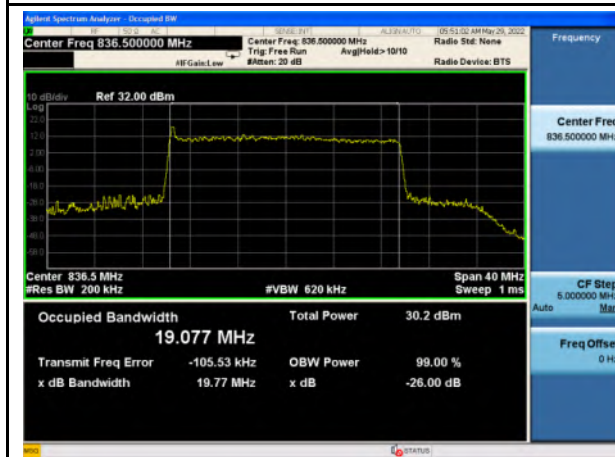
n5_256QAM_20M_Mid_Full RB Config
