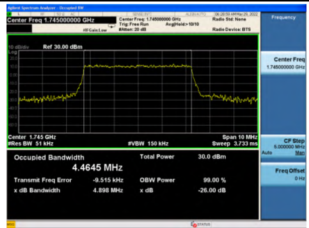
n66_64QAM_5M_Mid_Full RB Config
