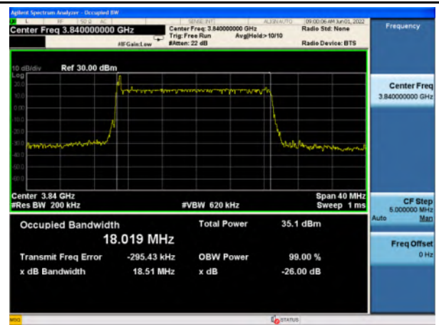
n77_High Band_64QAM_20M_Mid_Full RB Config
