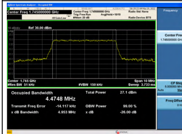
n66_256QAM_5M_Mid_Full RB Config
