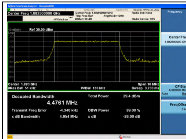
n2_Pi/2 BPSK_5M_Mid_Full RB Config
