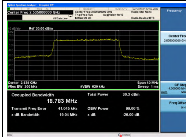
n7_256QAM_20M_Mid_Full RB Config
