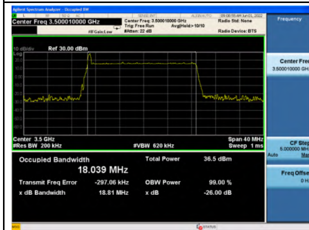
n77_Low Band_256QAM_20M_Mid_Full RB Config
