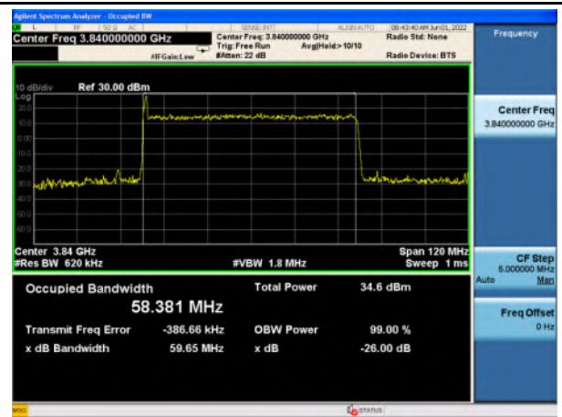
n77_High Band_64QAM_60M_Mid_Full RB Config
