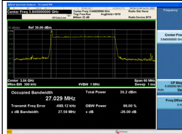
n77_High Band_16QAM_30M_Mid_Full RB Config
