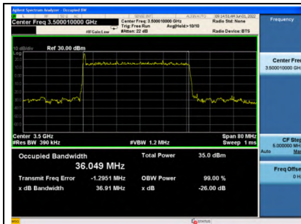
n77_Low Band_Pi/2 BPSK_40M_Mid_Full RB Config
