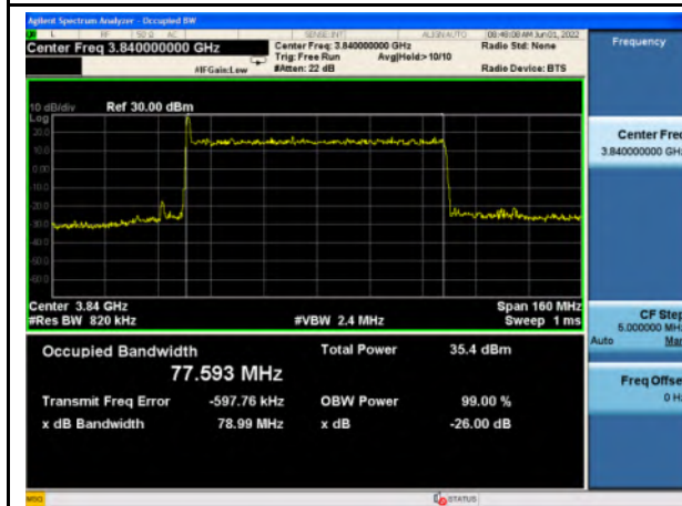
n77_High Band_256QAM_80M_Mid_Full RB Config
