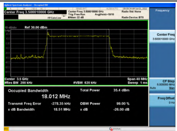
n77_Low Band_64QAM_20M_Mid_Full RB Config
