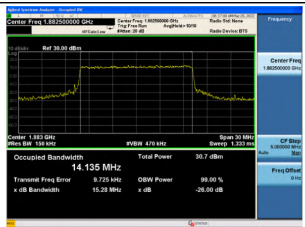
n2_QPSK_15M_Mid_Full RB Config
