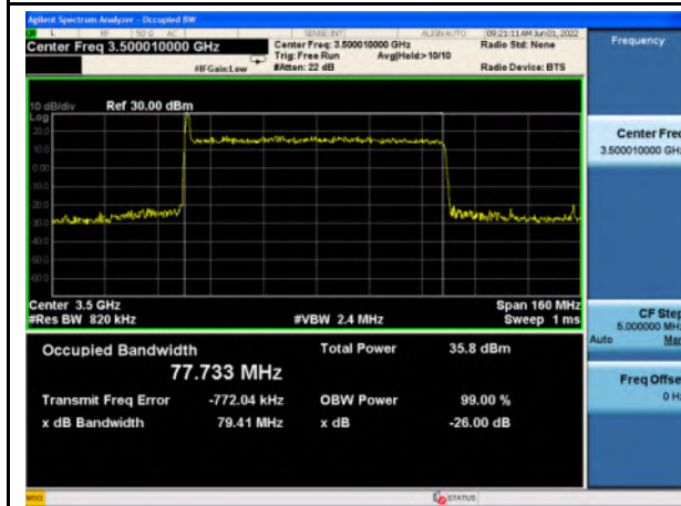
n77_Low Band_16QAM_80M_Mid_Full RB Config
