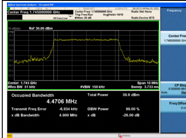
n66_16QAM_5M_Mid_Full RB Config
