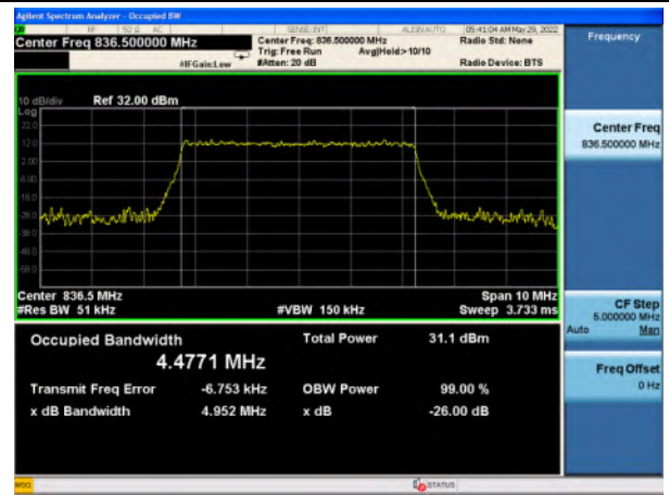
n5_64QAM_5M_Mid_Full RB Config
