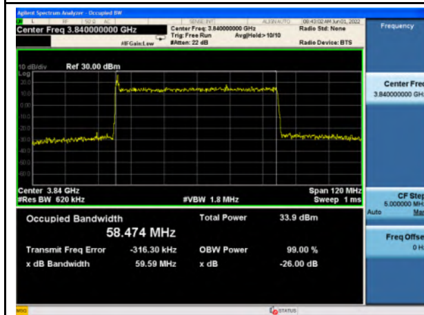
n77_High Band_256QAM_60M_Mid_Full RB Config
