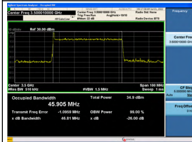
n77_Low Band_256QAM_50M_Mid_Full RB Config
