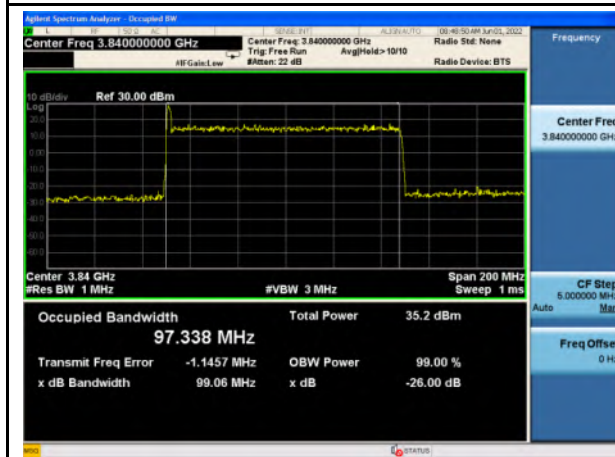
n77_High Band_256QAM_100M_Mid_Full RB Config
