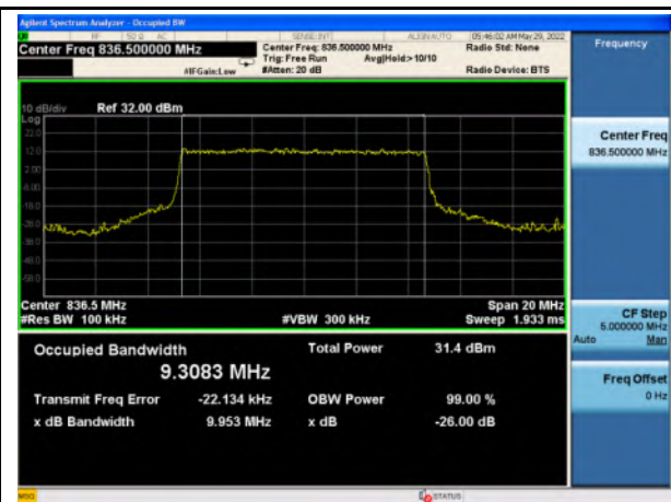
n5_QPSK_10M_Mid_Full RB Config
