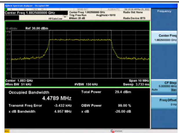
n2_QPSK_5M_Mid_Full RB Config
