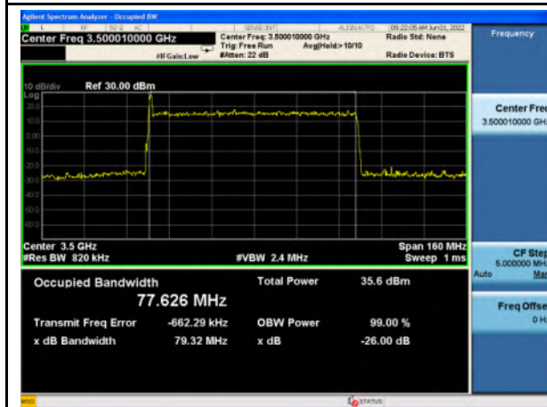
n77_Low Band_256QAM_80M_Mid_Full RB Config
