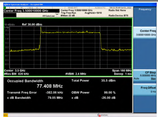
n77_Low Band_64QAM_80M_Mid_Full RB Config
