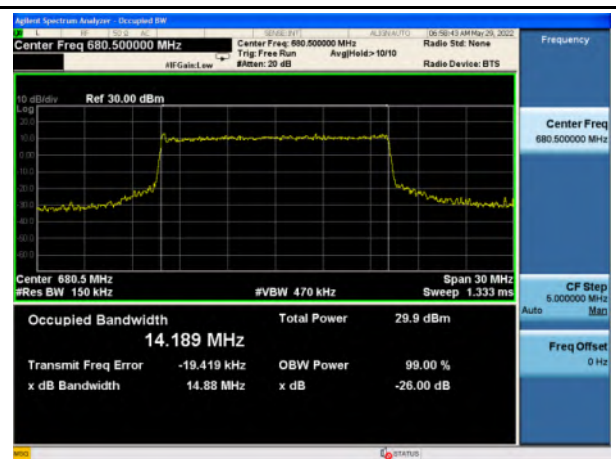
n71_QPSK_15M_Mid_Full RB Config
