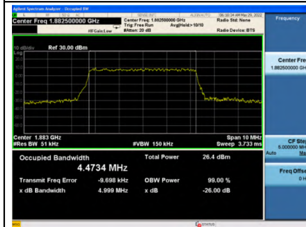
n2_256QAM_5M_Mid_Full RB Config
