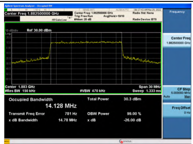
n2_64QAM_15M_Mid_Full RB Config
