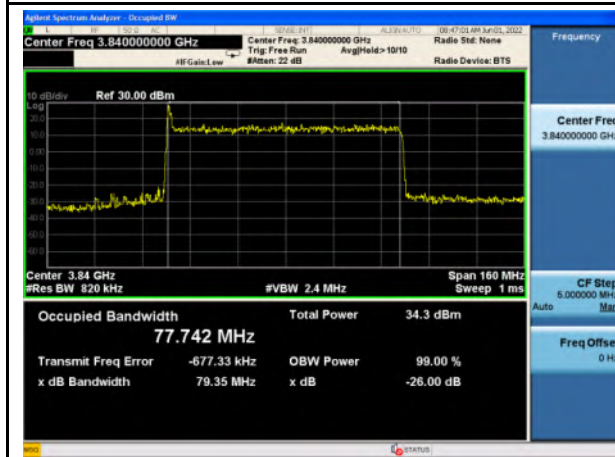
n77_High Band_16QAM_80M_Mid_Full RB Config
