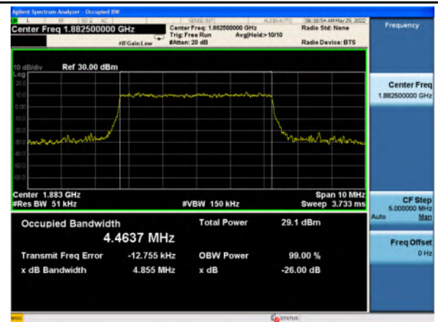
n2_64QAM_5M_Mid_Full RB Config
