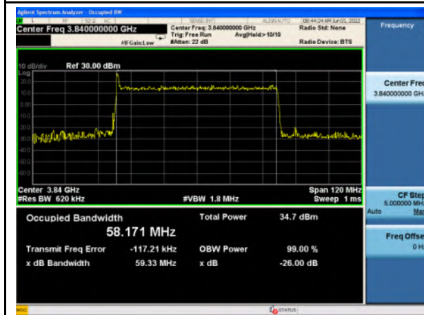
n77_High Band_16QAM_60M_Mid_Full RB Config
