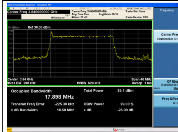
n77_High Band_256QAM_20M_Mid_Full RB Config
