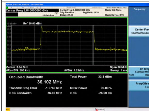
n77_High Band_256QAM_40M_Mid_Full RB Config
