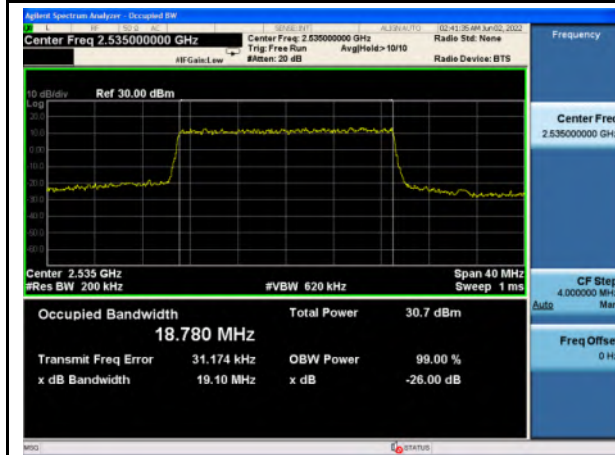
n7_16QAM_20M_Mid_Full RB Config
