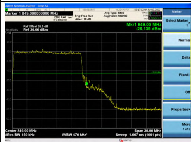
n5_15MHz_Upper Band Edge
