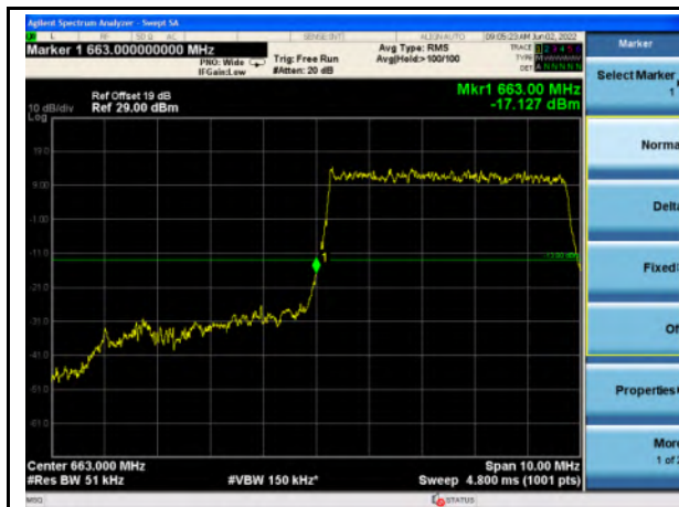
n71_5MHz_Lower Band Edge
