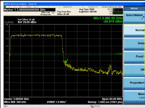
n77_Higher Band_30MHz_Upper Band Edge
