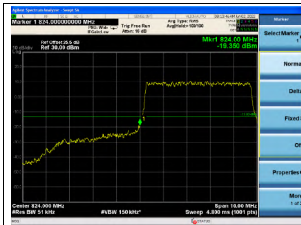
n5_5MHz_Lower Band Edge
