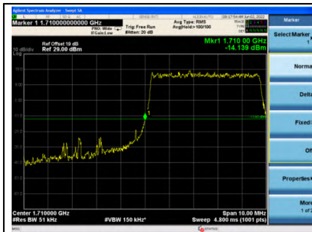
n66_5MHz_Lower Band Edge
