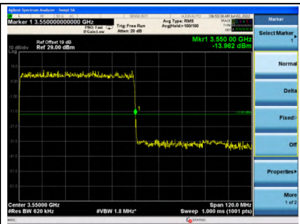
n77_Low Band_60MHz_Upper Band Edge
