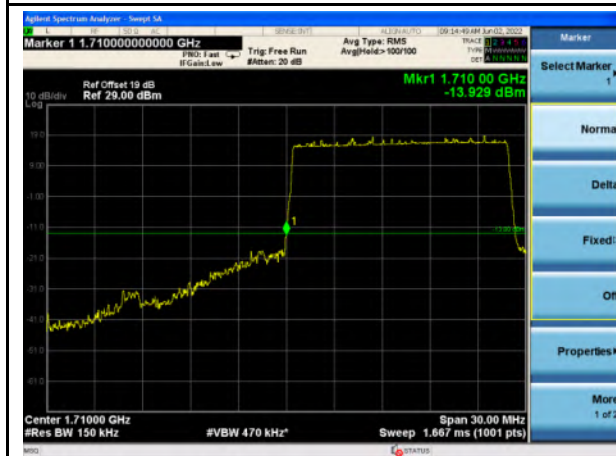
n66_15MHz_Lower Band Edge
