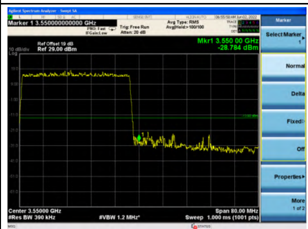
n77_Low Band_40MHz_Upper Band Edge
