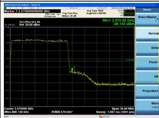
n7_15MHz_Upper Band Edge
