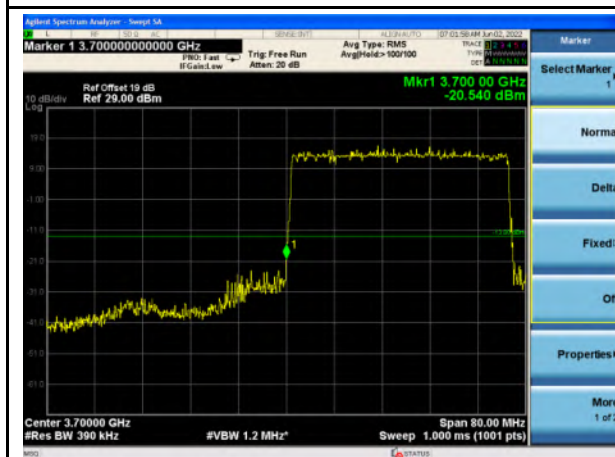
n77_Higher Band_40MHz_Lower Band Edge
