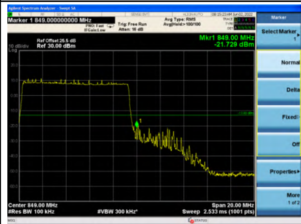
n5_10MHz_Upper Band Edge
