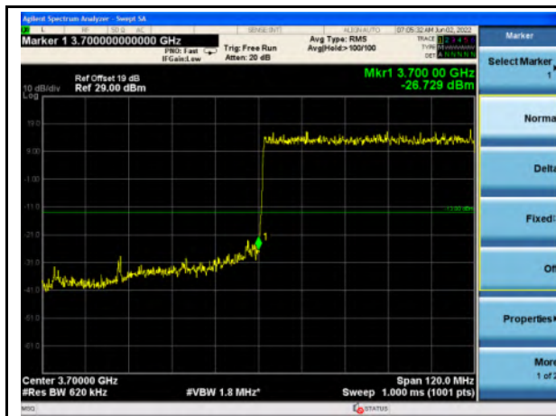
n77_Higher Band_60MHz_Lower Band Edge
