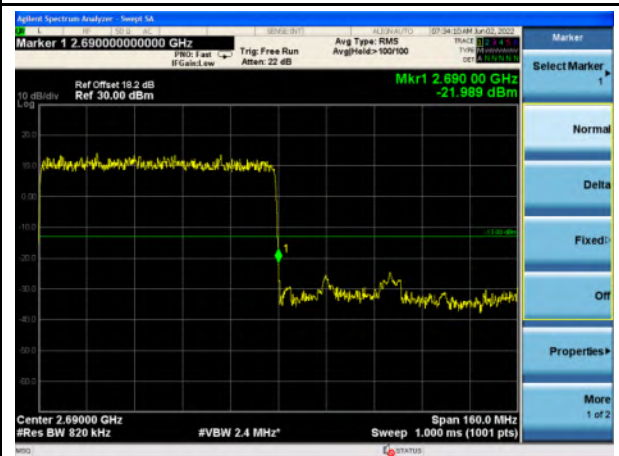
n41_80MHz_Upper Band Edge
