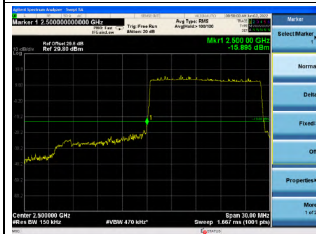
n7_15MHz_Lower Band Edge
