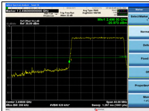
n41_20MHz_Lower Band Edge
