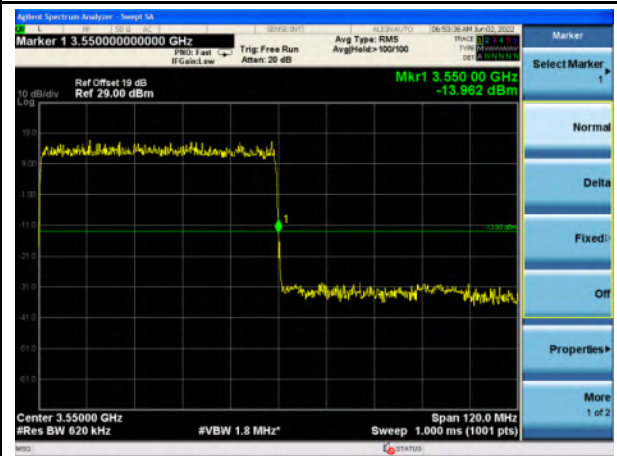
n77_Low Band_80MHz_Upper Band Edge
