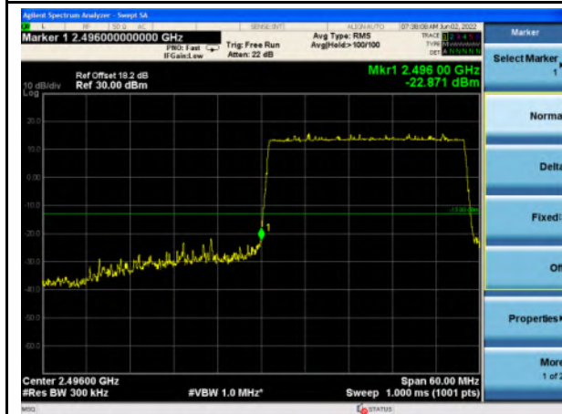
n41_30MHz_Lower Band Edge
