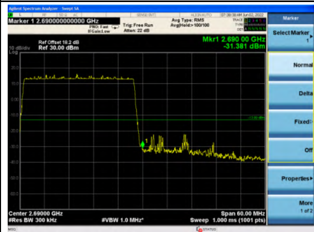
n41_30MHz_Upper Band Edge
