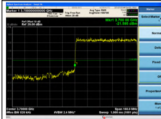
n77_Higher Band_80MHz_Lower Band Edge
