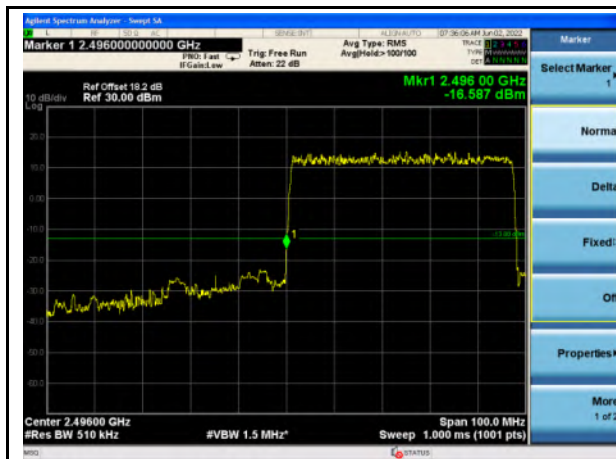
n41_50MHz_Lower Band Edge
