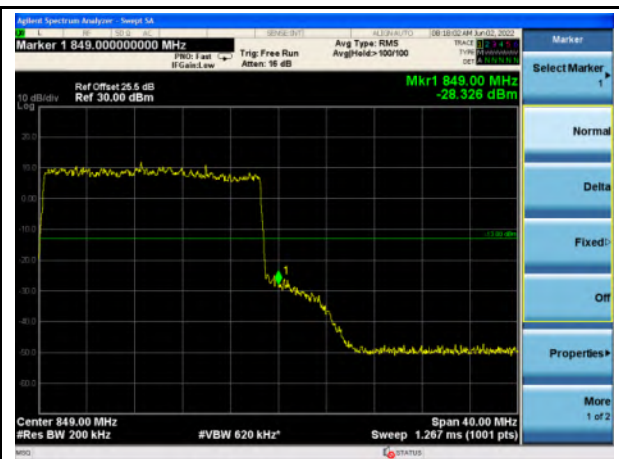
n5_20MHz_Upper Band Edge
