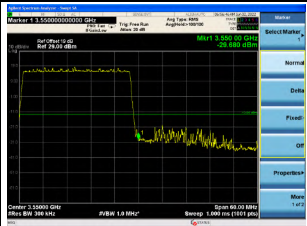
n77_Low Band_30MHz_Upper Band Edge
