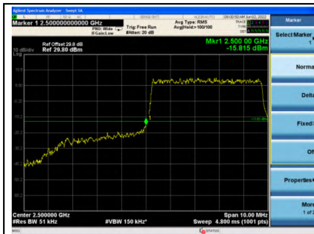
n7_5MHz_Lower Band Edge
