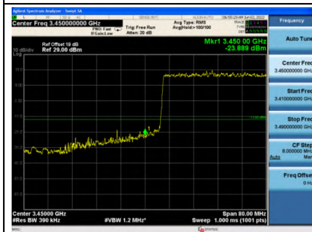
n77_Low Band_40MHz_Lower Band Edge
