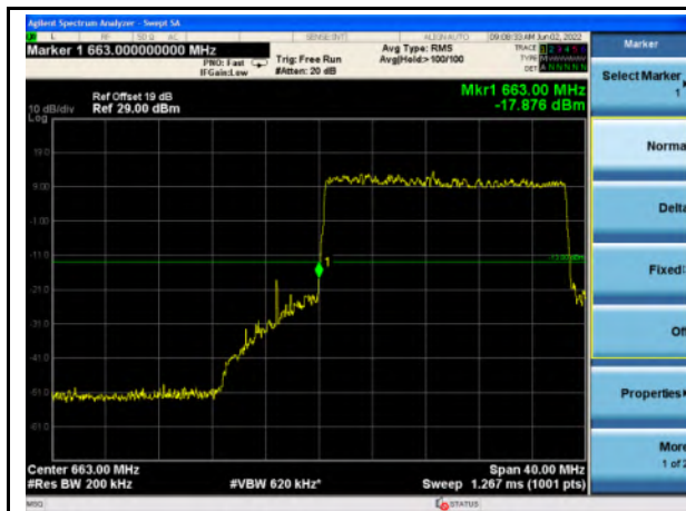
n71_20MHz_Lower Band Edge
