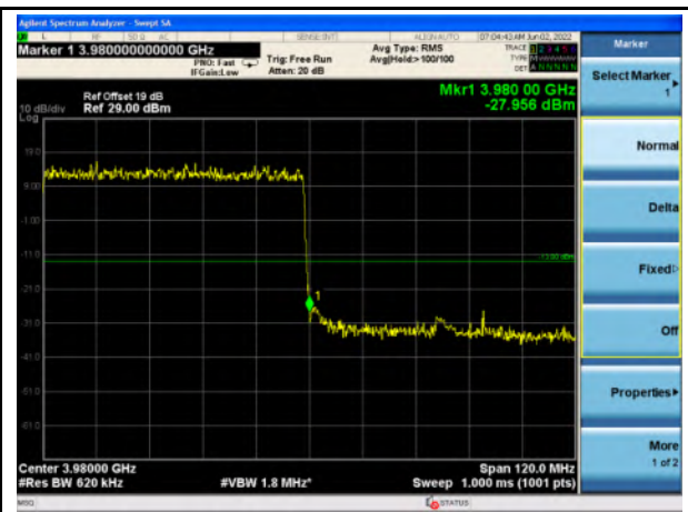
n77_Higher Band_60MHz_Upper Band Edge
