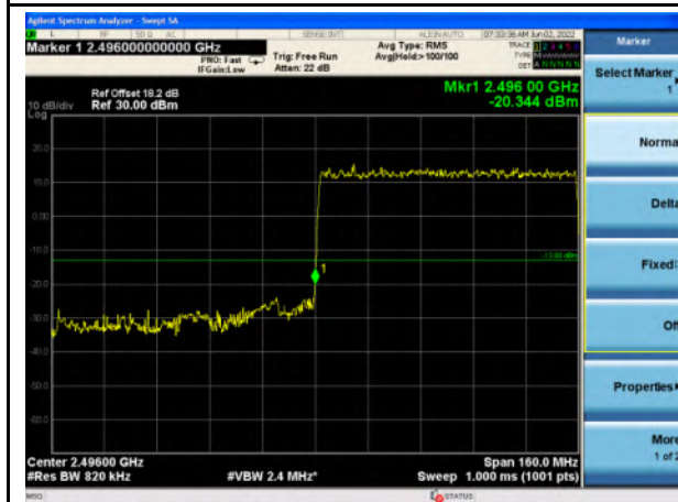
n41_80MHz_Lower Band Edge
