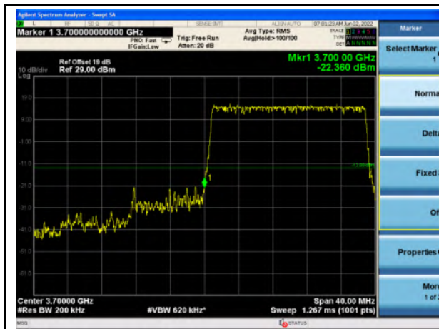
n77_Higher Band_20MHz_Lower Band Edge
