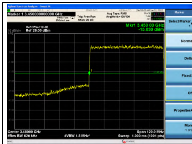
n77_Low Band_60MHz_Lower Band Edge
