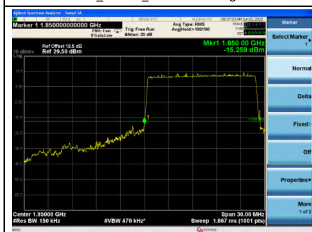
n2_15MHz_Lower Band Edge
