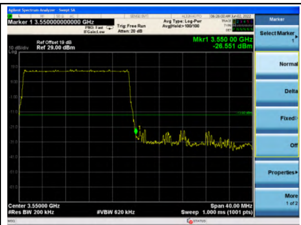
n77_Low Band_20MHz_Upper Band Edge
