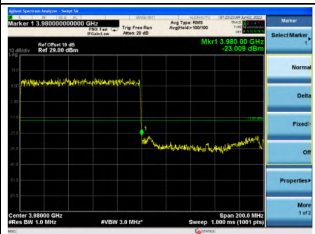
n77_Higher Band_100MHz_Upper Band Edge
