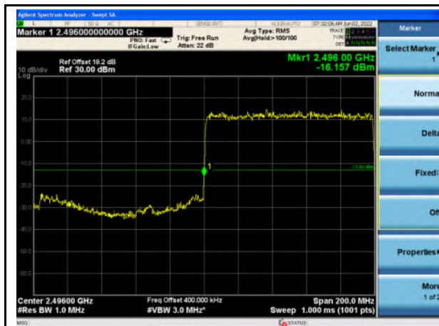
n41_100MHz_Lower Band Edge
