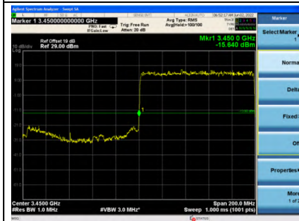
n77_Low Band_100MHz_Lower Band Edge
