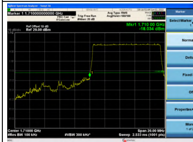
n66_10MHz_Lower Band Edge
