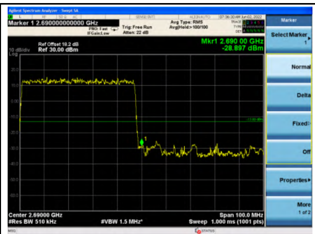
n41_50MHz_Upper Band Edge
