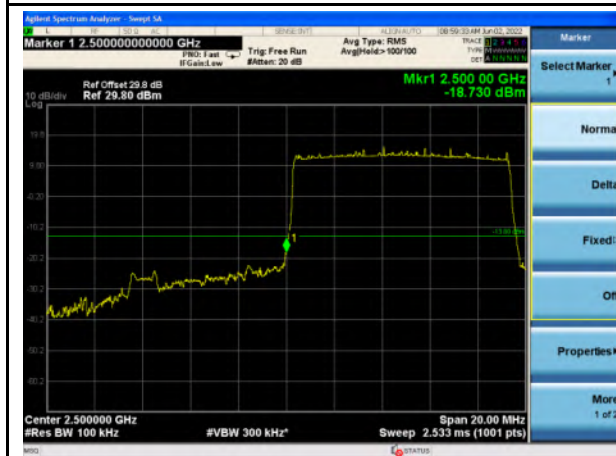
n7_10MHz_Lower Band Edge
