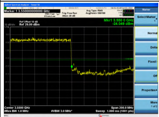
n77_Low Band_100MHz_Upper Band Edge
