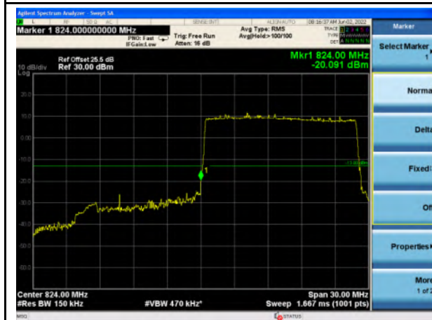
n5_15MHz_Lower Band Edge
