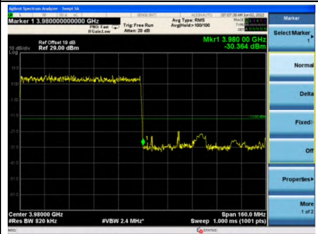
n77_Higher Band_80MHz_Upper Band Edge
