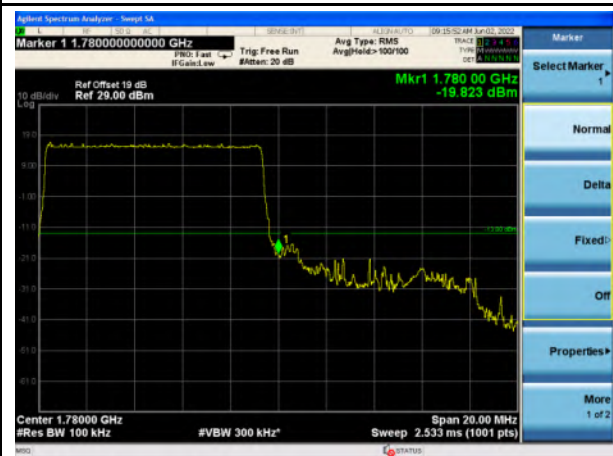
n66_10MHz_Upper Band Edge
