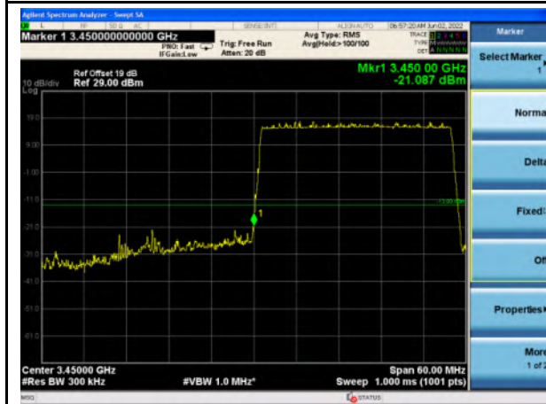
n77_Low Band_30MHz_Lower Band Edge
