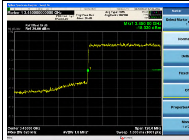
n77_Low Band_80MHz_Lower Band Edge
