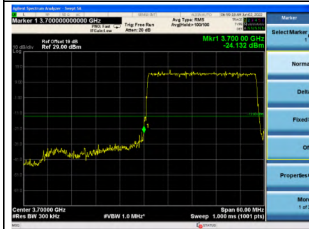
n77_Higher Band_30MHz_Lower Band Edge
