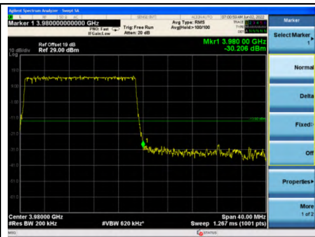
n77_Higher Band_20MHz_Upper Band Edge
