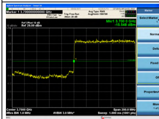
n77_Higher Band_100MHz_Lower Band Edge
