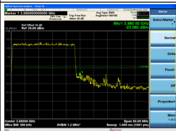
n77_Higher Band_40MHz_Upper Band Edge
