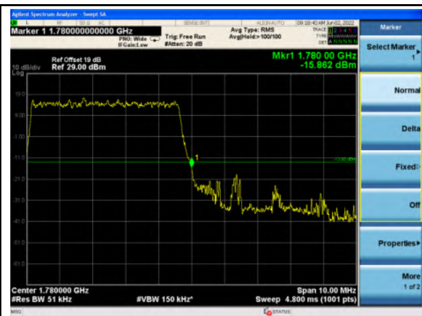
n66_5MHz_Upper Band Edge
