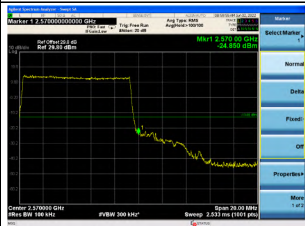
n7_10MHz_Upper Band Edge
