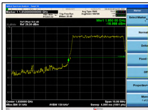
n2_5MHz_Lower Band Edge
