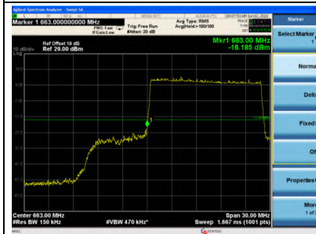
n71_15MHz_Lower Band Edge
