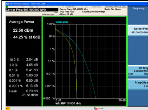
Band 71_QPSK_10M_High_Full RB Config
