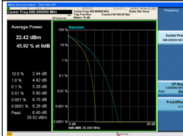
Band 71_QPSK_20M_High_Full RB Config
