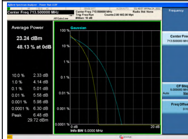
Band 12_QPSK_5M_High_Full RB Config
