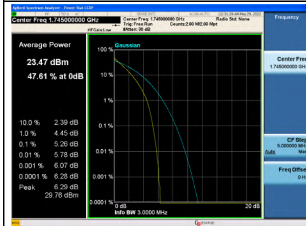
Band 66_QPSK_3M_Mid_Full RB Config
