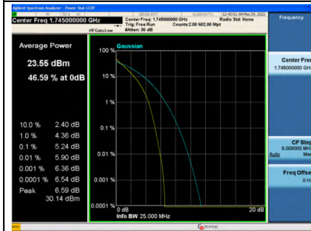
Band 66_QPSK_20M_Mid_Full RB Config
