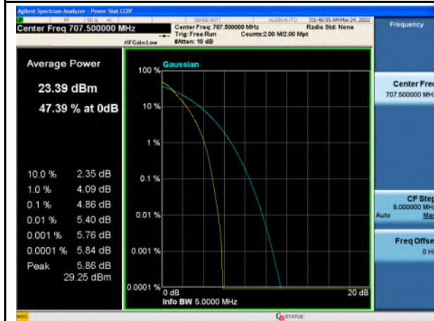
Band 12_QPSK_5M_Mid_Full RB Config
