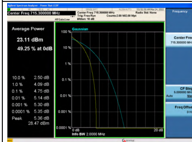
Band 12_QPSK_1.4M_High_Full RB Config
