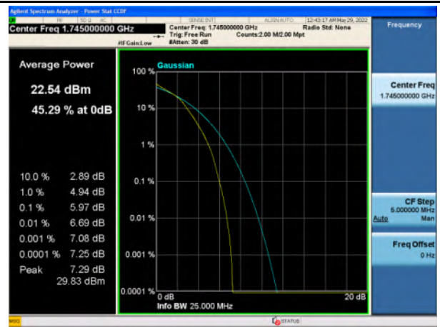
Band 66_16-QAM_20M_Mid_Full RB Config
