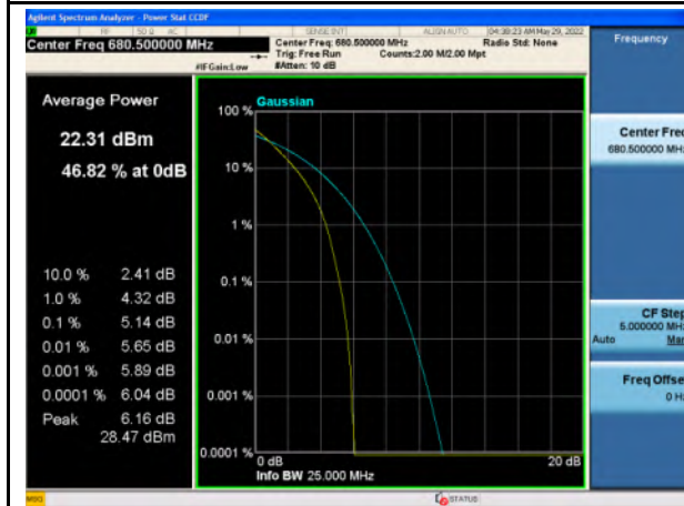
Band 71_QPSK_15M_Mid_Full RB Config
