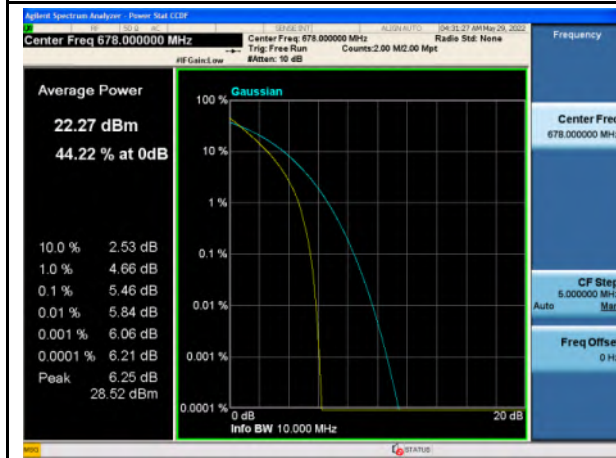
Band 71_QPSK_10M_Mid_Full RB Config
