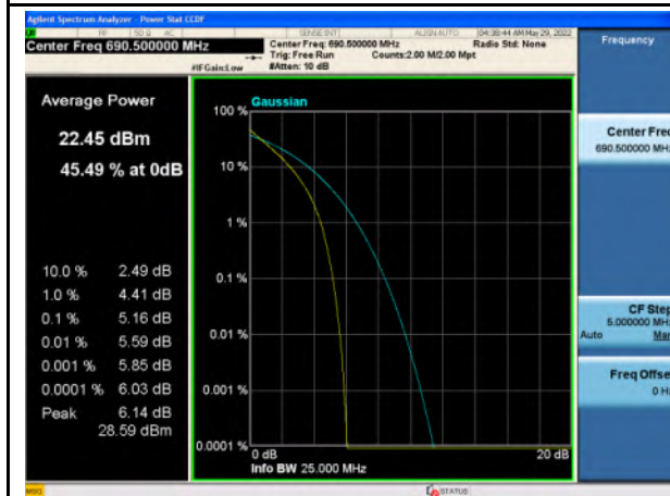
Band 71_QPSK_15M_High_Full RB Config
