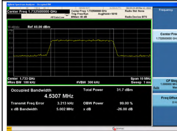
Band 4_QPSK_5M_Mid_Full RB Config
