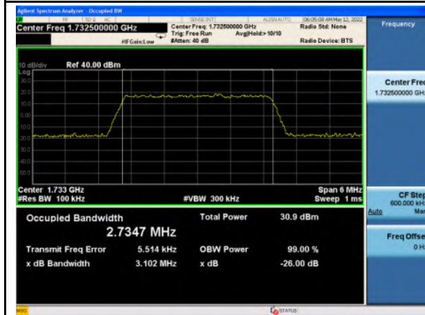
Band 4_QPSK_3M_Mid_Full RB Config
