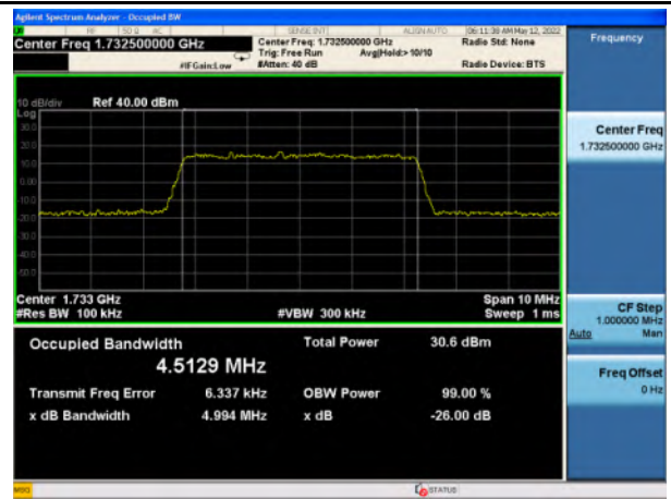
Band 4_16-QAM_5M_Mid_Full RB Config
