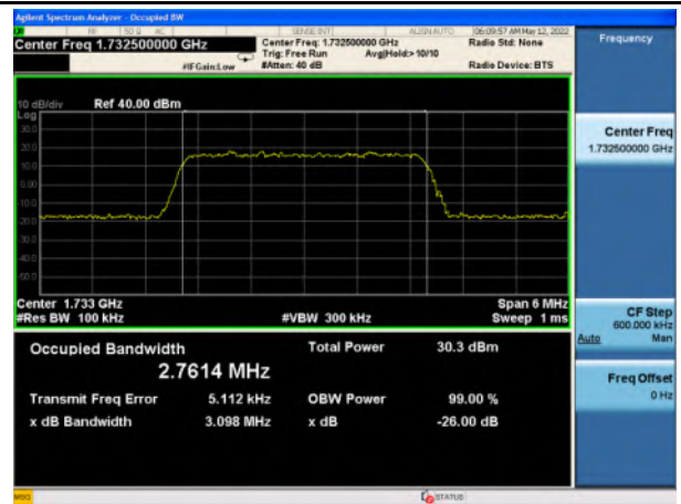
Band 4_16-QAM_3M_Mid_Full RB Config
