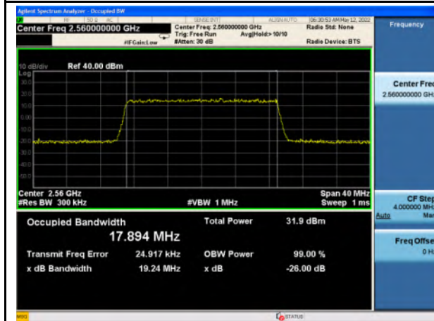
Band 7_QPSK_20M_High_Full RB Config
