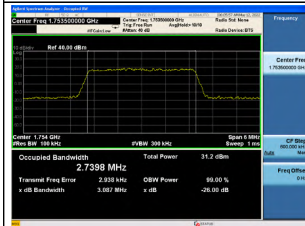
Band 4_QPSK_3M_High_Full RB Config
