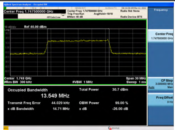
Band 4_16-QAM_15M_High_Full RB Config
