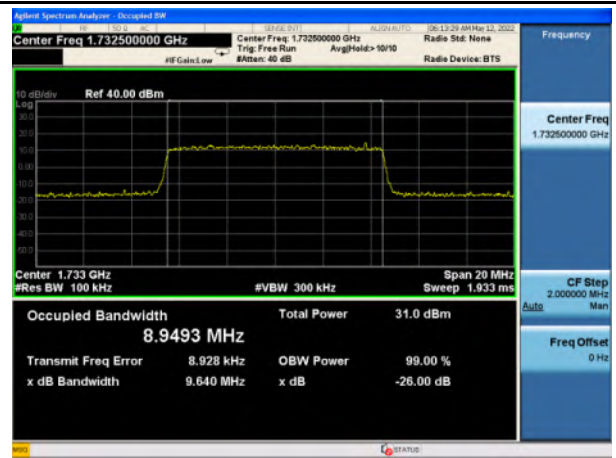
Band 4_16-QAM_10M_Mid_Full RB Config
