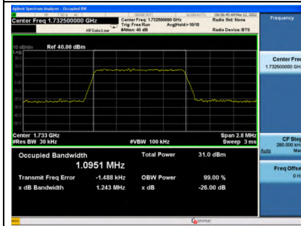
Band 4_QPSK_1.4M_Mid_Full RB Config
