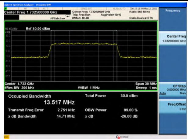
Band 4_16-QAM_15M_Mid_Full RB Config
