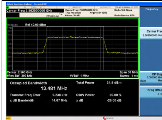
Band 7_QPSK_15M_High_Full RB Config
