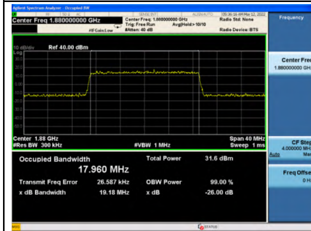
Band 2_QPSK_20M_Mid_Full RB Config
