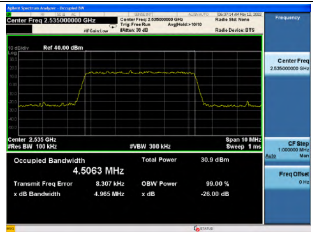
Band 7_16-QAM_5M_Mid_Full RB Config
