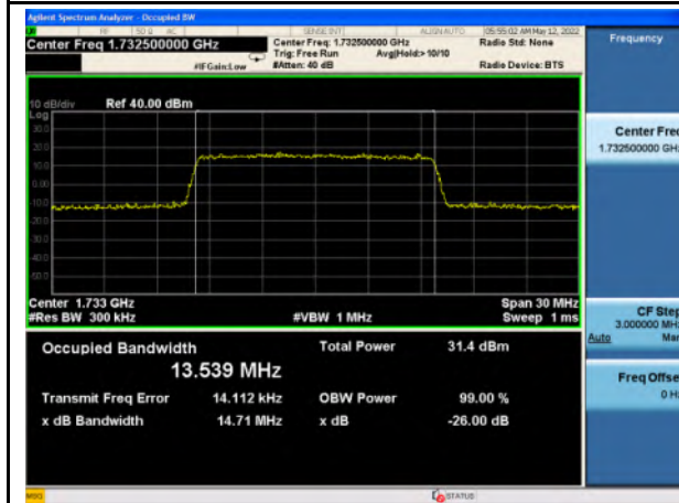
Band 4_QPSK_15M_Mid_Full RB Config
