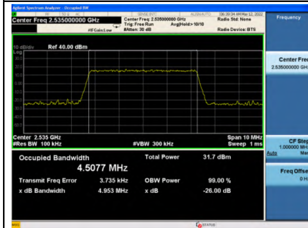
Band 7_QPSK_5M_Mid_Full RB Config
