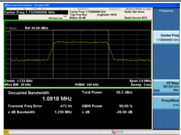
Band 4_16-QAM_1.4M_Mid_Full RB Config
