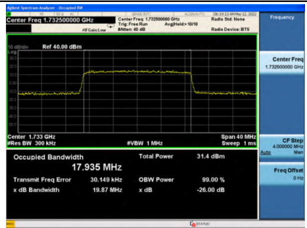
Band 4_16-QAM_20M_Mid_Full RB Config
