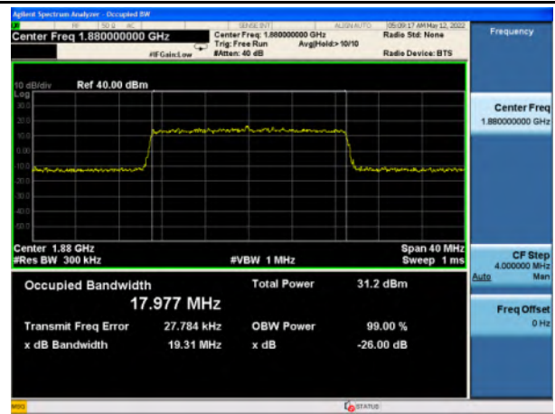
Band 2_16-QAM_20M_Mid_Full RB Config
