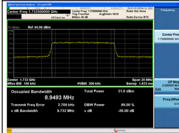
Band 4_QPSK_10M_Mid_Full RB Config
