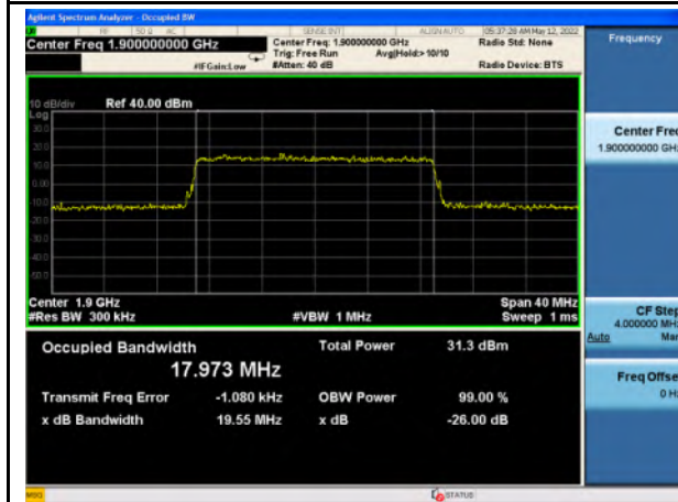
Band 2_QPSK_20M_High_Full RB Config
