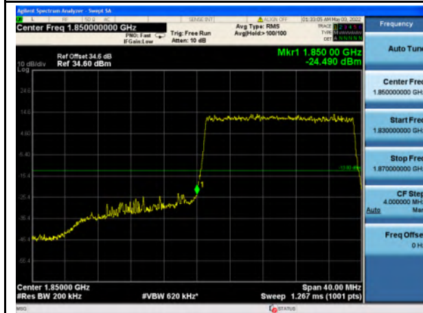
Band 2_QPSK_20M_Low_Full RB Config
