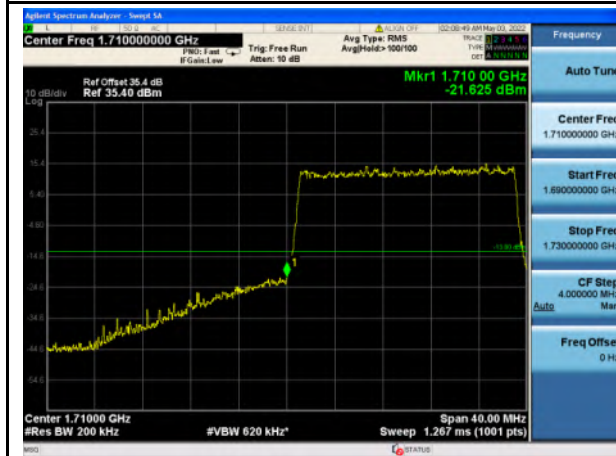
Band 4_QPSK_20M_Low_Full RB Config
