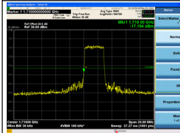
Band 66_QPSK_3M_Low_Full RB Config
