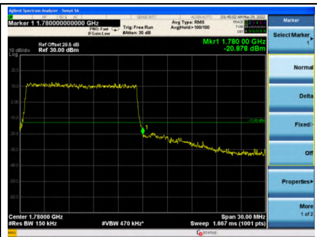
Band 66_16-QAM_15M_High_Full RB Config
