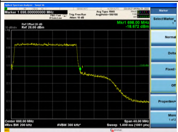
Band 71_16-QAM_20M_High_Full RB Config
