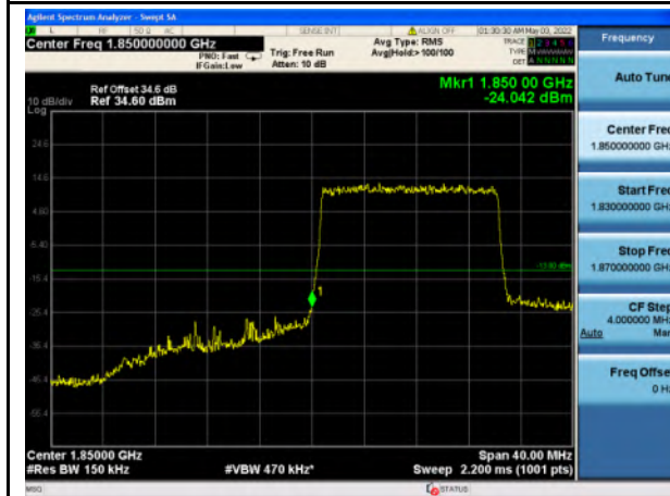
Band 2_QPSK_15M_Low_Full RB Config
