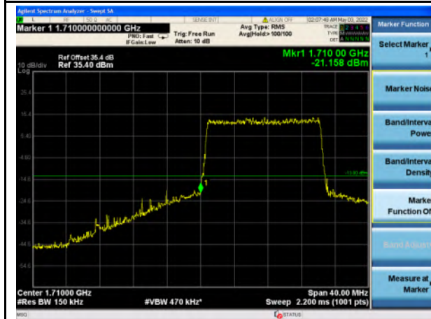
Band 4_QPSK_15M_Low_Full RB Config
