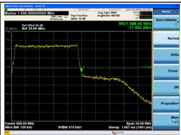
Band 71_16-QAM_15M_High_Full RB Config
