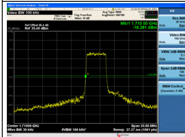
Band 4_QPSK_3M_Low_Full RB Config
