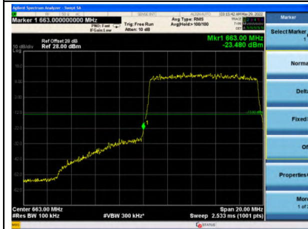
Band 71_16-QAM_10M_Low_Full RB Config
