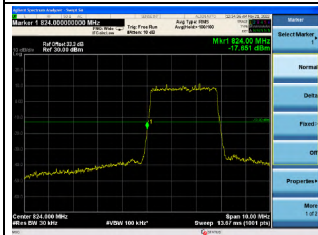
Band 5_QPSK_3M_Low_Full RB Config
