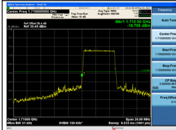
Band 4_16-QAM_5M_Low_Full RB Config
