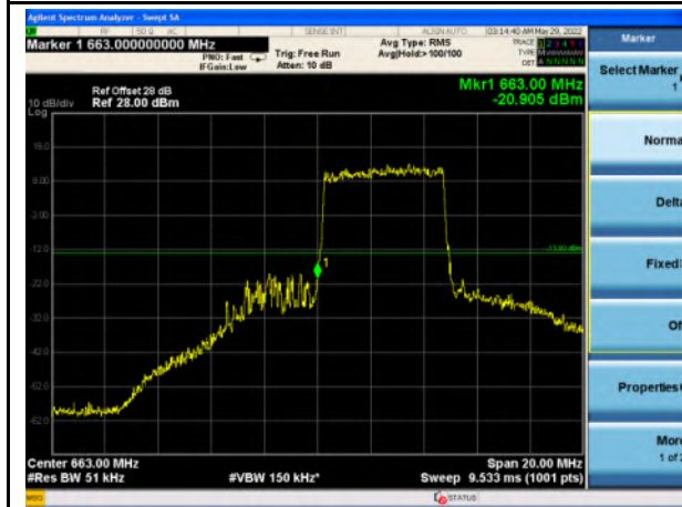
Band 71_16-QAM_5M_Low_Full RB Config
