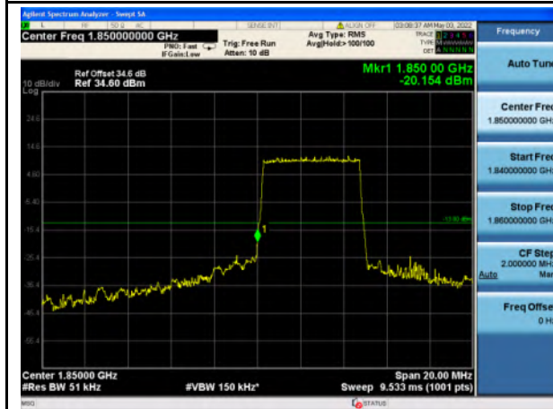
Band 2_16-QAM_5M_Low_Full RB Config
