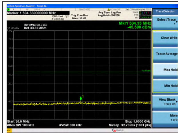
Band 38_QPSK_20M_Mid - 30MHz~1GHz
