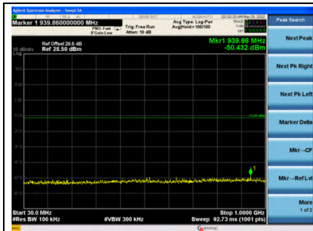
Band 66_QPSK_1.4M_Mid - 30MHz~1GHz
