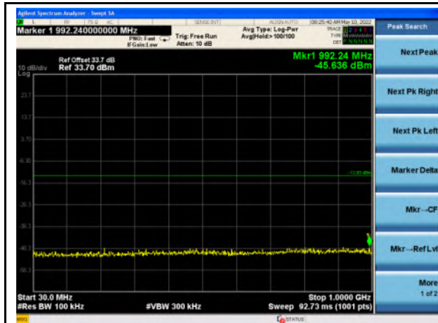
Band 7_QPSK_5M_Mid - 30MHz~1GHz
