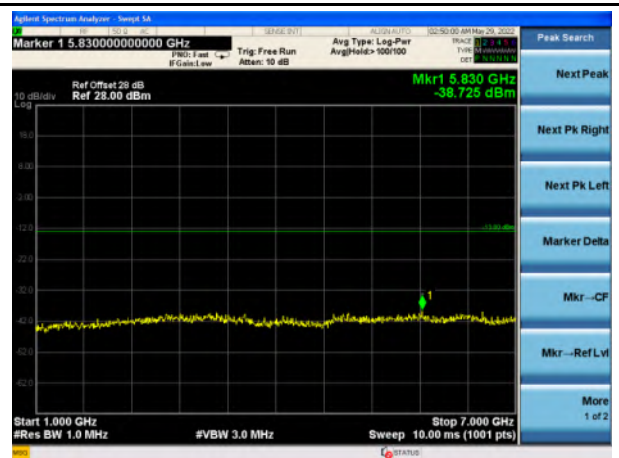
Band 71_QPSK_5M - Mid- 1GHz~7GHz
