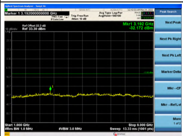
Band 5_QPSK_5M - Mid- 1GHz~9GHz
