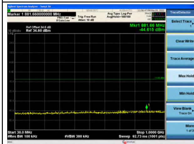
Band 2_QPSK_20M_Mid - 30MHz~1GHz
