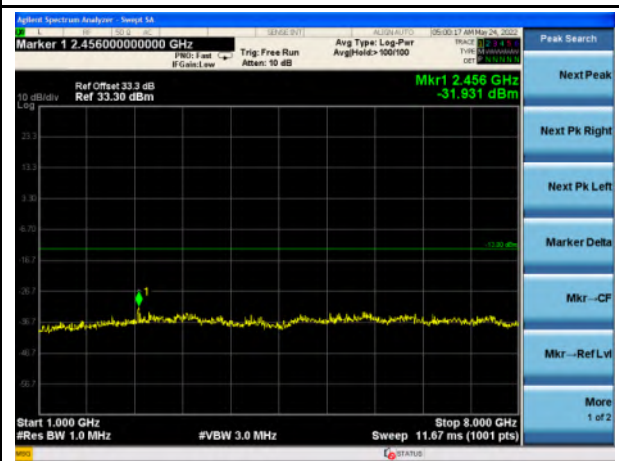
Band 13_QPSK_10M - Mid- 1GHz~8GHz
