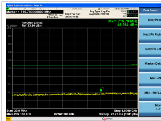
Band 38_QPSK_5M_Mid - 30MHz~1GHz
