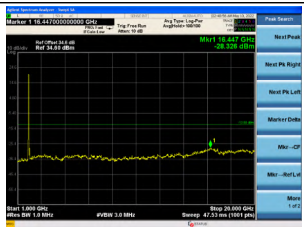
Band 2_QPSK_15M - Mid- 1GHz~20GHz
