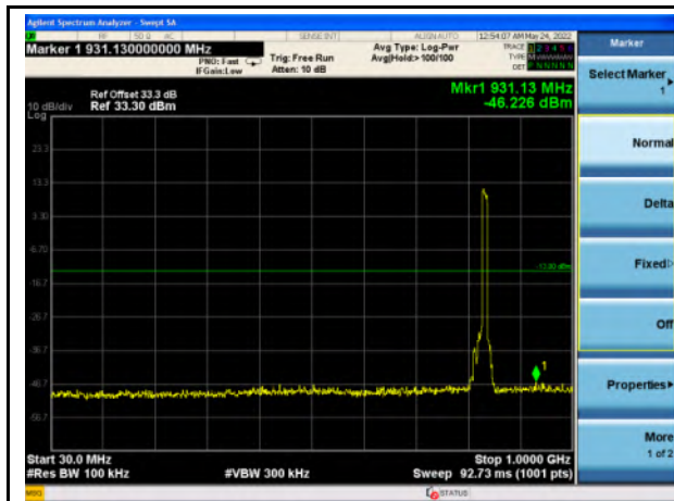
Band 5_QPSK_10M_Mid - 30MHz~1GHz
