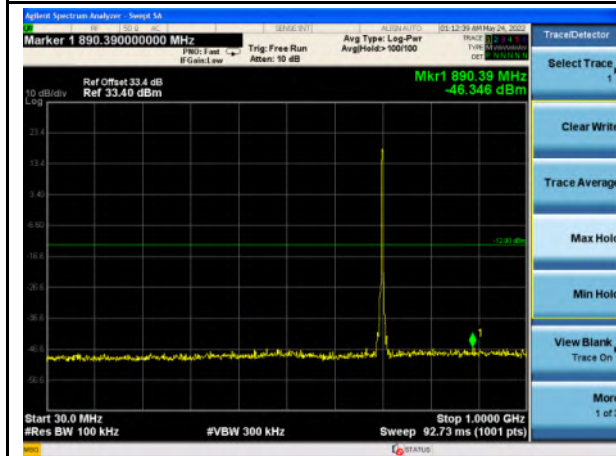
Band 12_QPSK_3M_Mid - 30MHz~1GHz
