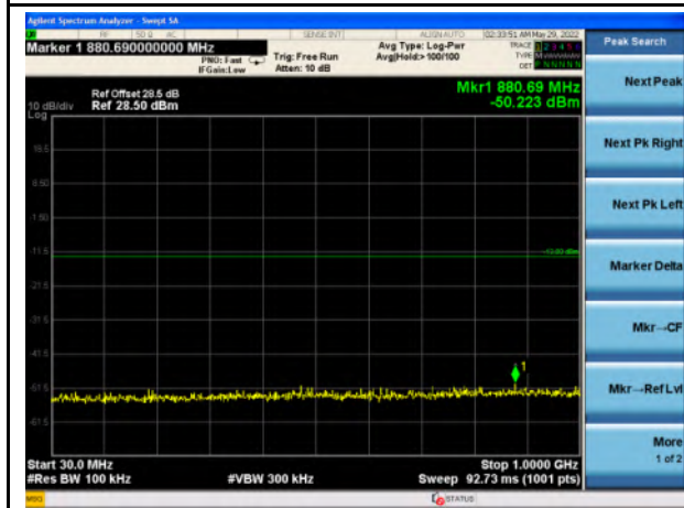
Band 66_QPSK_3M_Mid - 30MHz~1GHz
