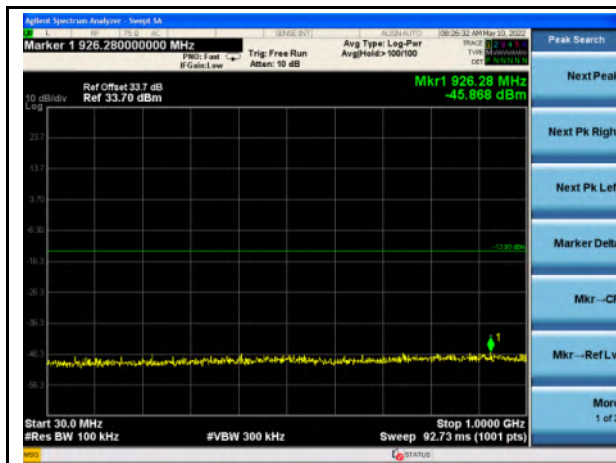
Band 7_QPSK_10M_Mid - 30MHz~1GHz
