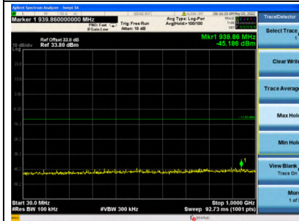
Band 38_QPSK_15M_Mid - 30MHz~1GHz
