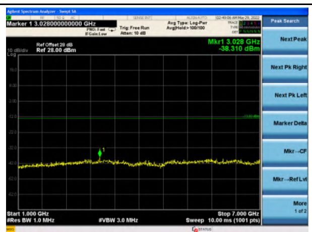
Band 71_QPSK_10M - Mid- 1GHz~7GHz
