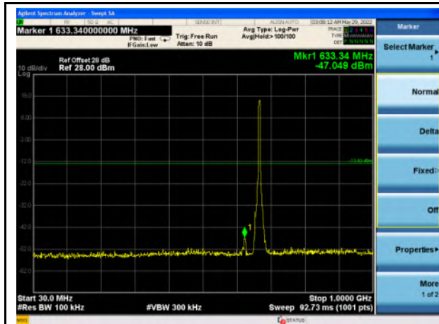
Band 71_QPSK_5M_Mid - 30MHz~1GHz
