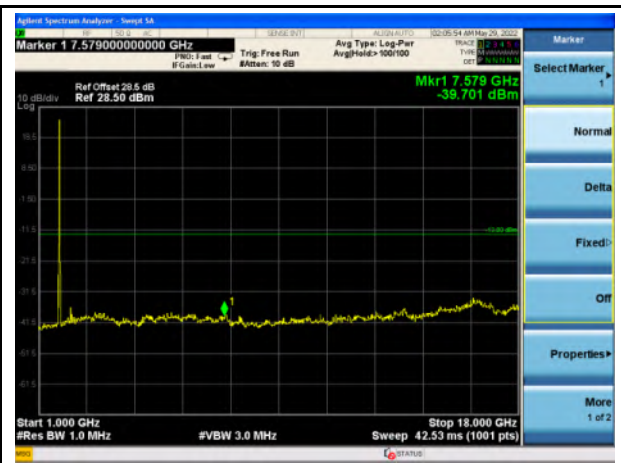
Band 66_QPSK_5M - Mid- 1GHz~18GHz
