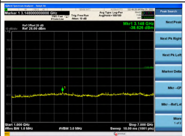
Band 71_QPSK_20M - Mid- 1GHz~7GHz
