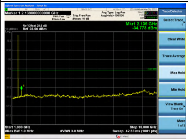
Band 66_QPSK_3M - Mid- 1GHz~18GHz
