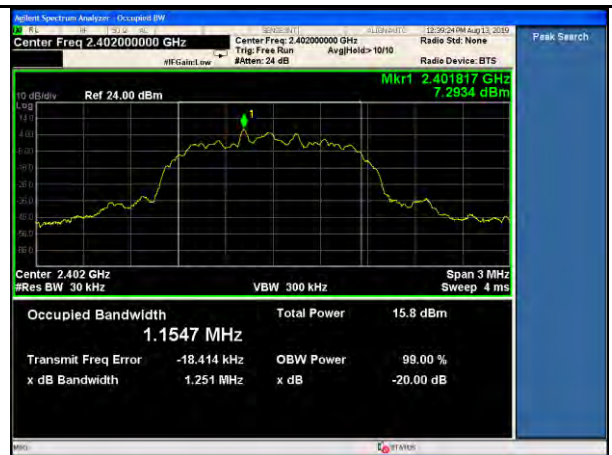
BT- \pi/4 DQPSK-20 dB BW-Low
