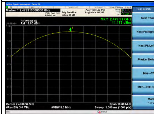
BT-8DPSK-PWR-High
