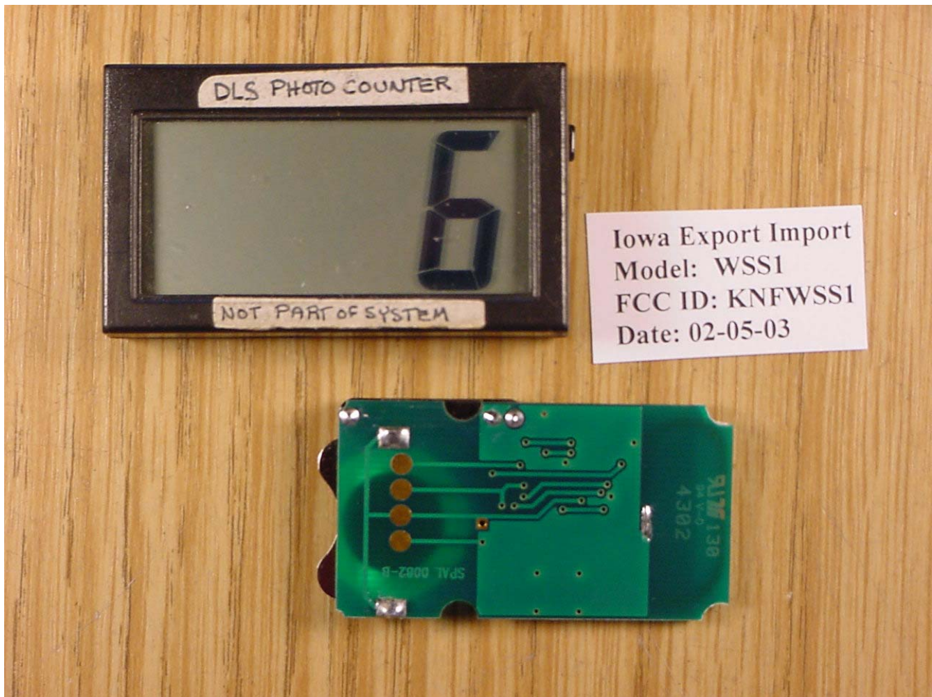
CIRCUIT BOARD - SIDE 2
